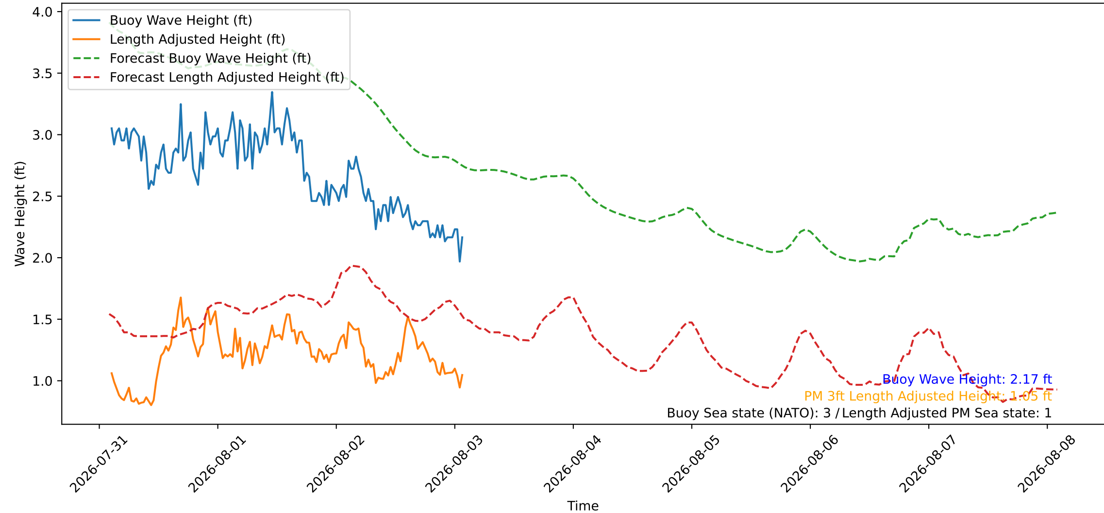
Wave Heights over Time for Red Beach at 2026-08-03 02:10:46
