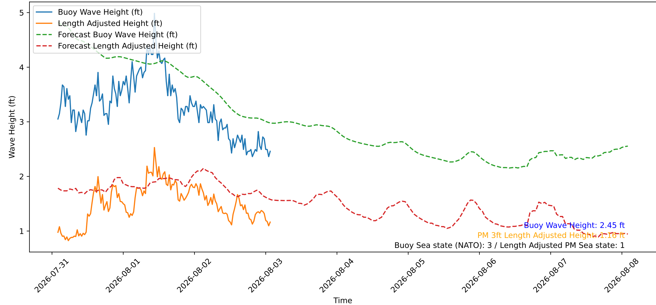
Wave Heights over Time for Green Beach at 2026-08-03 02:11:08
