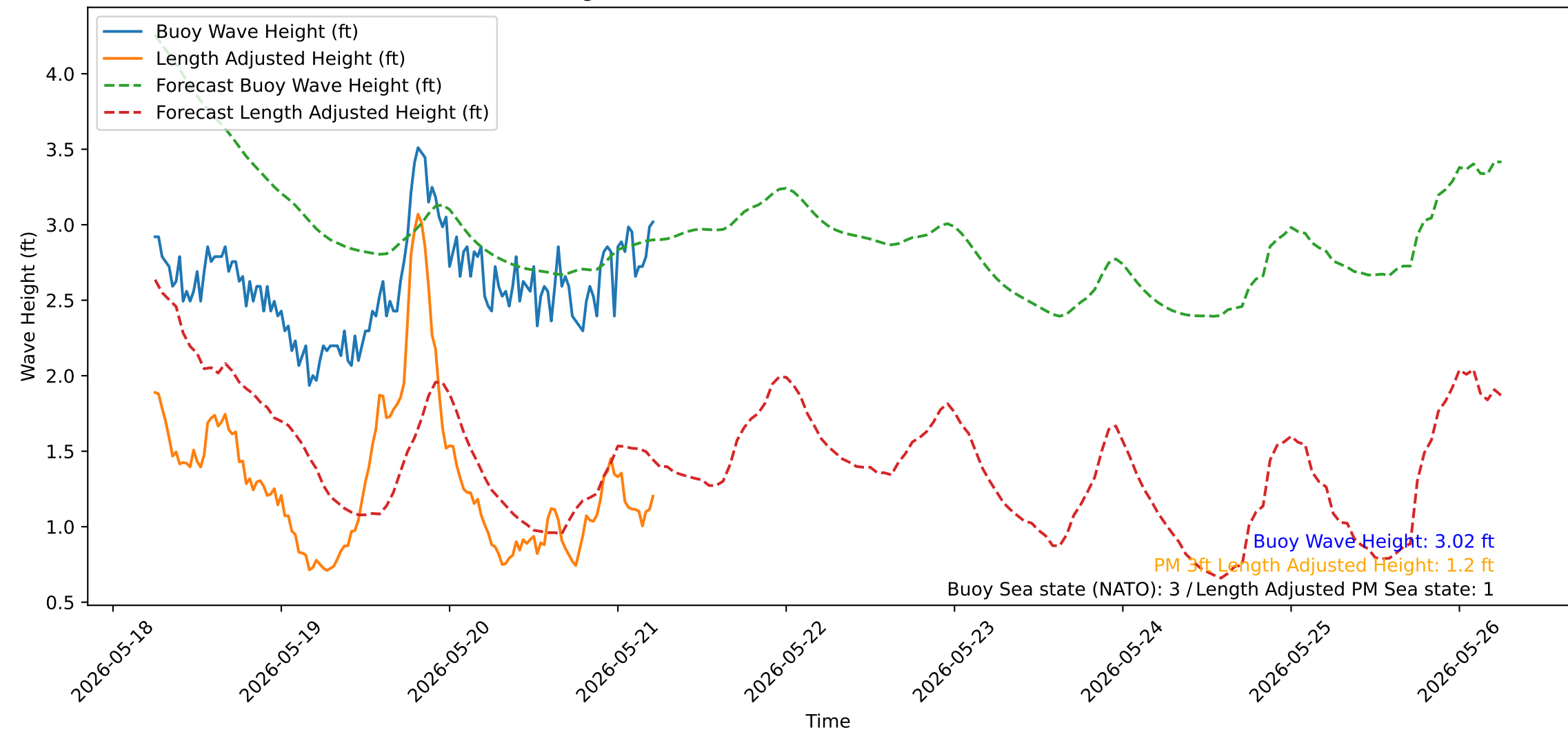
Wave Heights over Time for Red Beach at 2026-05-21 05:50:52
