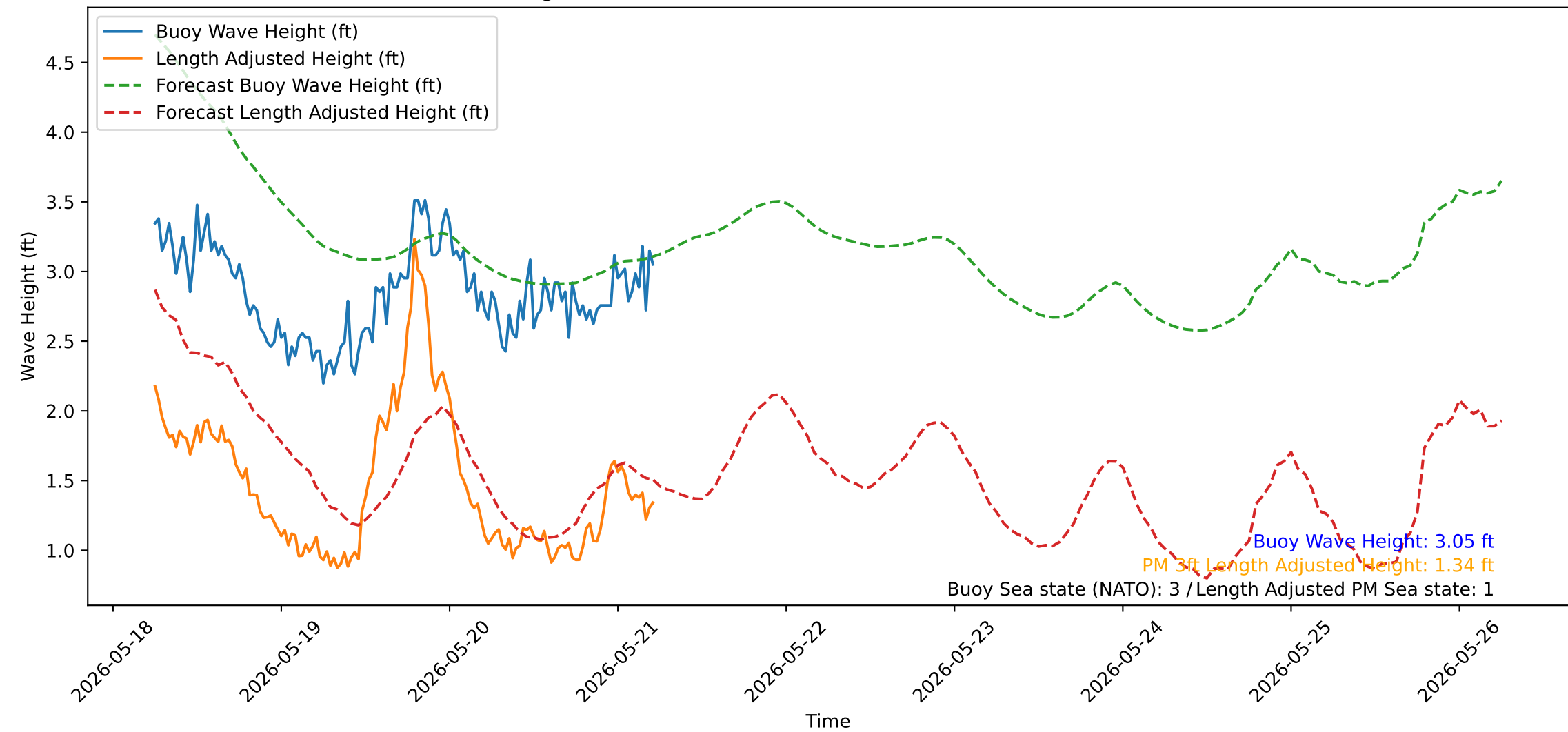
Wave Heights over Time for Oceanside Harbor at 2026-05-21 05:50:32
