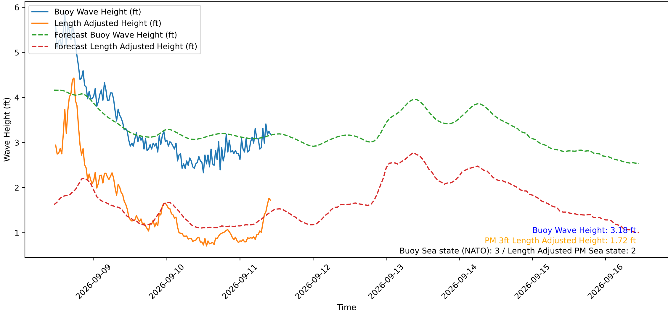
Wave Heights over Time for Red Beach at 2026-09-11 11:00:50
