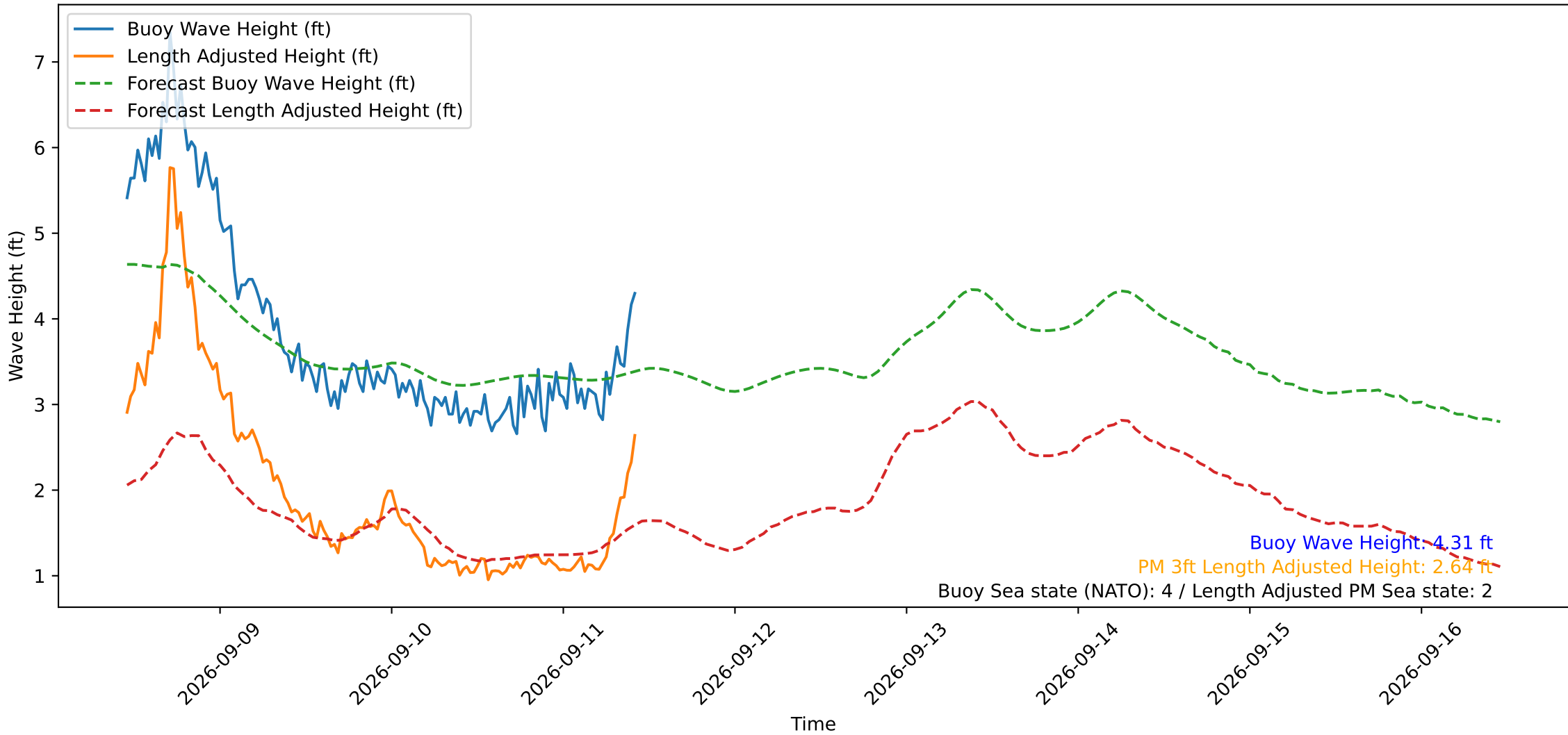
Wave Heights over Time for Oceanside Harbor at 2026-09-11 11:00:30
