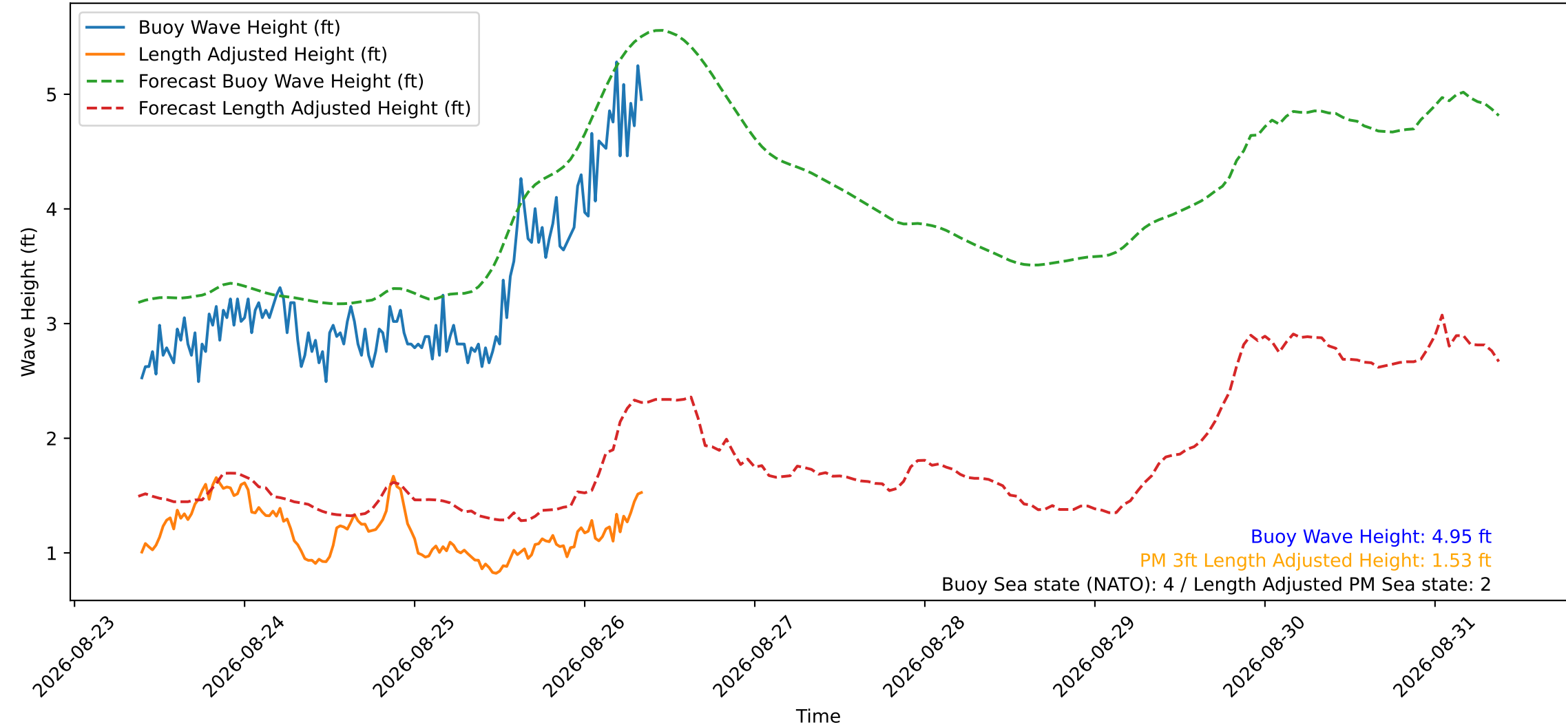
Wave Heights over Time for Green Beach at 2026-08-26 09:01:16
