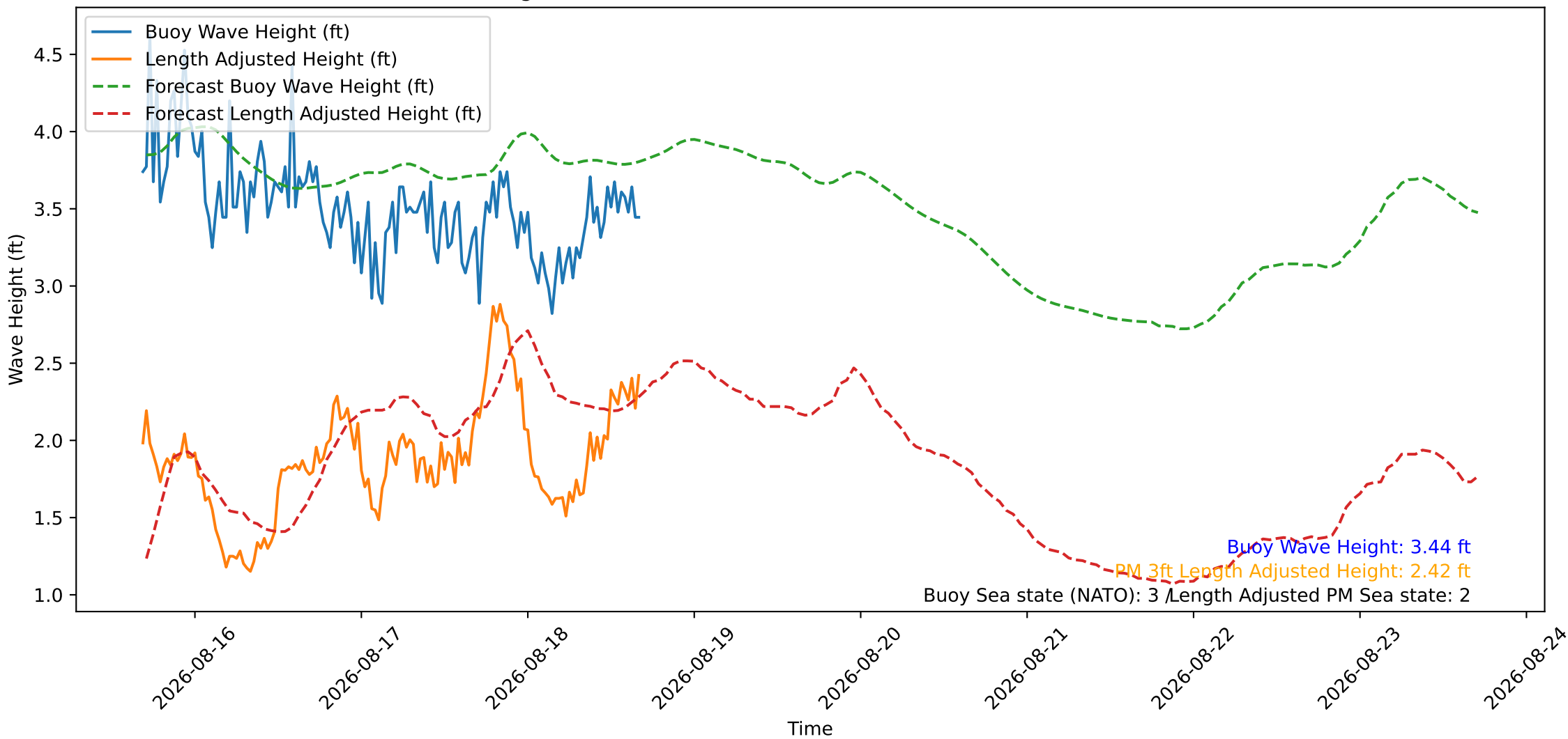
Wave Heights over Time for Oceanside Harbor at 2026-08-18 16:40:26
