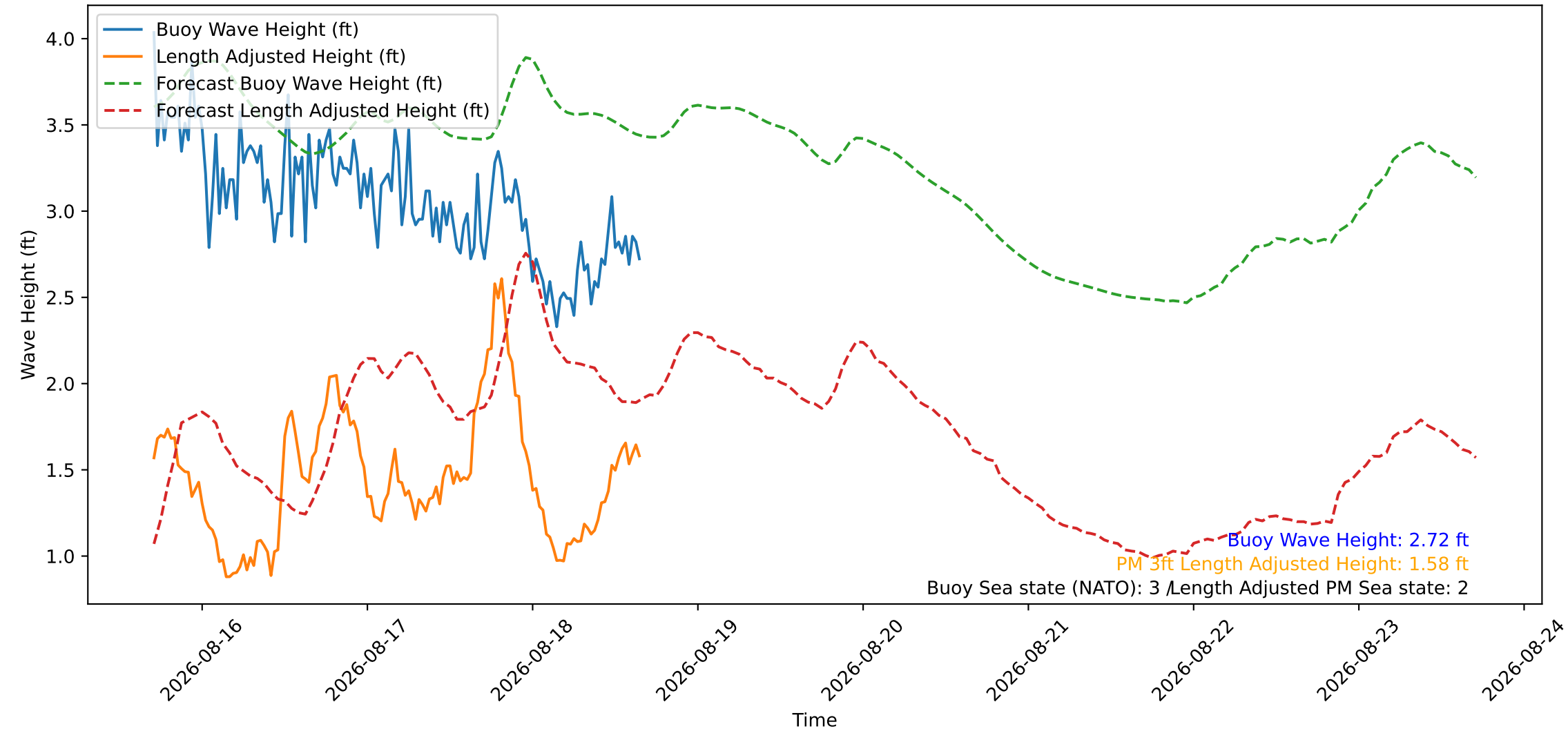
Wave Heights over Time for Red Beach at 2026-08-18 16:40:46
