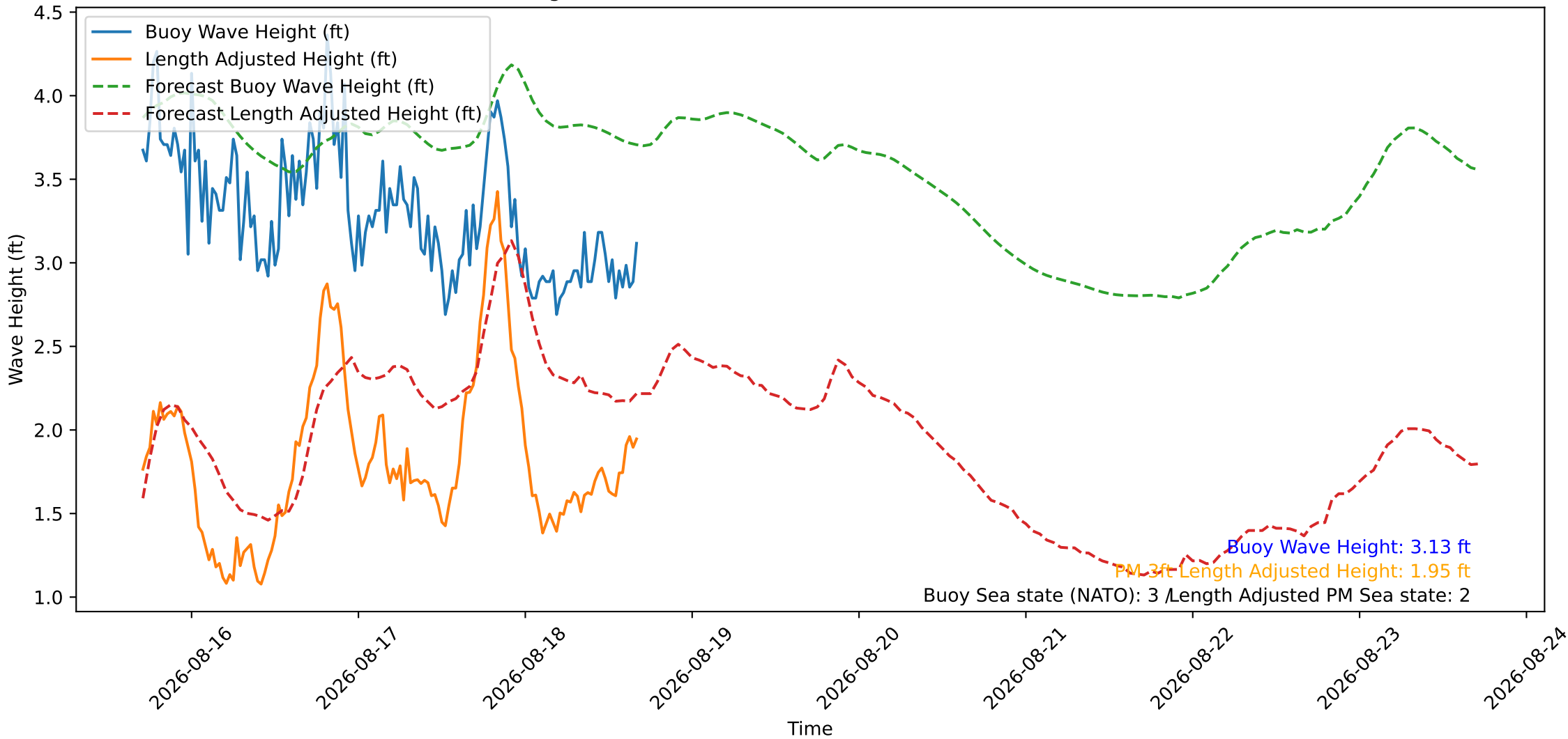
Wave Heights over Time for Green Beach at 2026-08-18 16:41:08
