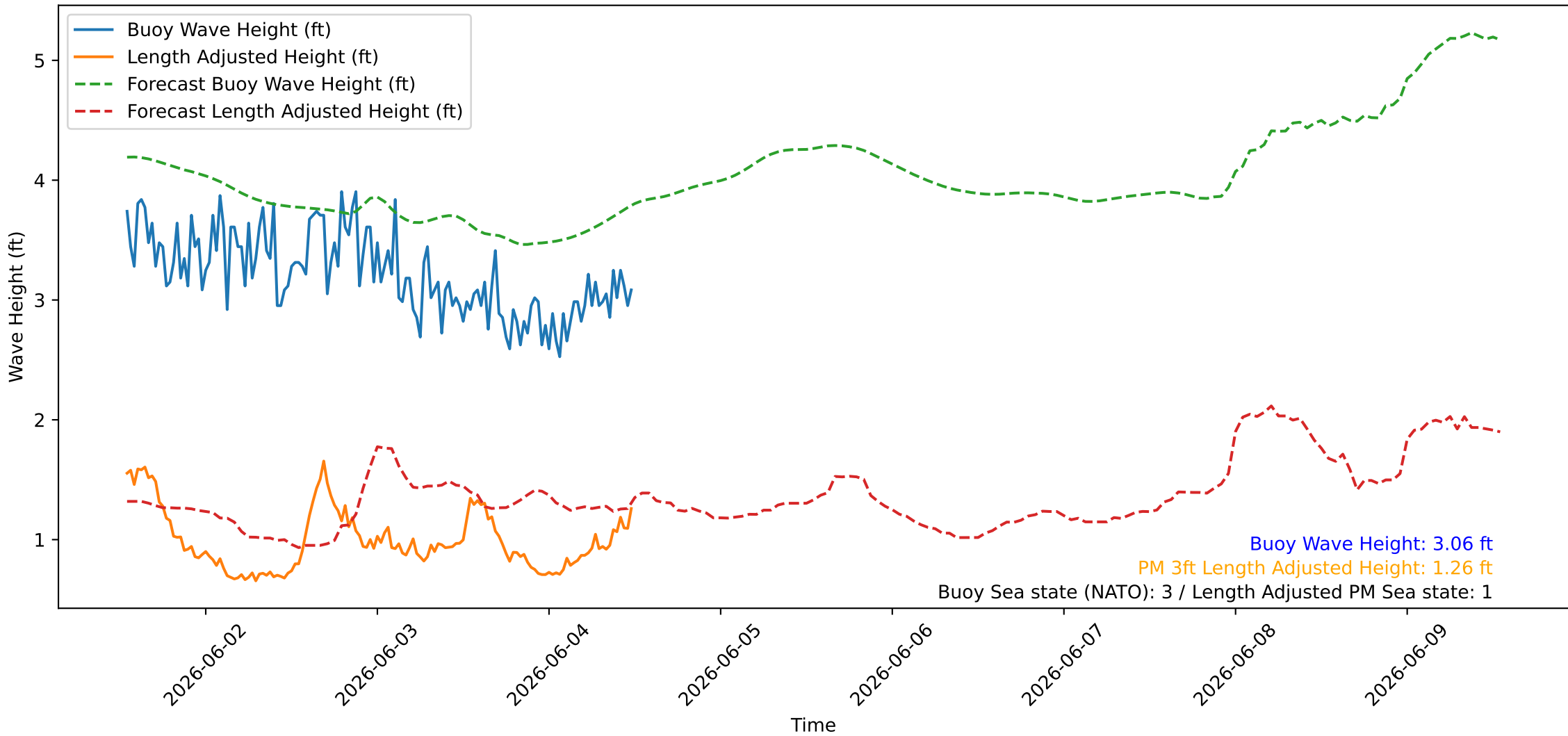
Wave Heights over Time for Red Beach at 2026-06-04 12:30:45
