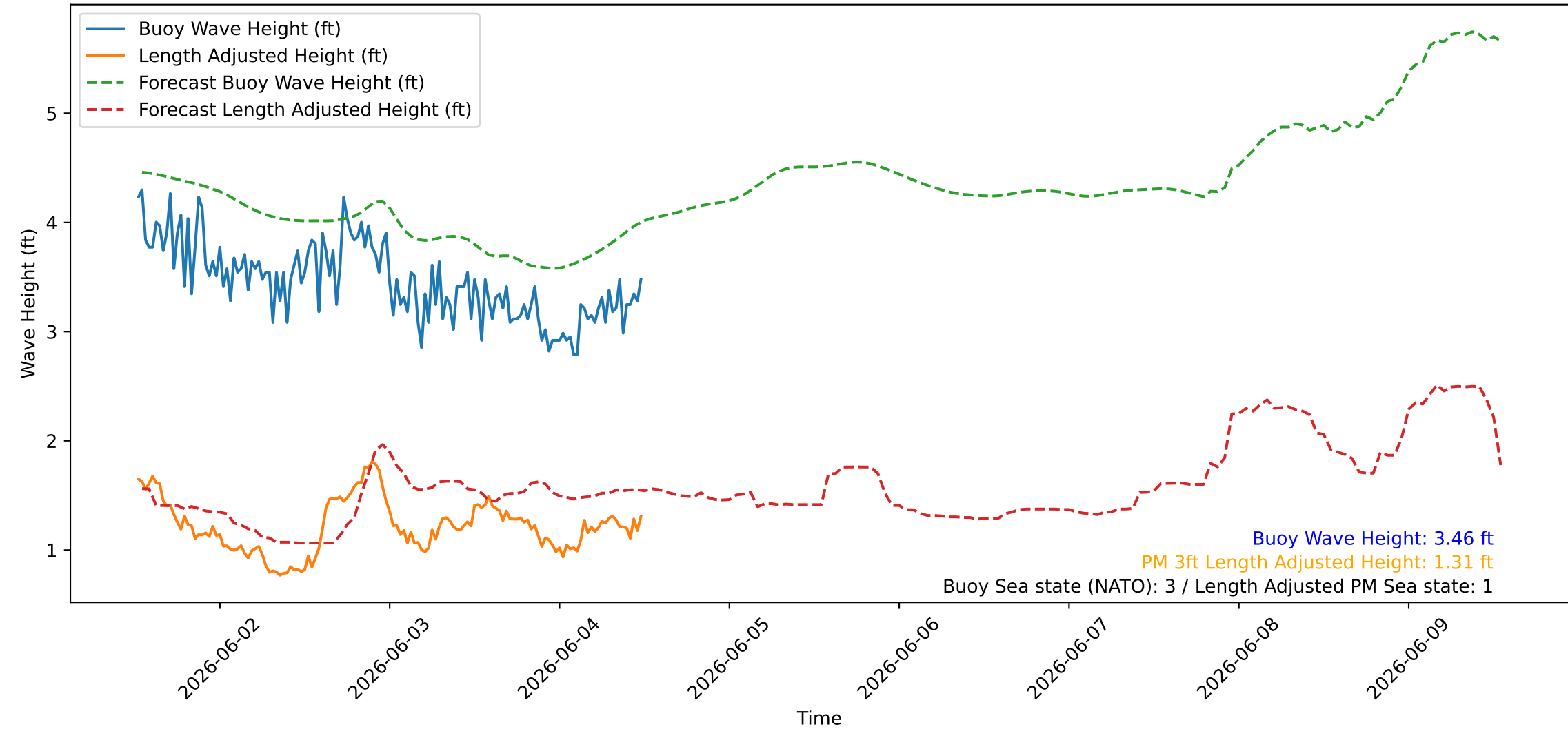
Wave Heights over Time for Green Beach at 2026-06-04 12:31:08
