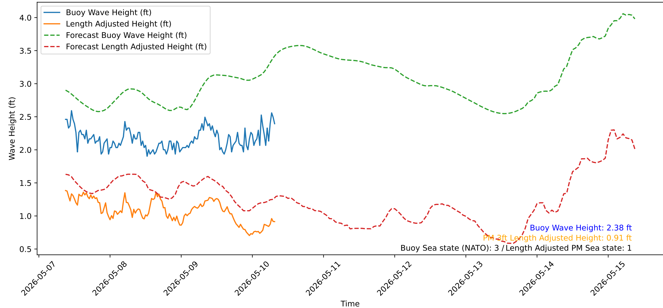
Wave Heights over Time for Red Beach at 2026-05-10 08:30:53
