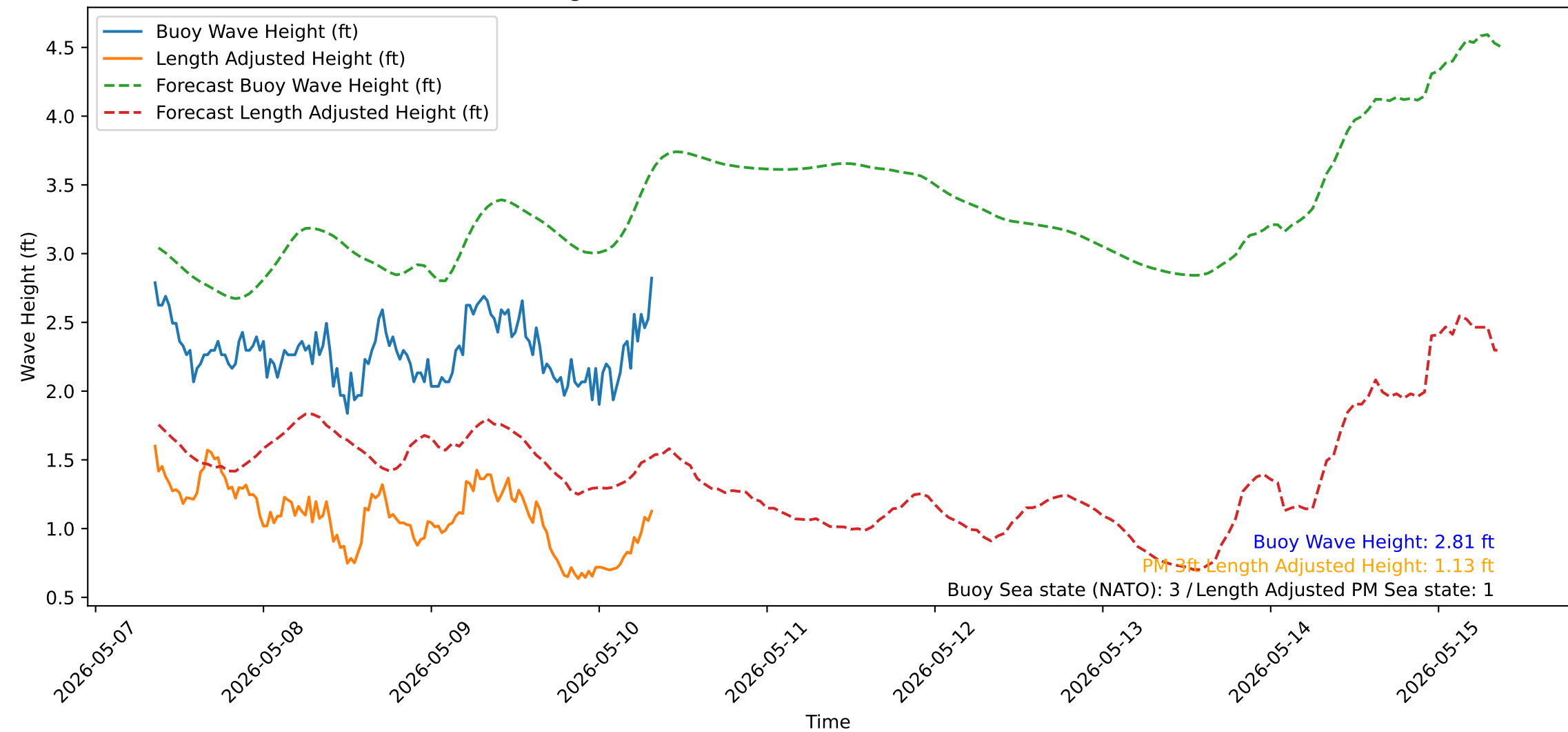
Wave Heights over Time for Green Beach at 2026-05-10 08:31:18
