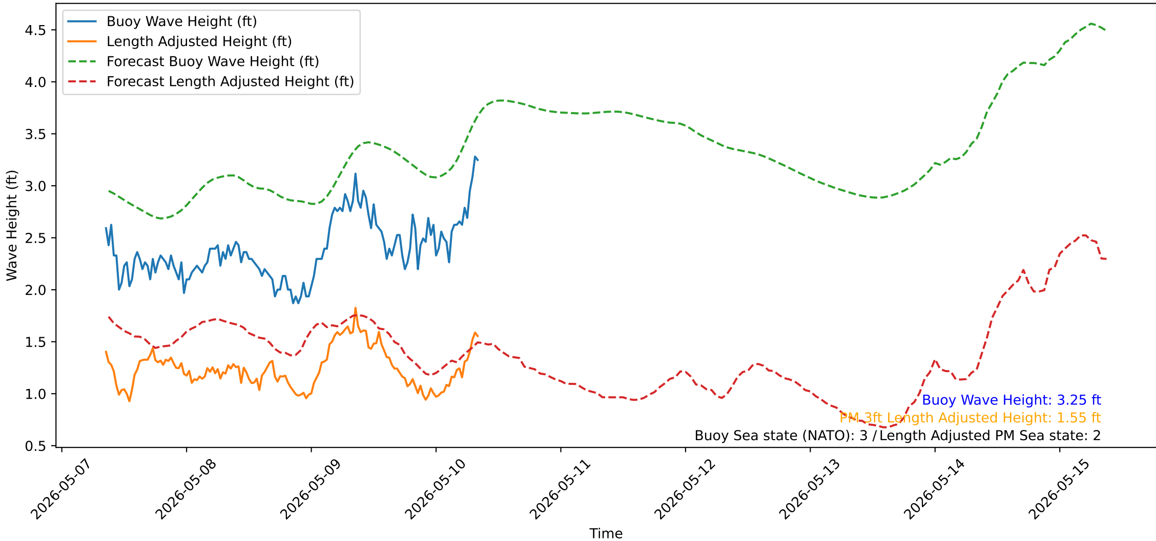
Wave Heights over Time for Oceanside Harbor at 2026-05-10 08:30:33
