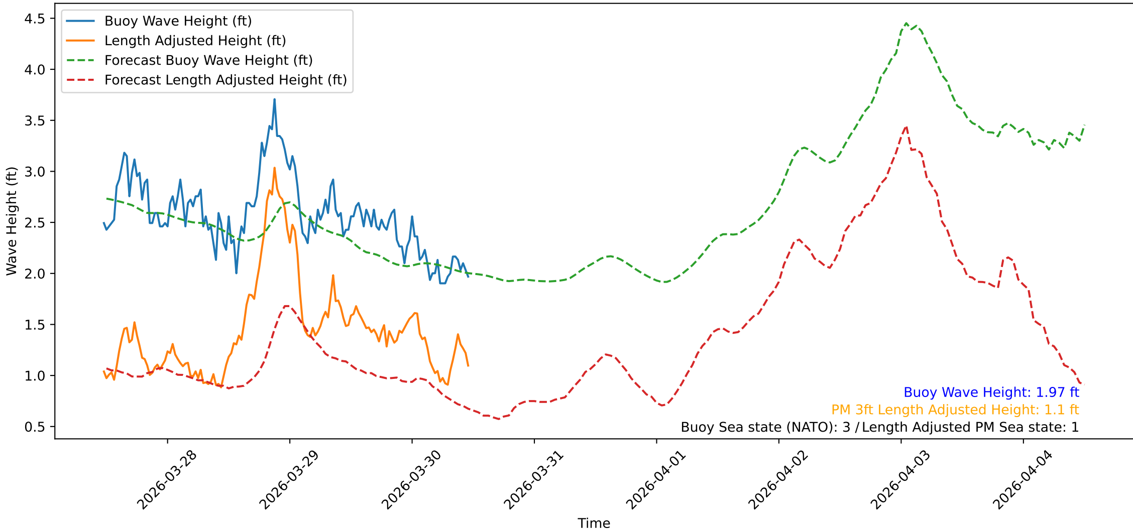
Wave Heights over Time for Green Beach at 2026-03-30 11:41:09
