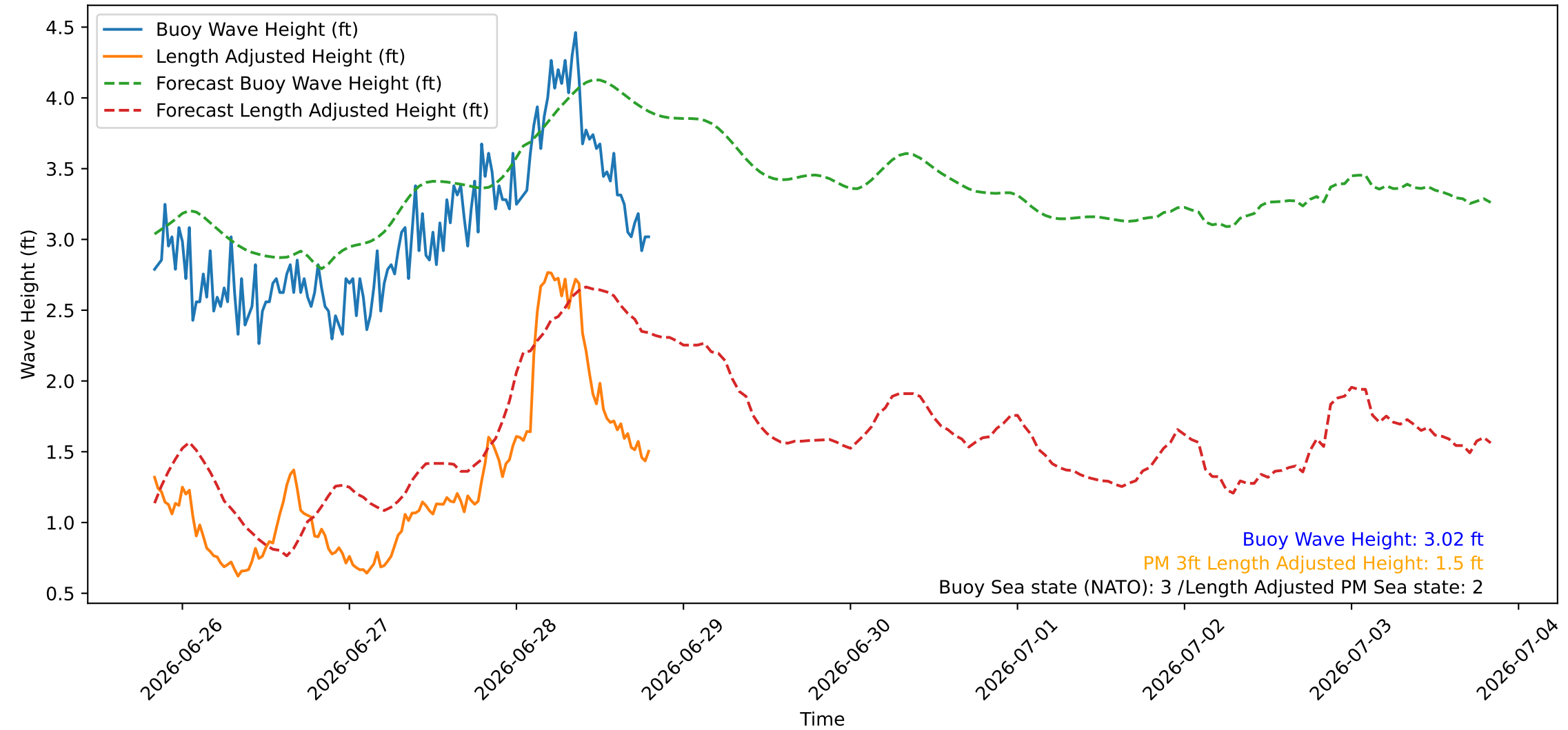
Wave Heights over Time for Red Beach at 2026-06-28 19:40:45
