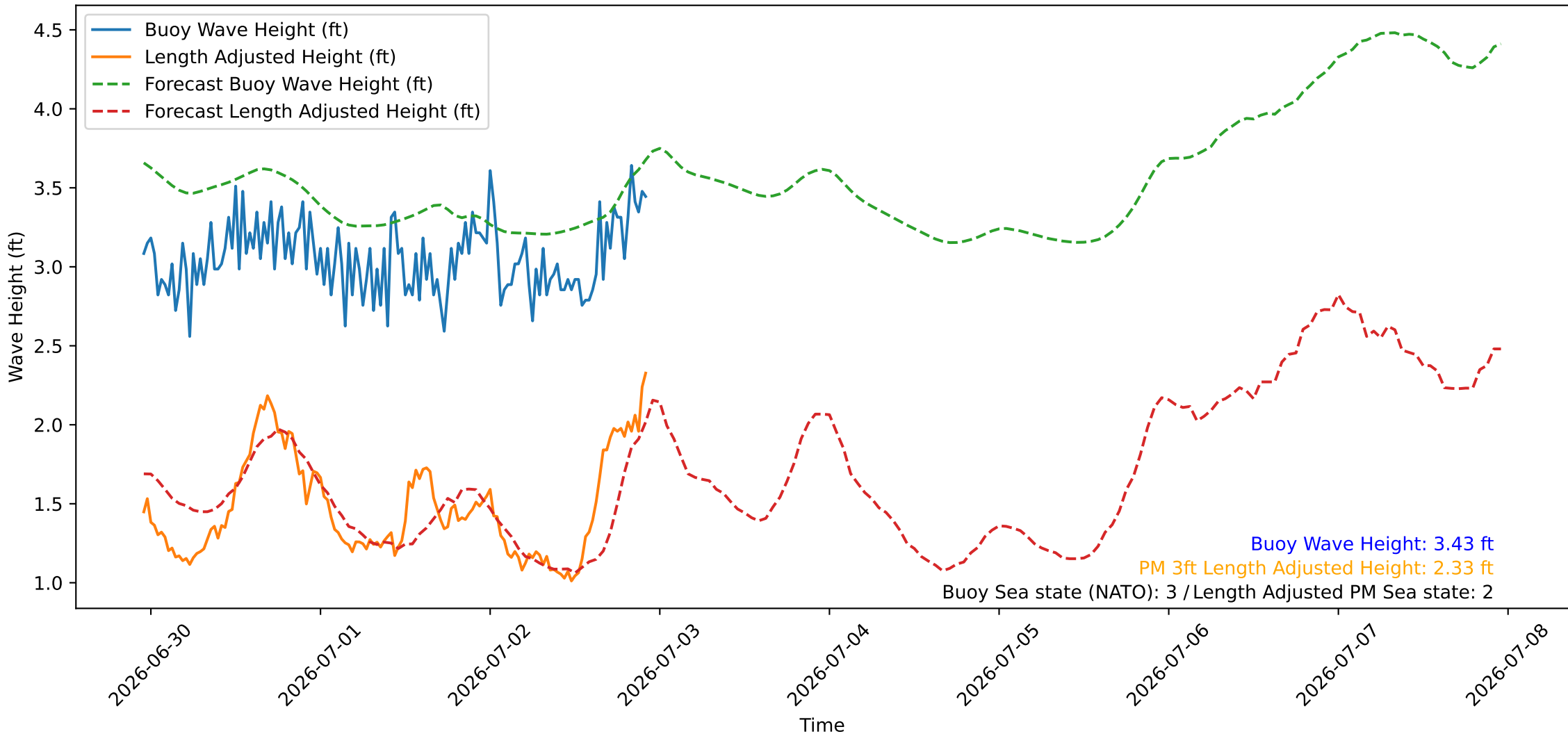
Wave Heights over Time for Oceanside Harbor at 2026-07-02 22:50:26
