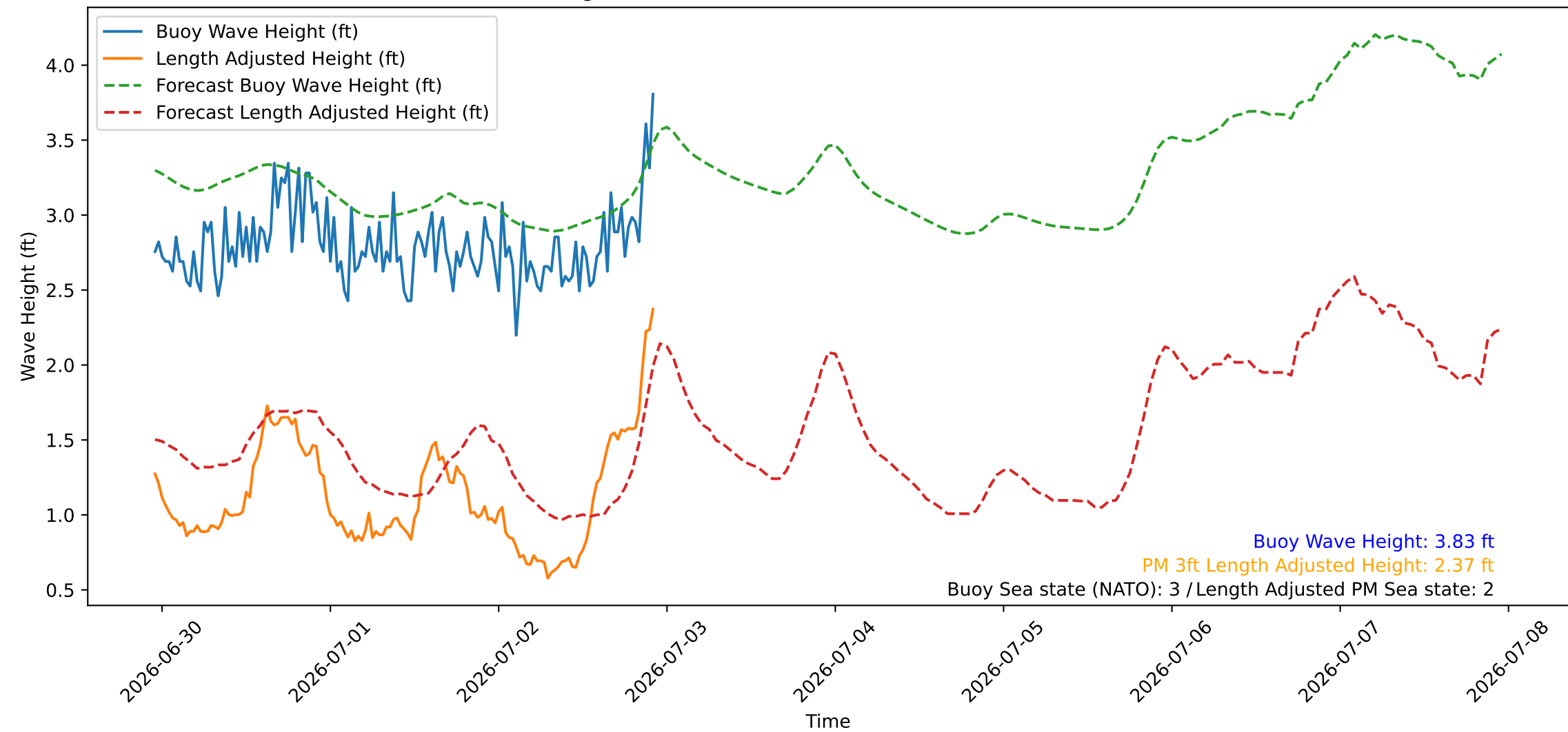
Wave Heights over Time for Red Beach at 2026-07-02 22:50:48
