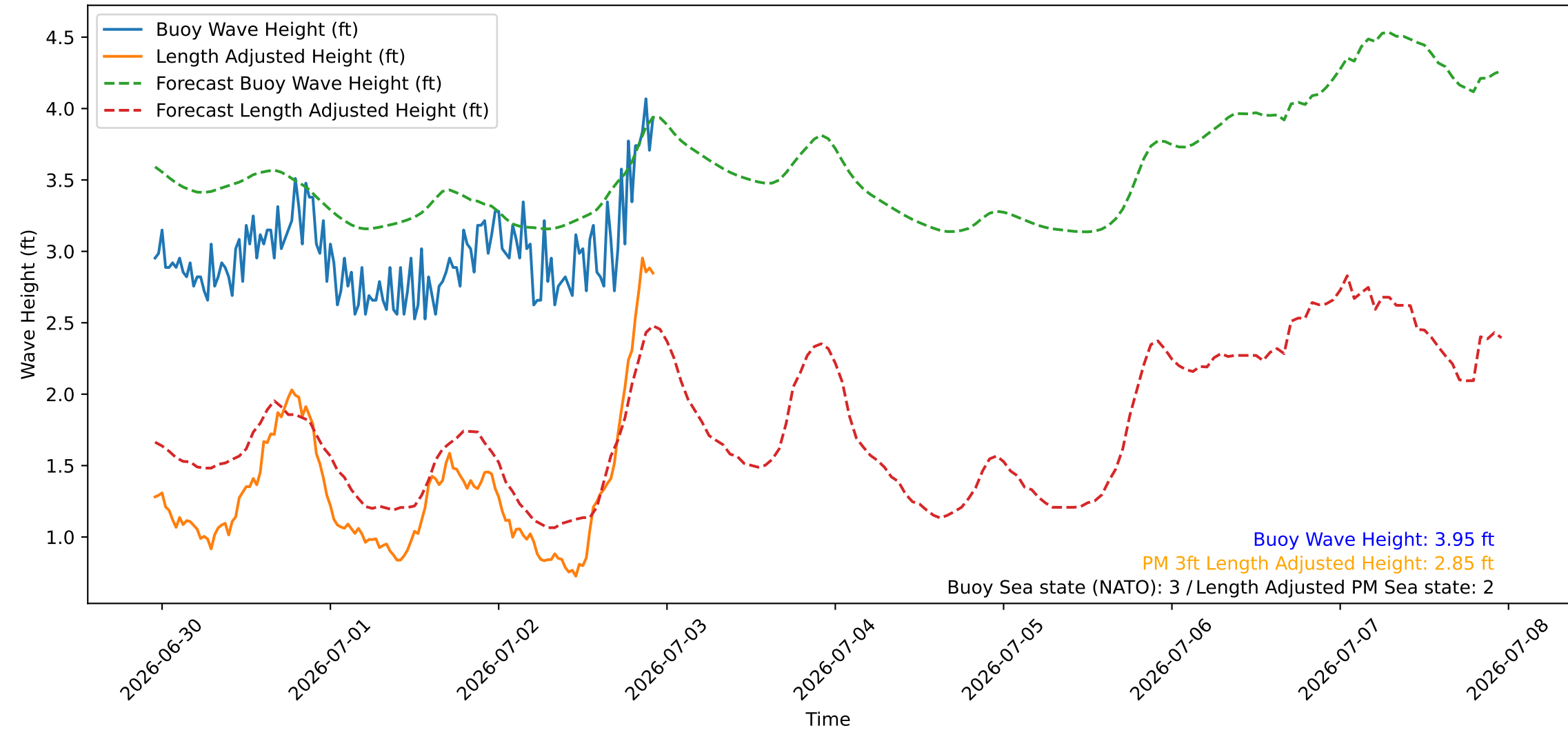
Wave Heights over Time for Green Beach at 2026-07-02 22:51:10
