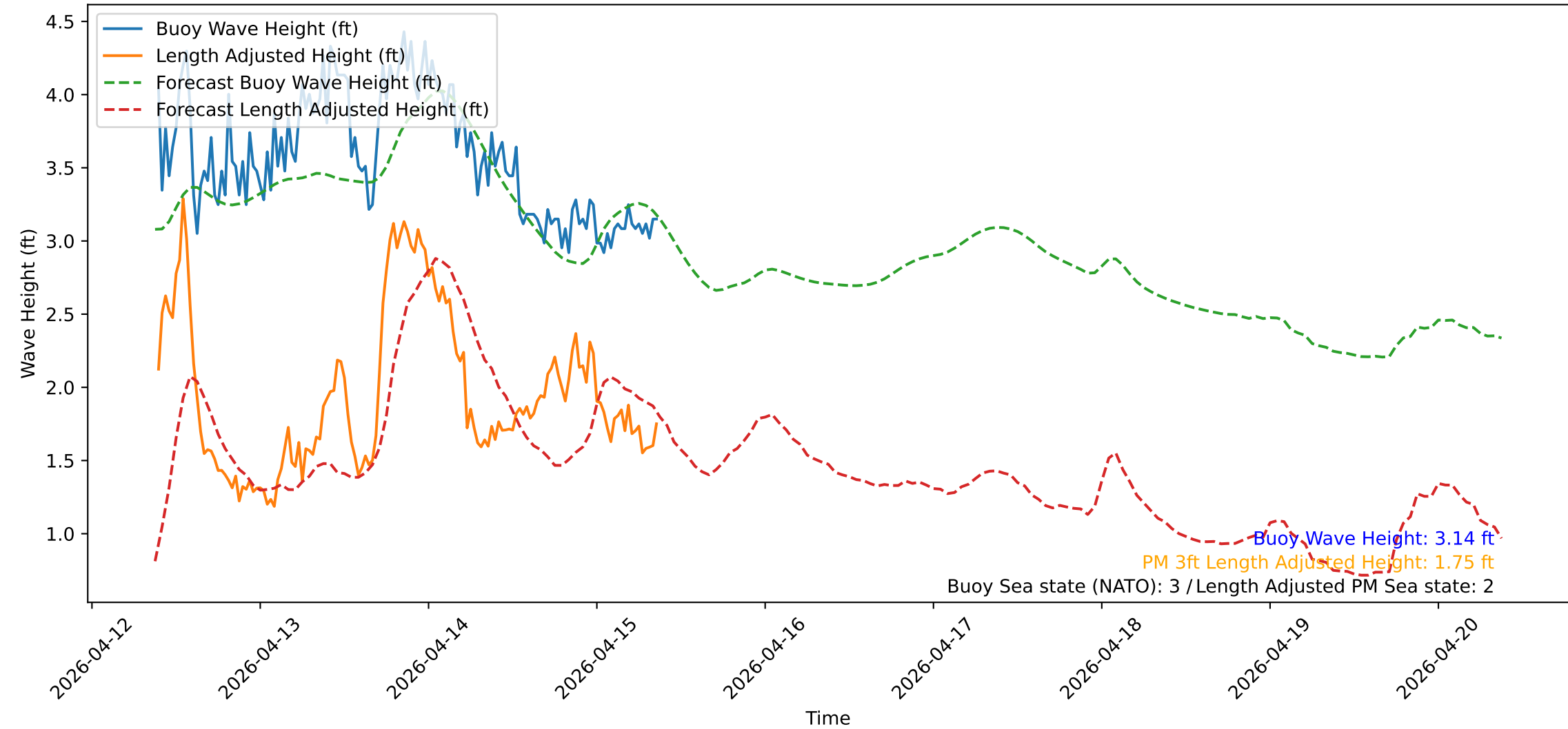
Wave Heights over Time for Red Beach at 2026-04-15 09:10:50
