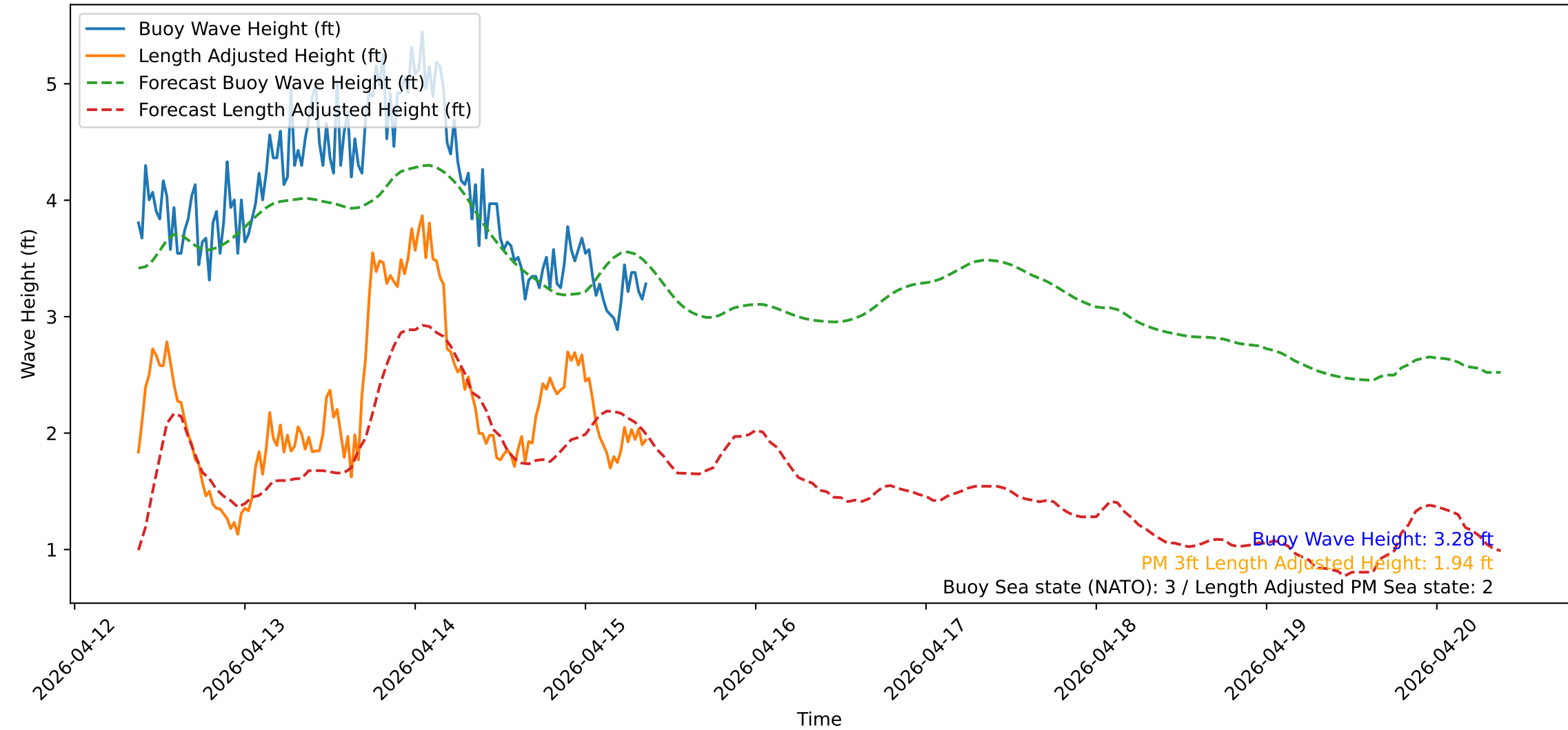
Wave Heights over Time for Oceanside Harbor at 2026-04-15 09:10:31
