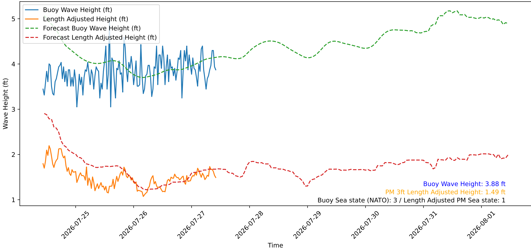
Wave Heights over Time for Oceanside Harbor at 2026-07-27 10:40:26
