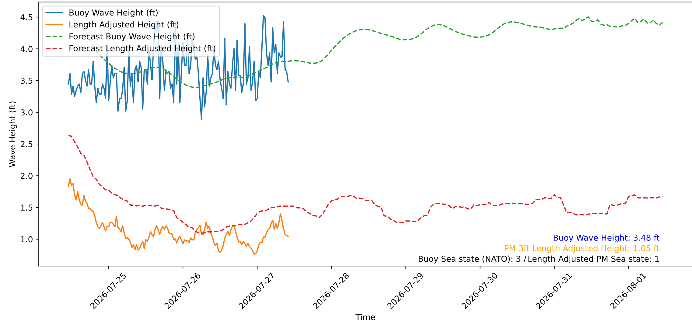
Wave Heights over Time for Red Beach at 2026-07-27 10:40:46
