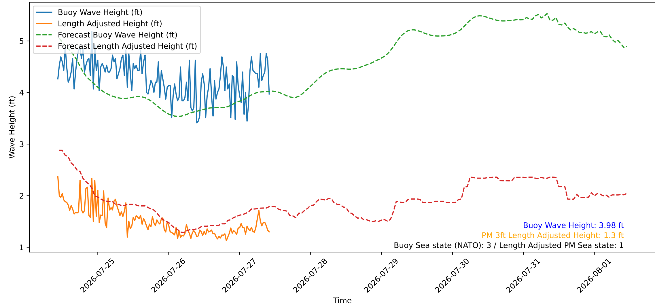
Wave Heights over Time for Green Beach at 2026-07-27 10:41:09
