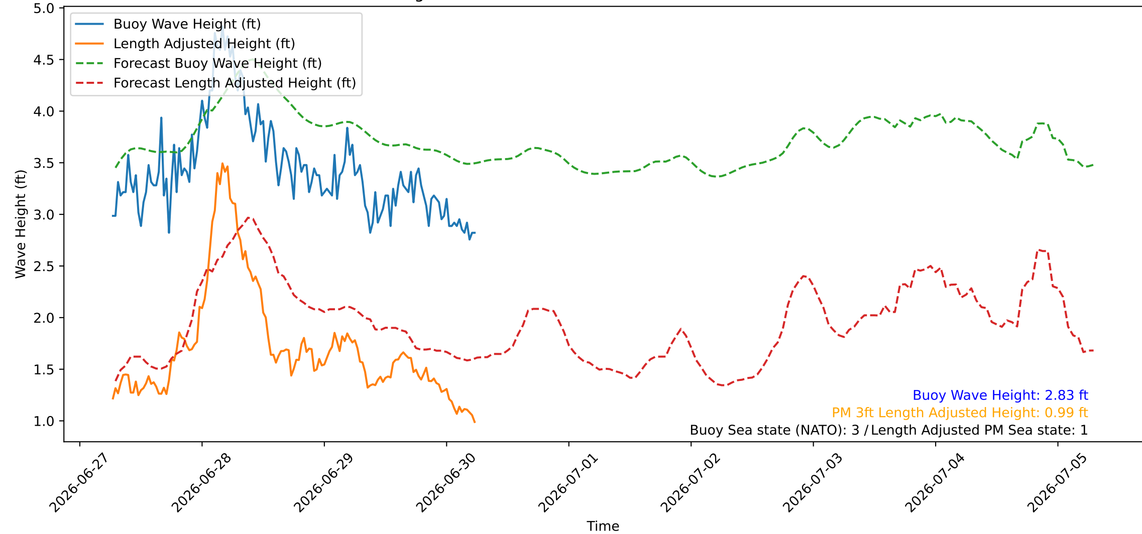
Wave Heights over Time for Green Beach at 2026-06-30 06:31:07
