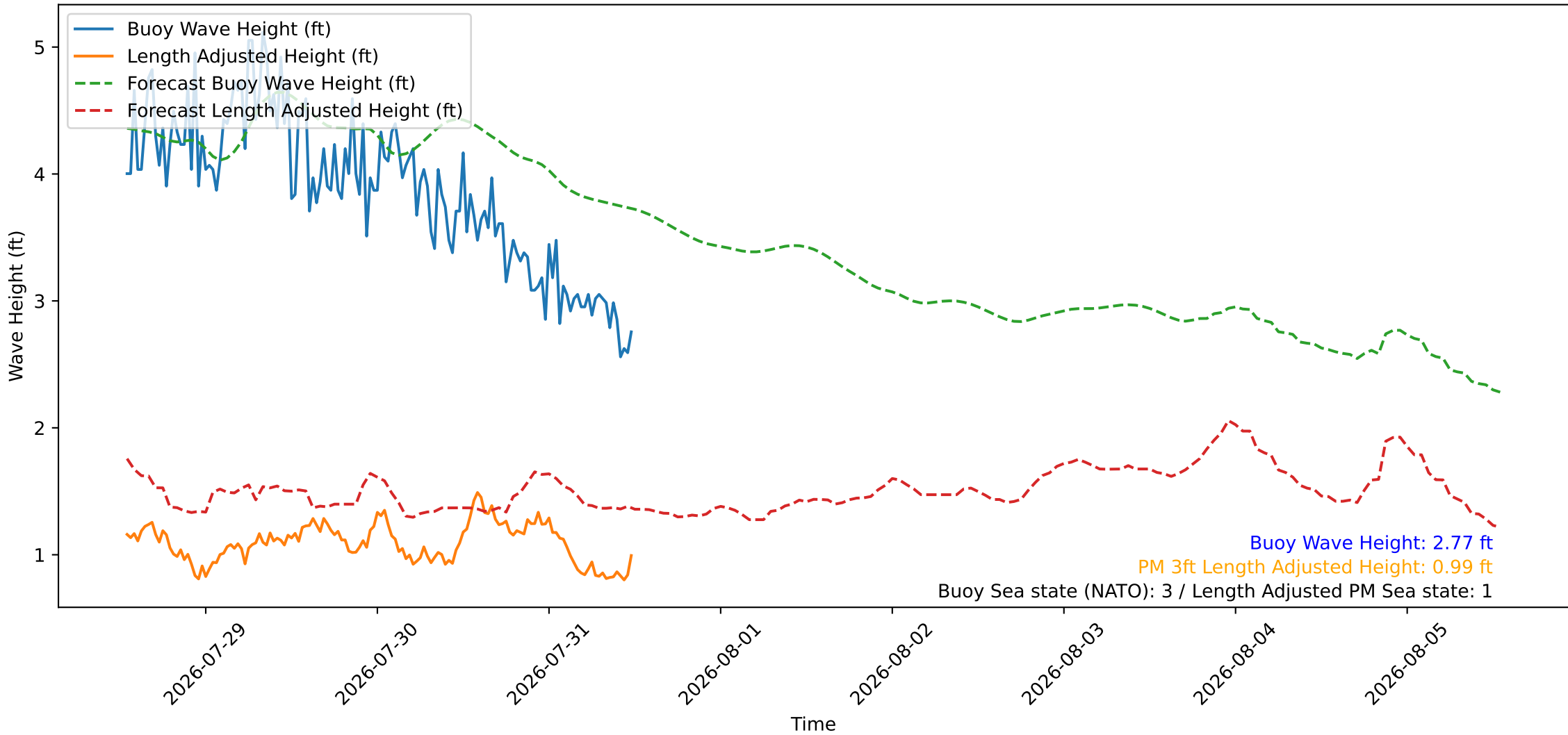
Wave Heights over Time for Red Beach at 2026-07-31 12:40:47
