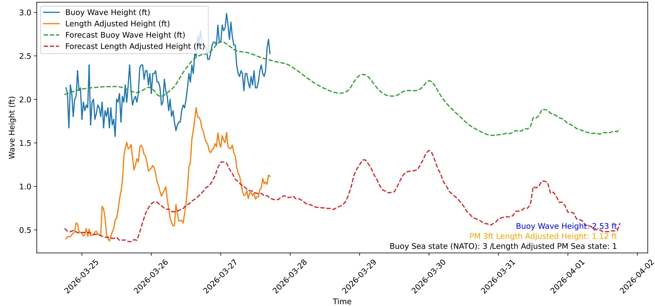
Wave Heights over Time for Red Beach at 2026-03-27 18:00:47
