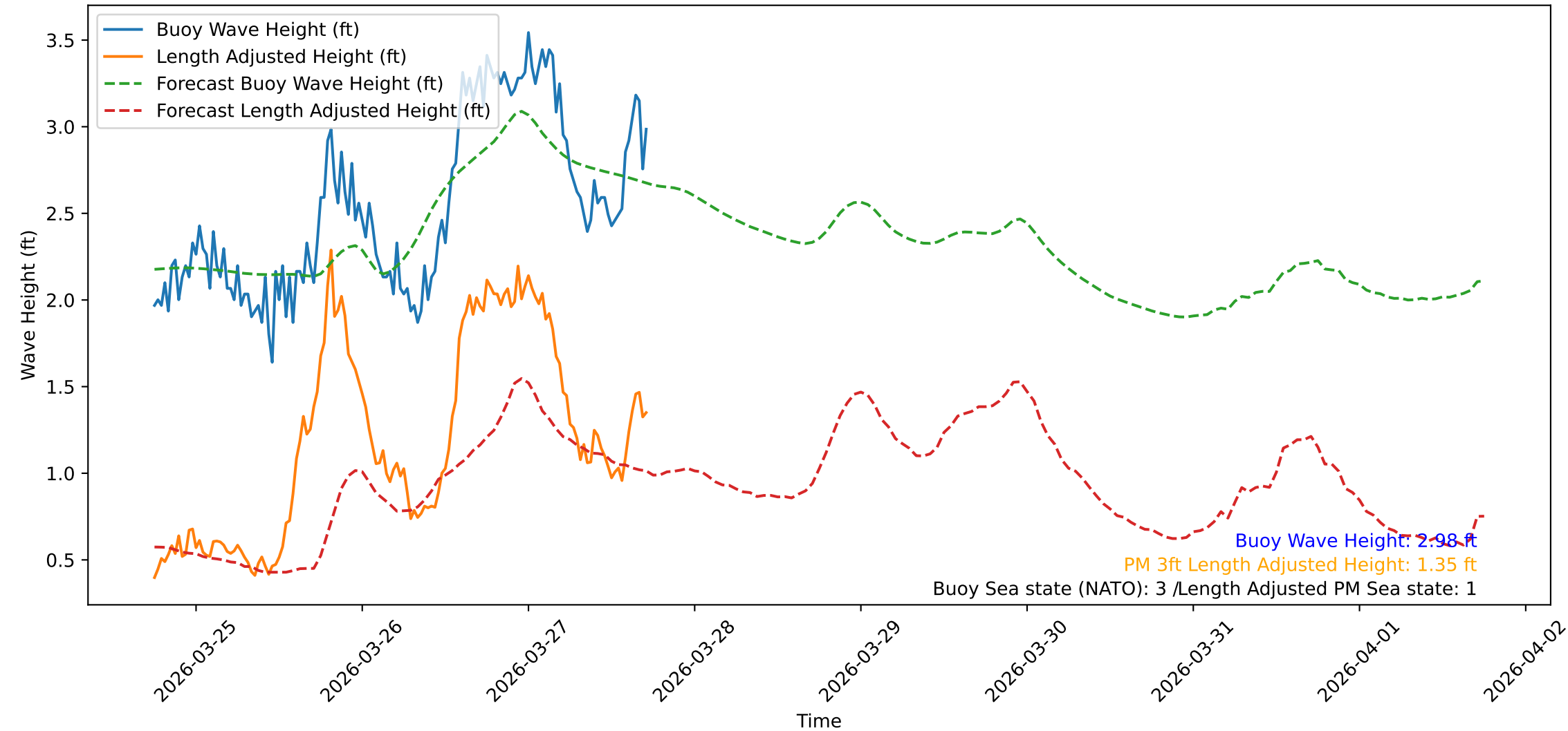
Wave Heights over Time for Green Beach at 2026-03-27 18:01:08
