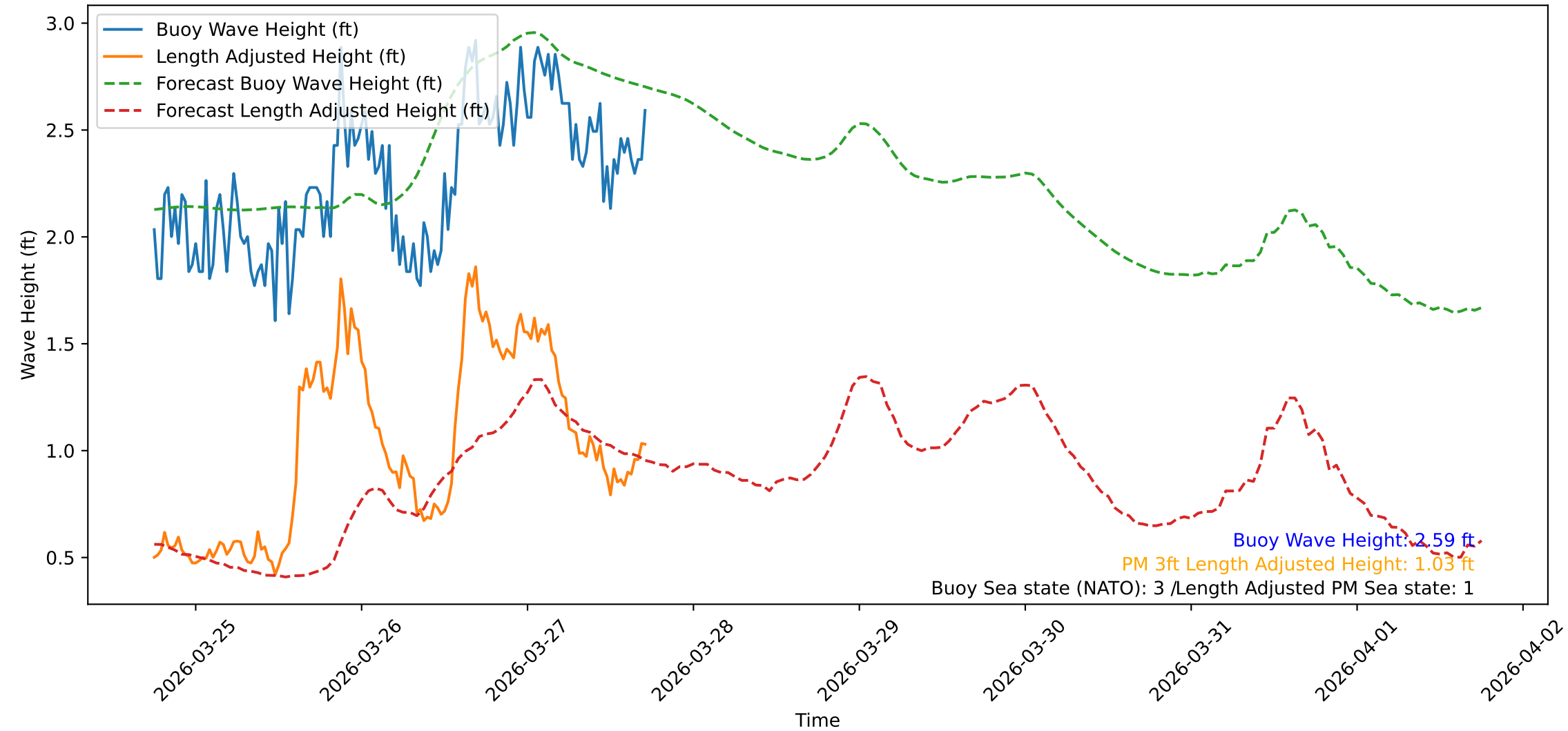
Wave Heights over Time for Oceanside Harbor at 2026-03-27 18:00:31
