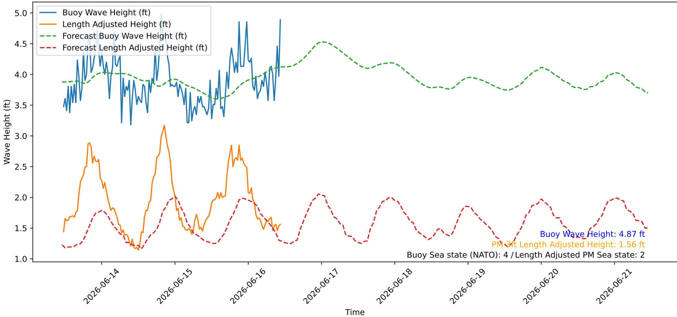
Wave Heights over Time for Oceanside Harbor at 2026-06-16 11:20:25
