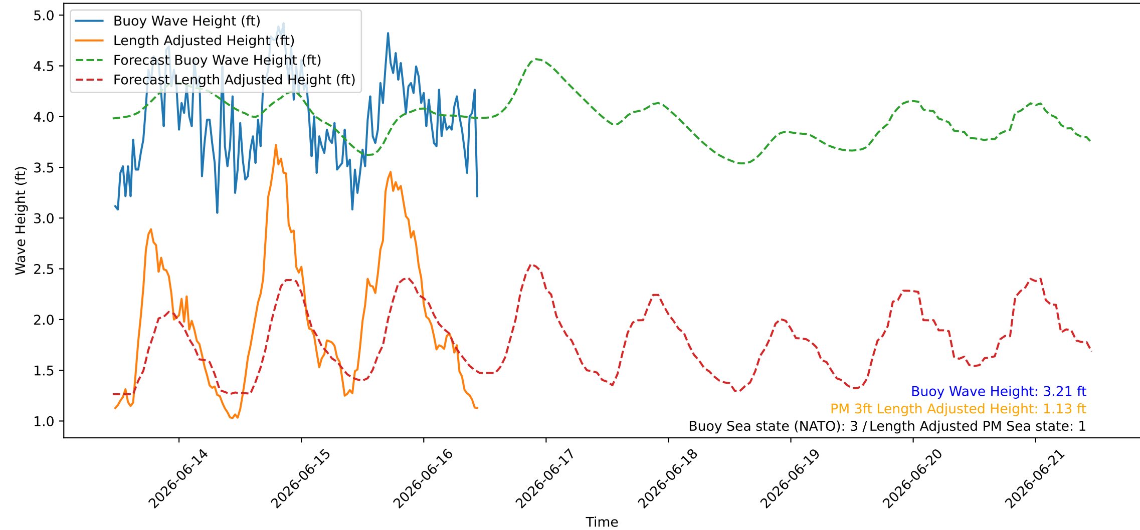
Wave Heights over Time for Green Beach at 2026-06-16 11:21:09
