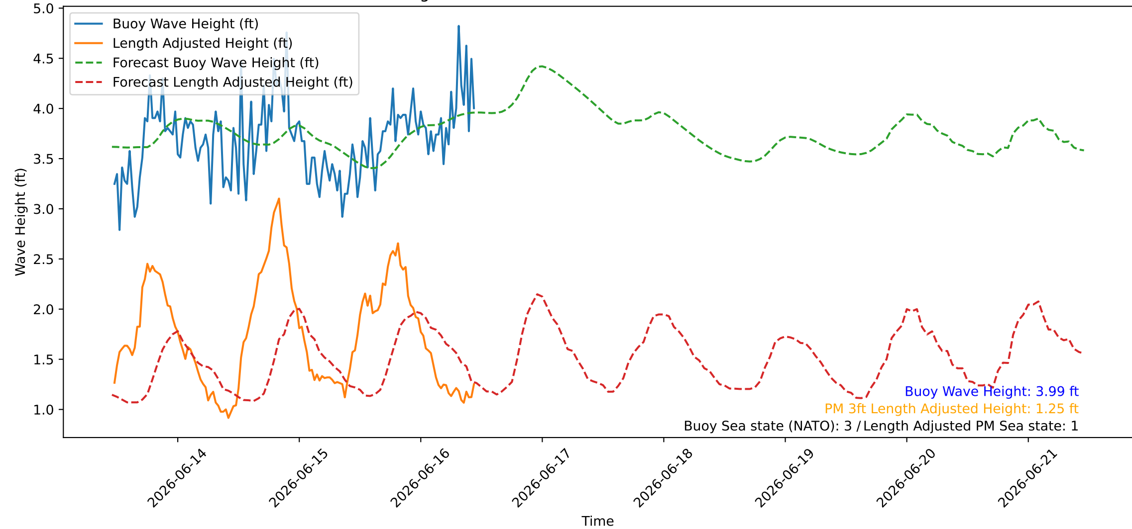
Wave Heights over Time for Red Beach at 2026-06-16 11:20:46
