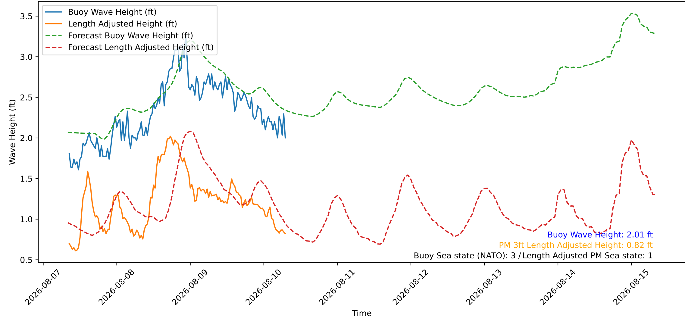
Wave Heights over Time for Red Beach at 2026-08-10 08:00:45
