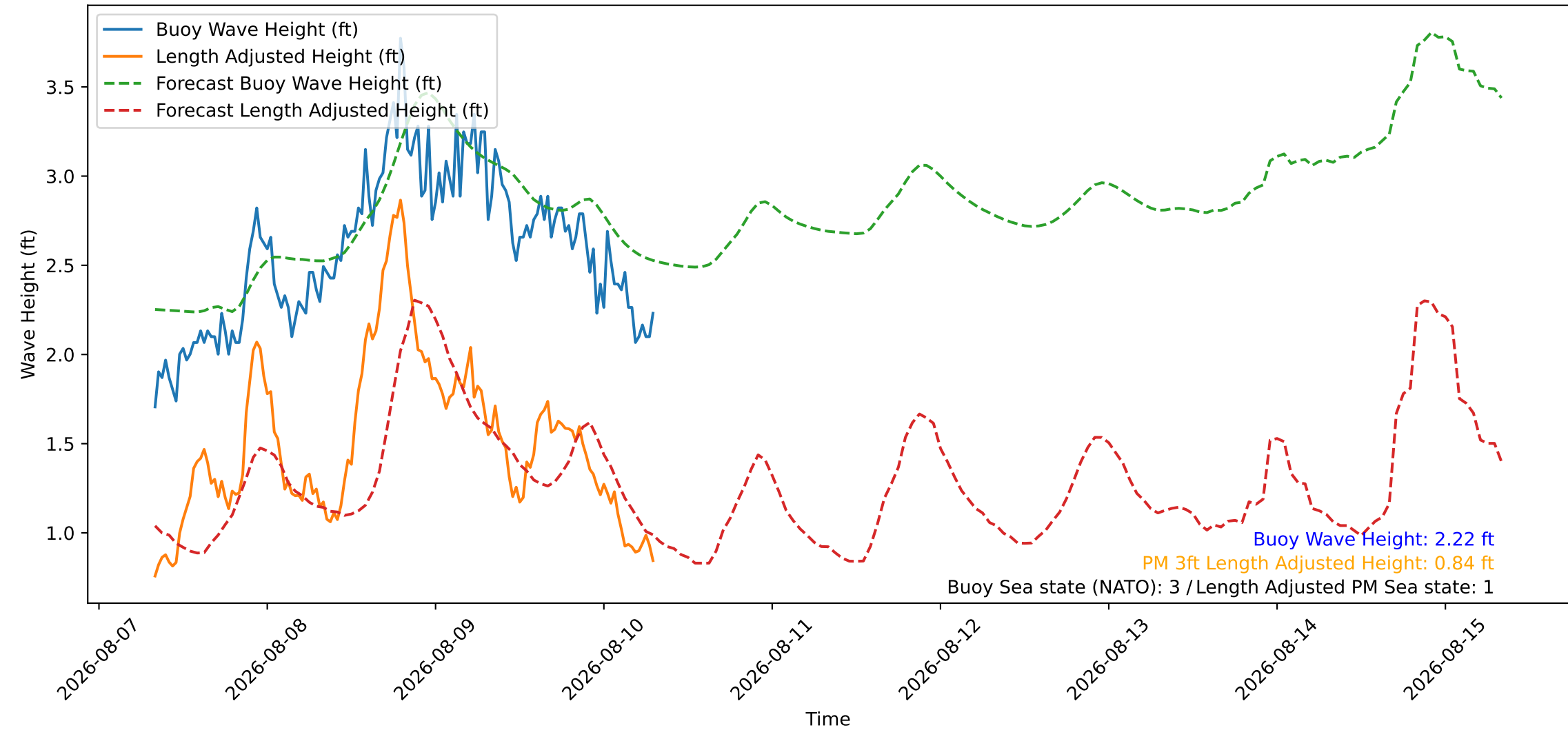
Wave Heights over Time for Green Beach at 2026-08-10 08:01:08
