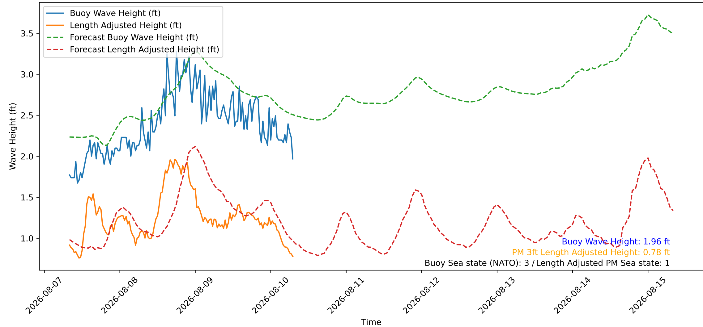
Wave Heights over Time for Oceanside Harbor at 2026-08-10 08:00:26
