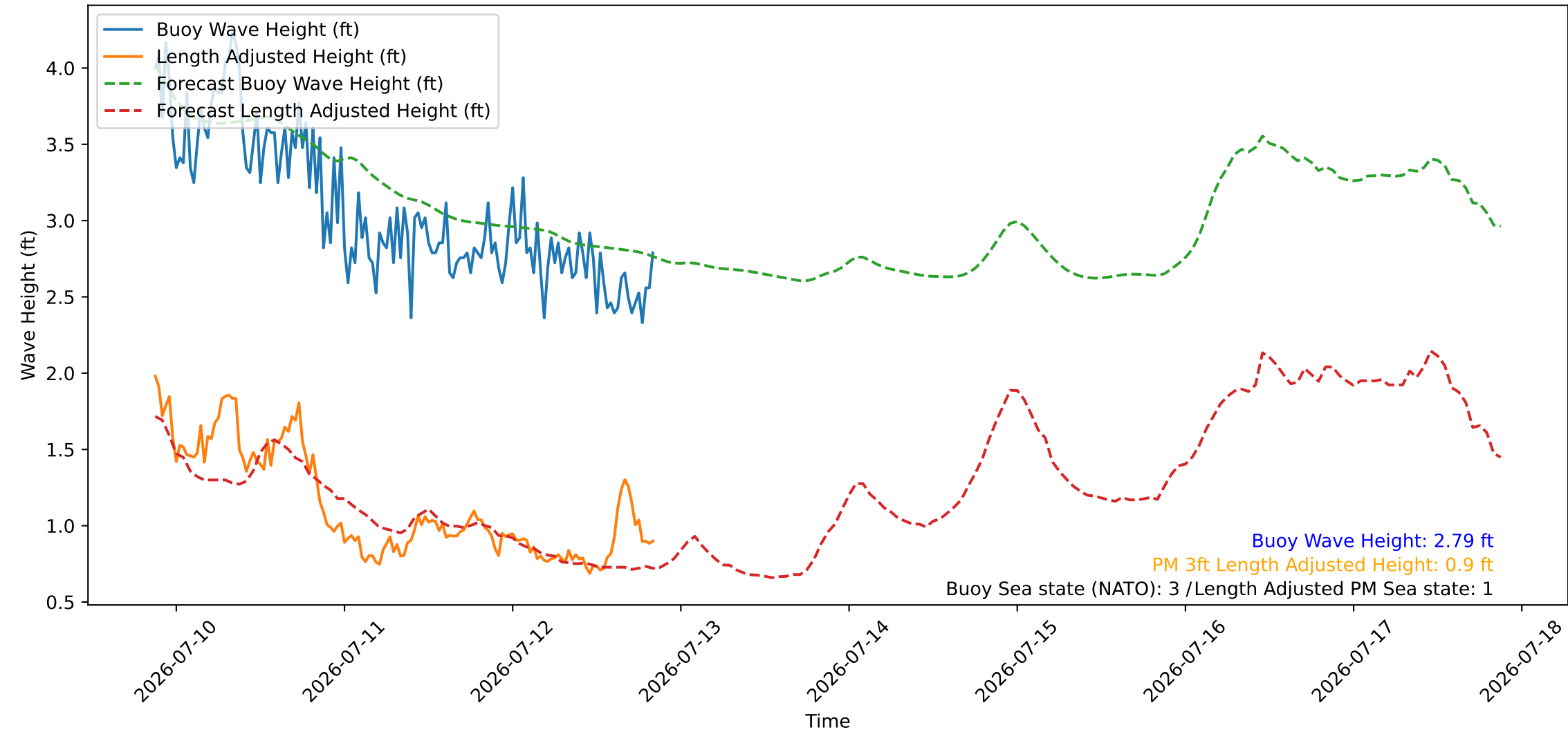
Wave Heights over Time for Oceanside Harbor at 2026-07-12 20:50:25
