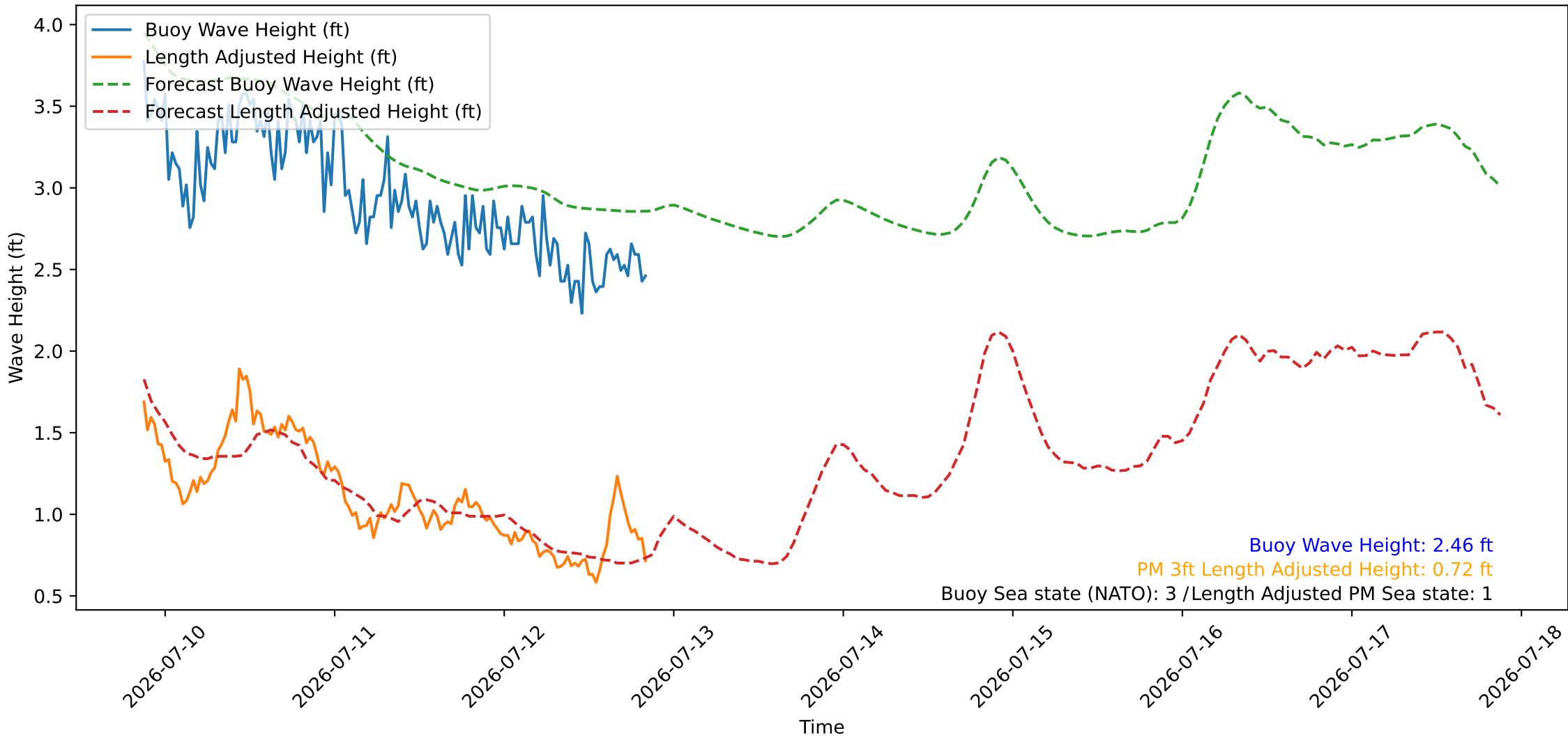
Wave Heights over Time for Green Beach at 2026-07-12 20:51:08
