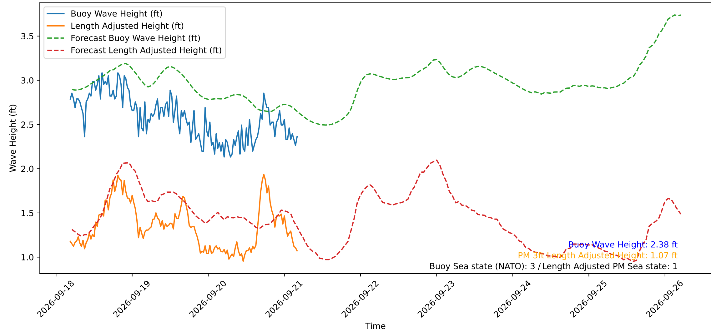
Wave Heights over Time for Oceanside Harbor at 2026-09-21 04:40:30
