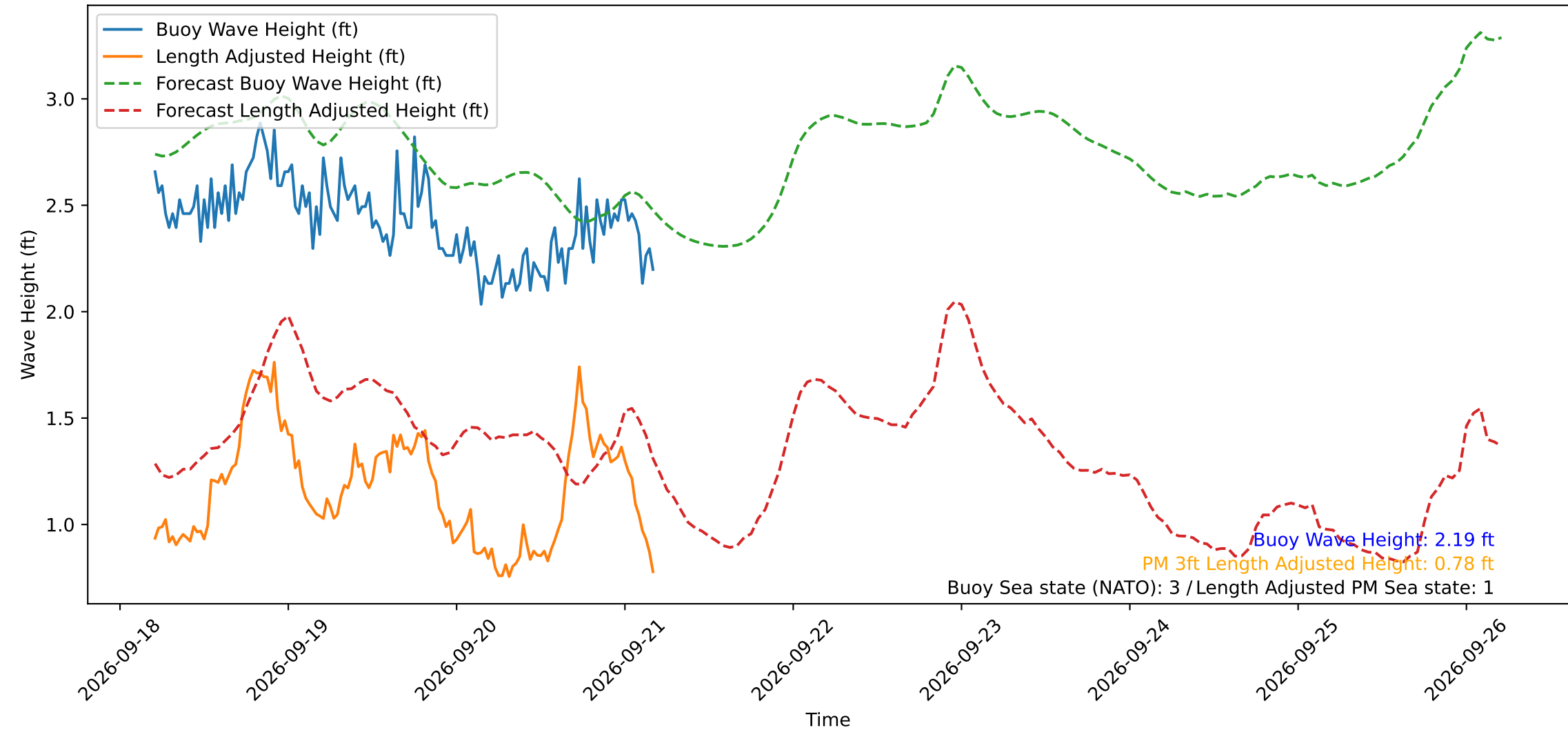
Wave Heights over Time for Red Beach at 2026-09-21 04:40:49
