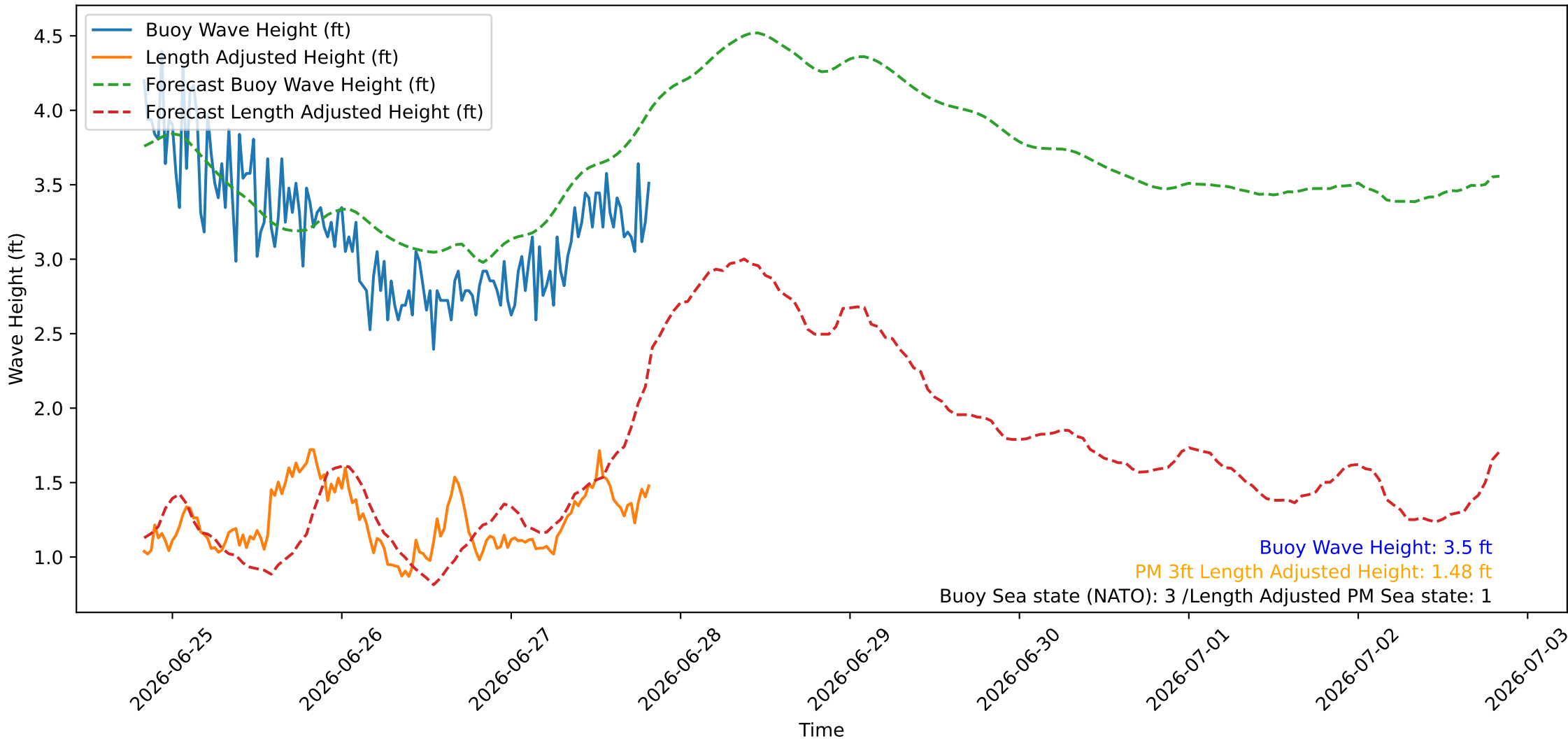
Wave Heights over Time for Oceanside Harbor at 2026-06-27 20:10:26
