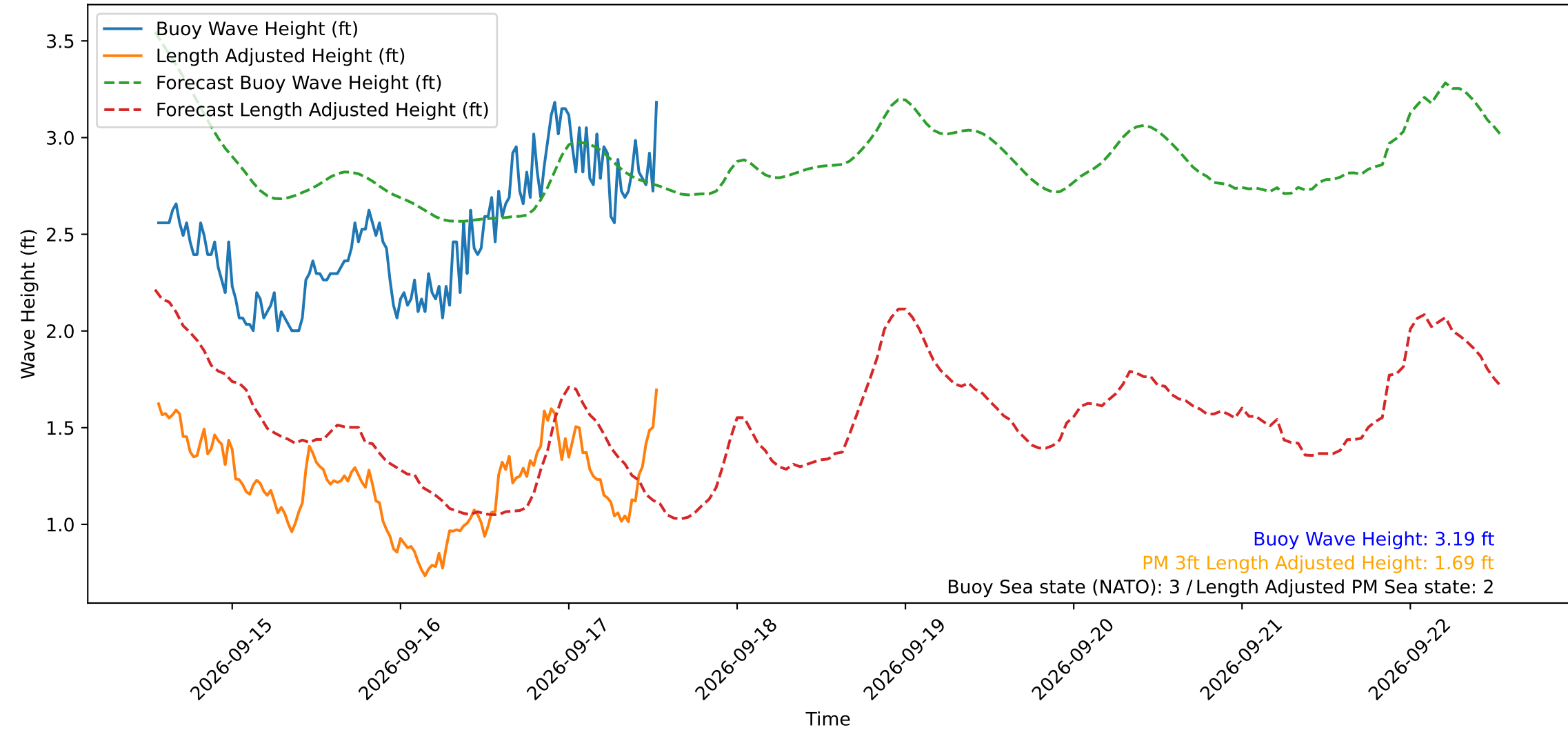
Wave Heights over Time for Red Beach at 2026-09-17 13:10:49
