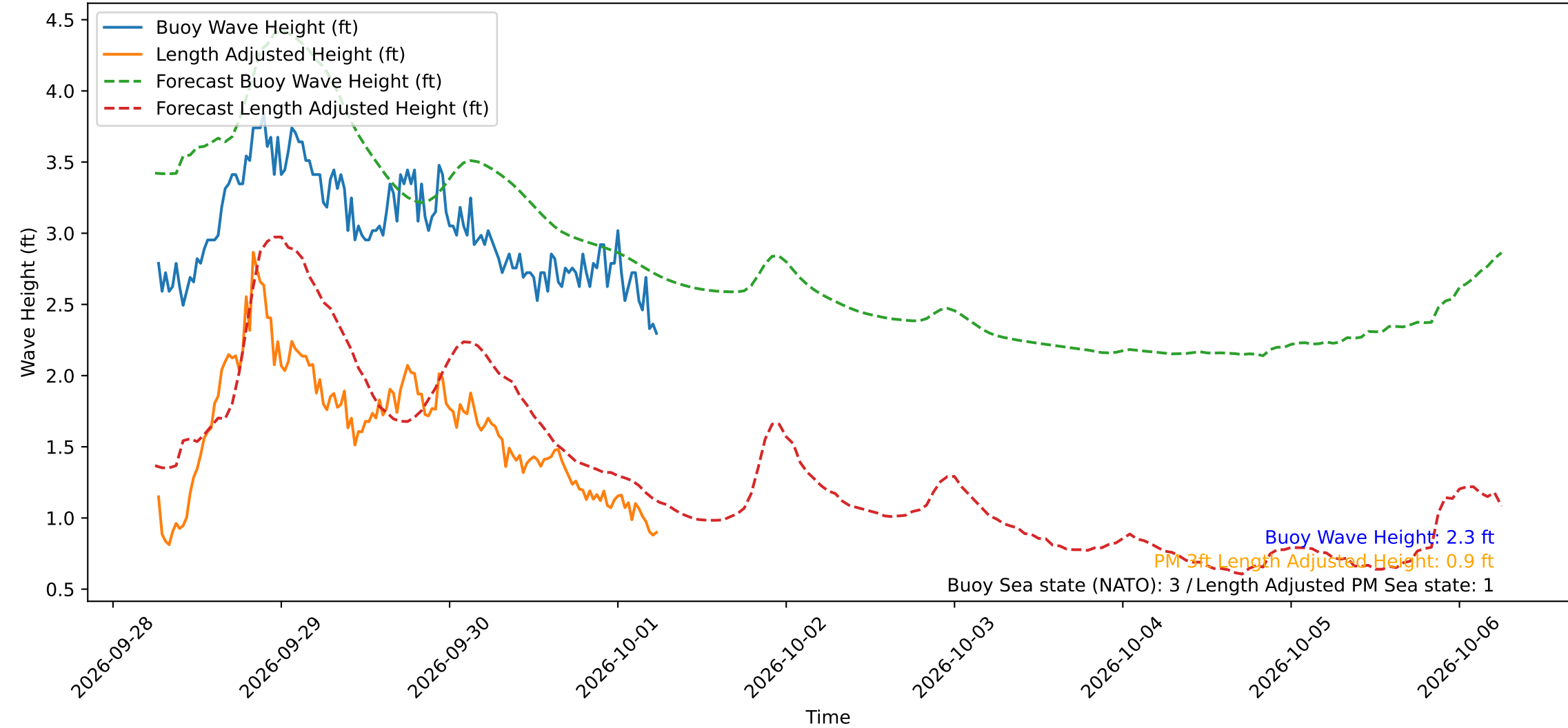
Wave Heights over Time for Red Beach at 2026-10-01 06:10:49
