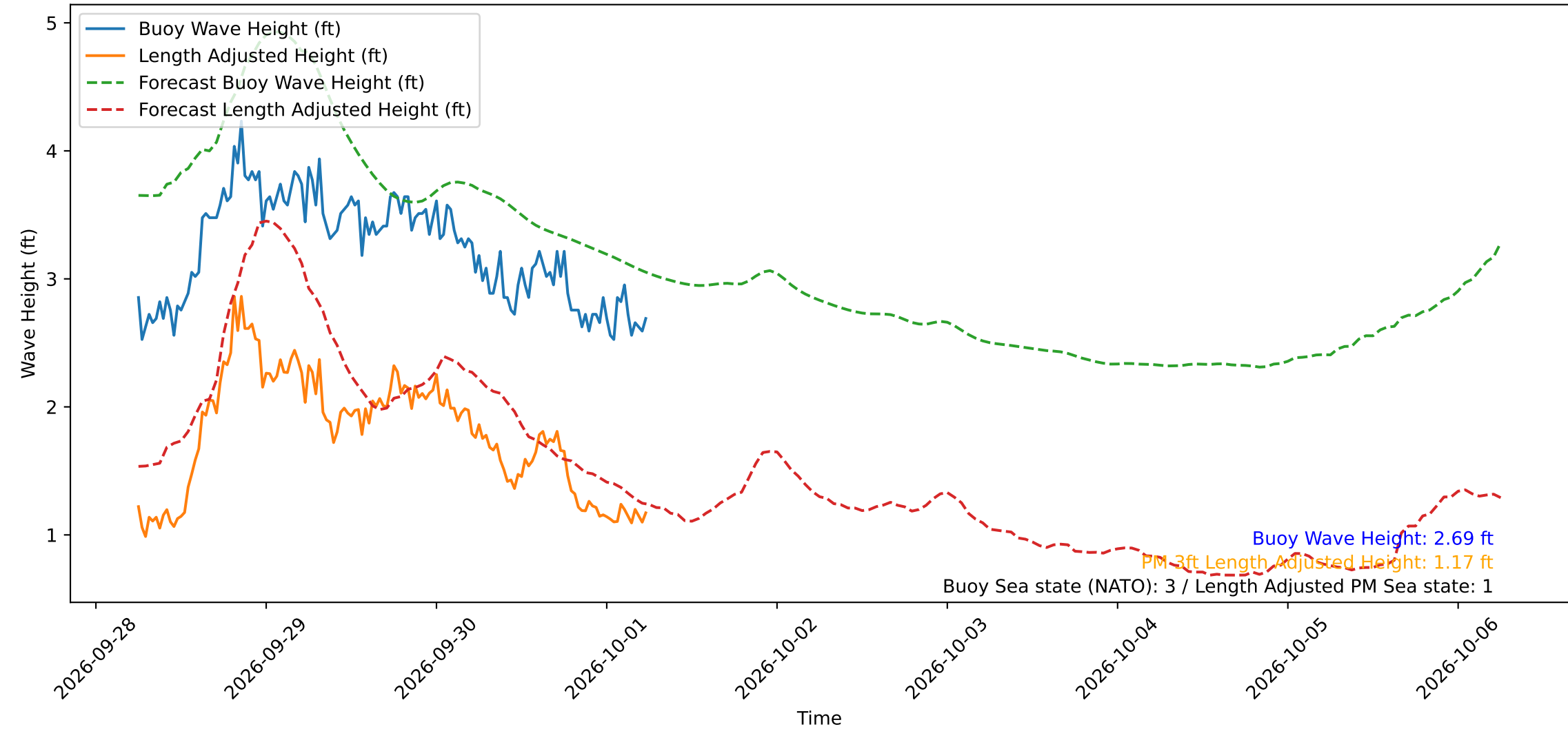
Wave Heights over Time for Oceanside Harbor at 2026-10-01 06:10:30
