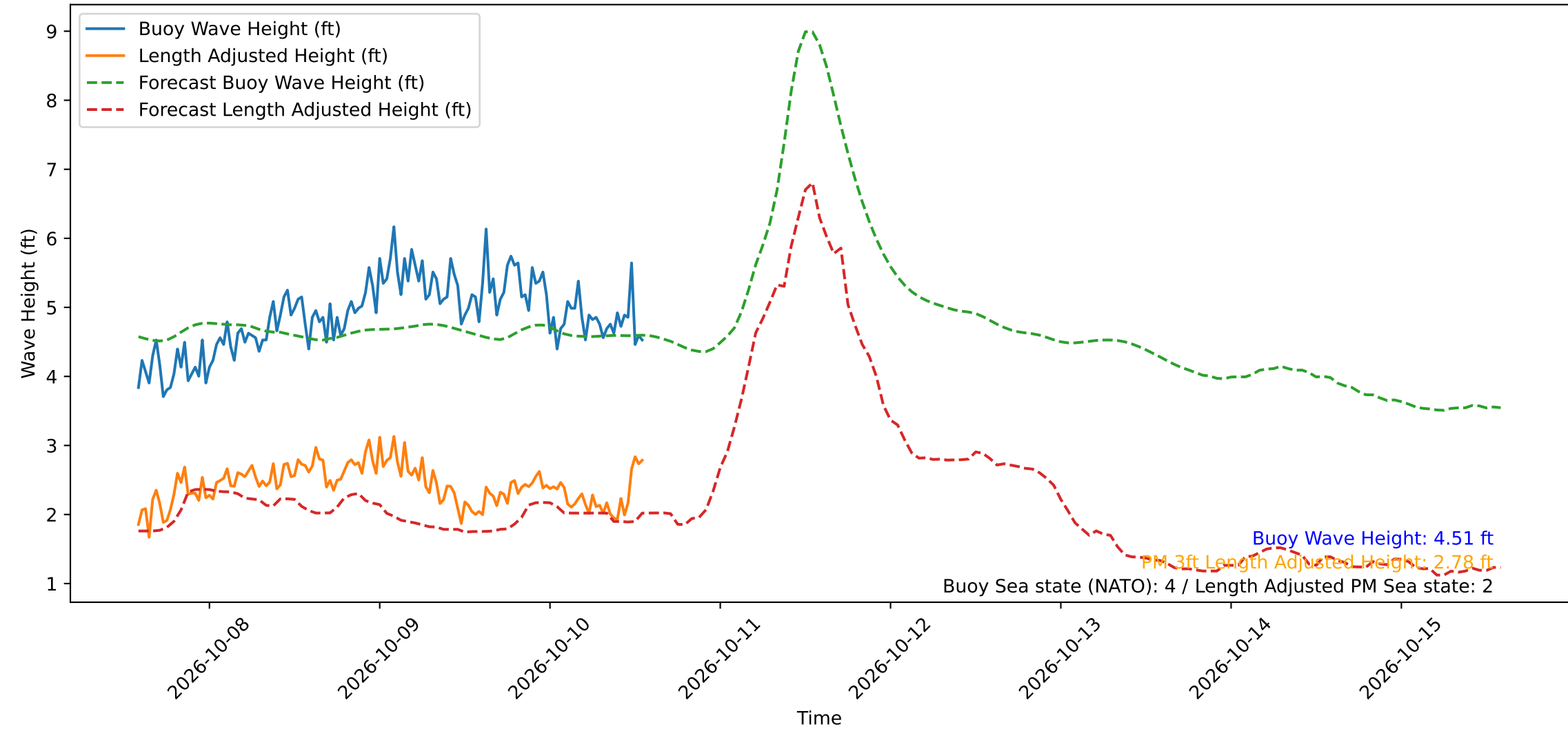
Wave Heights over Time for Green Beach at 2026-10-10 13:41:12
