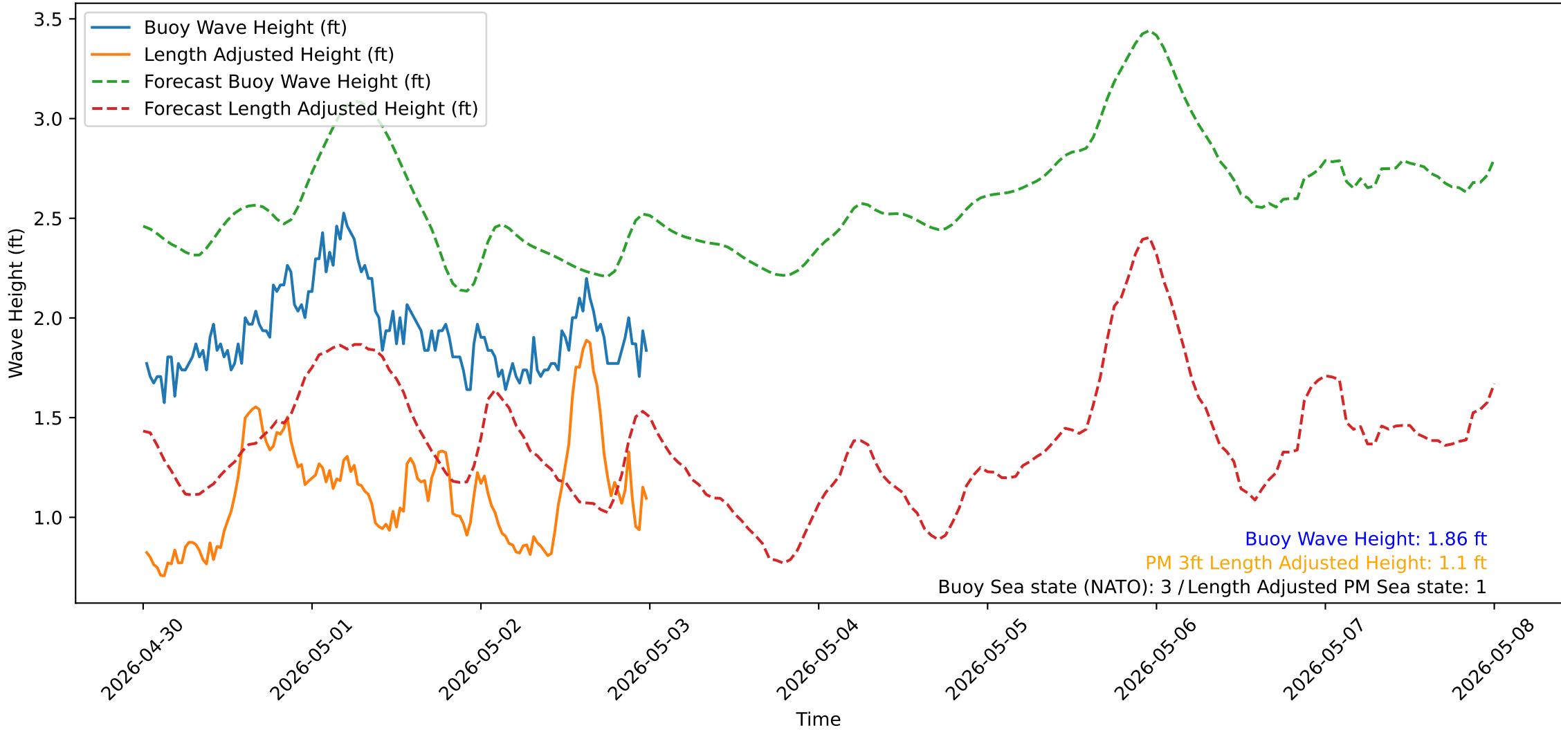
Wave Heights over Time for Red Beach at 2026-05-03 00:10:51
