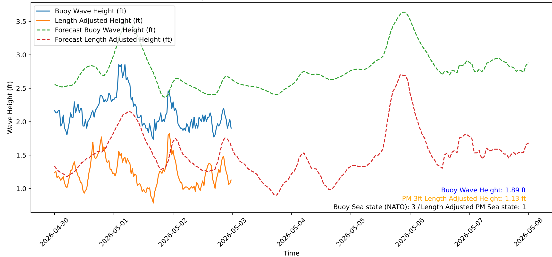
Wave Heights over Time for Green Beach at 2026-05-03 00:11:13
