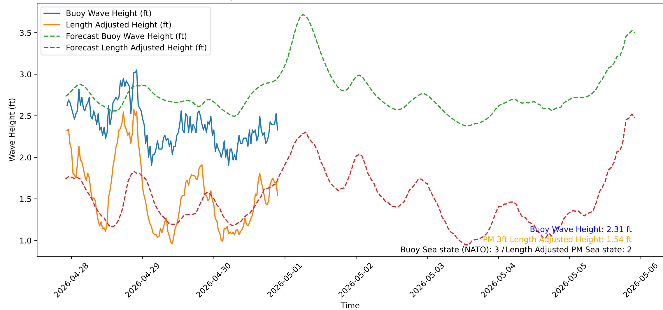
Wave Heights over Time for Oceanside Harbor at 2026-04-30 22:20:32
