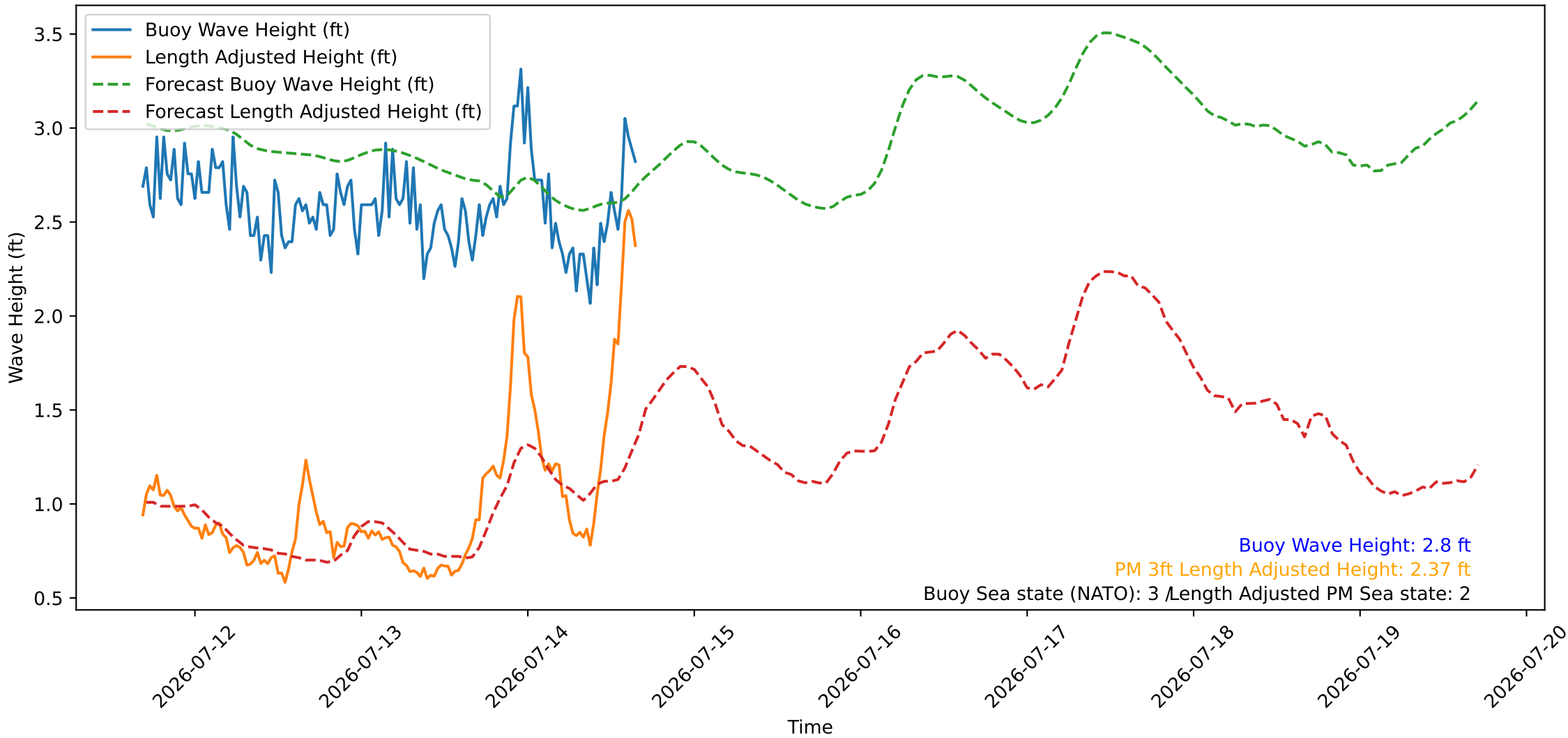
Wave Heights over Time for Green Beach at 2026-07-14 16:31:09
