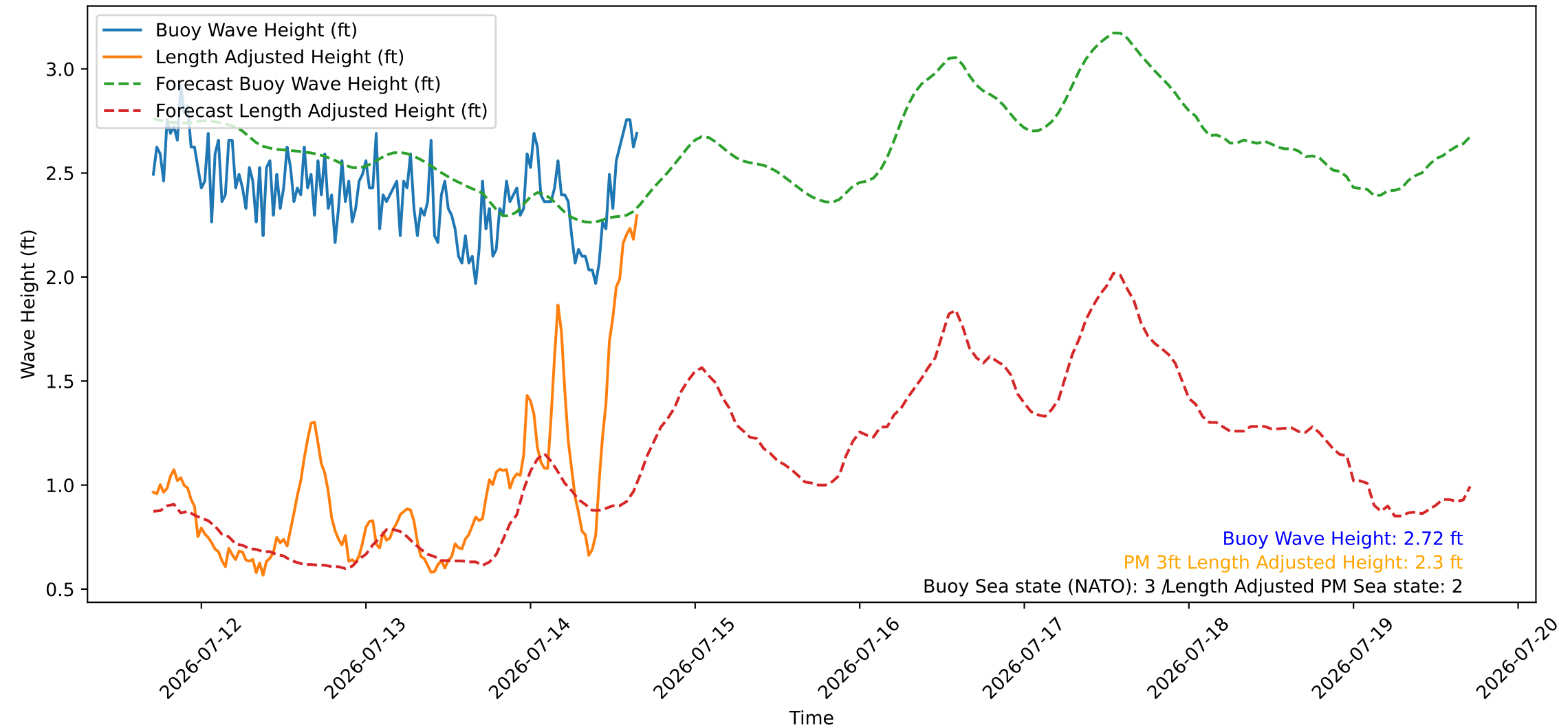
Wave Heights over Time for Red Beach at 2026-07-14 16:30:46
