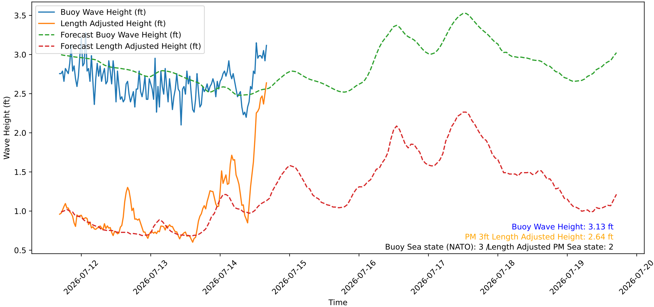
Wave Heights over Time for Oceanside Harbor at 2026-07-14 16:30:27
