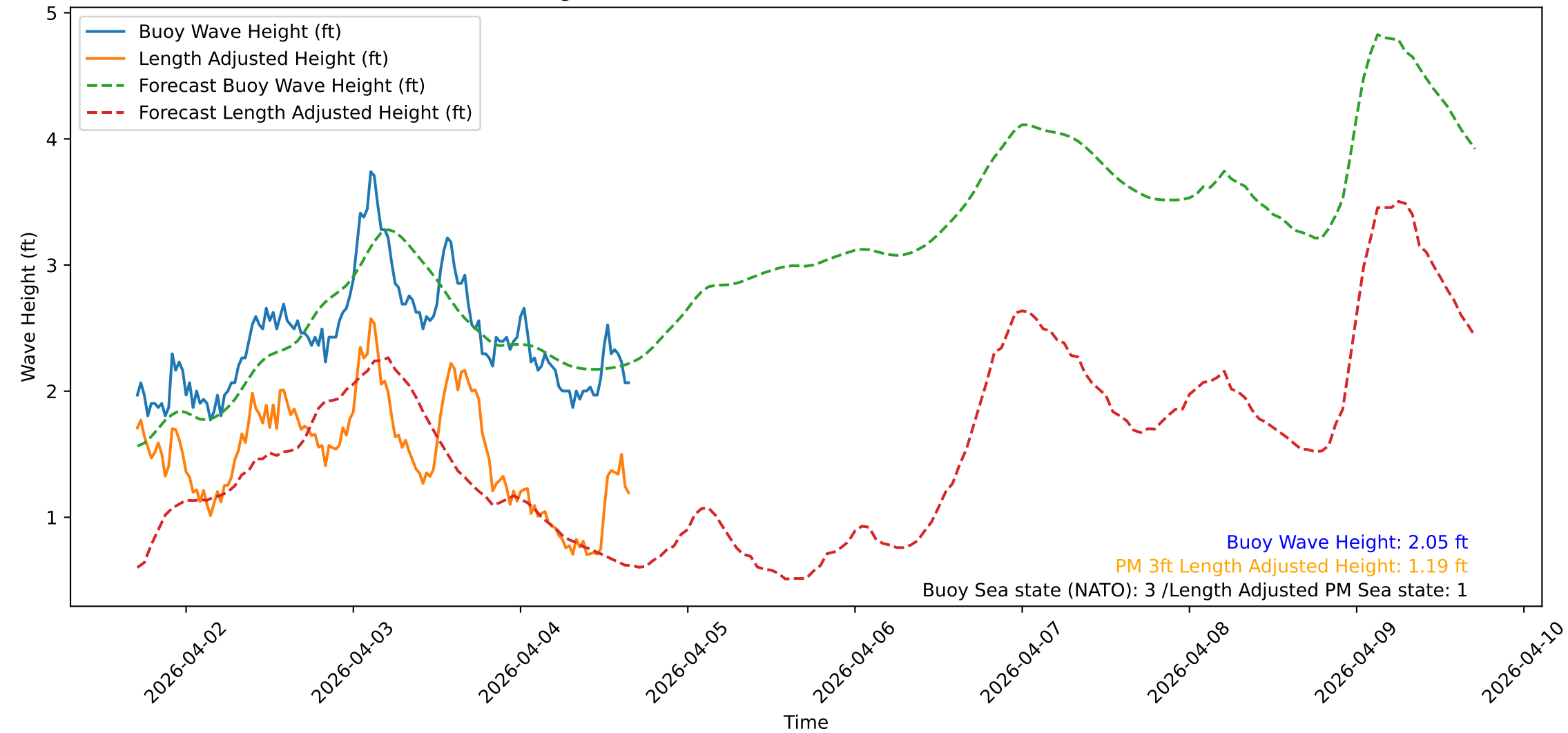
Wave Heights over Time for Red Beach at 2026-04-04 16:30:49
