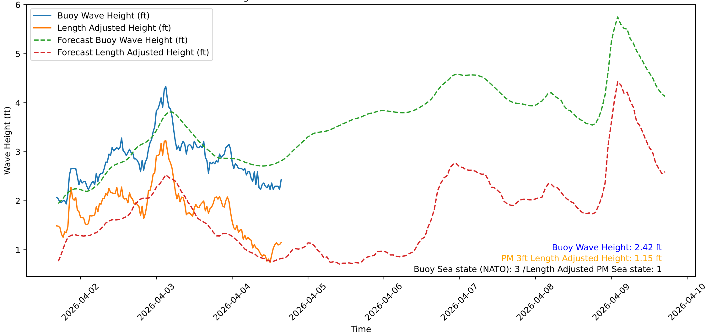
Wave Heights over Time for Green Beach at 2026-04-04 16:31:14
