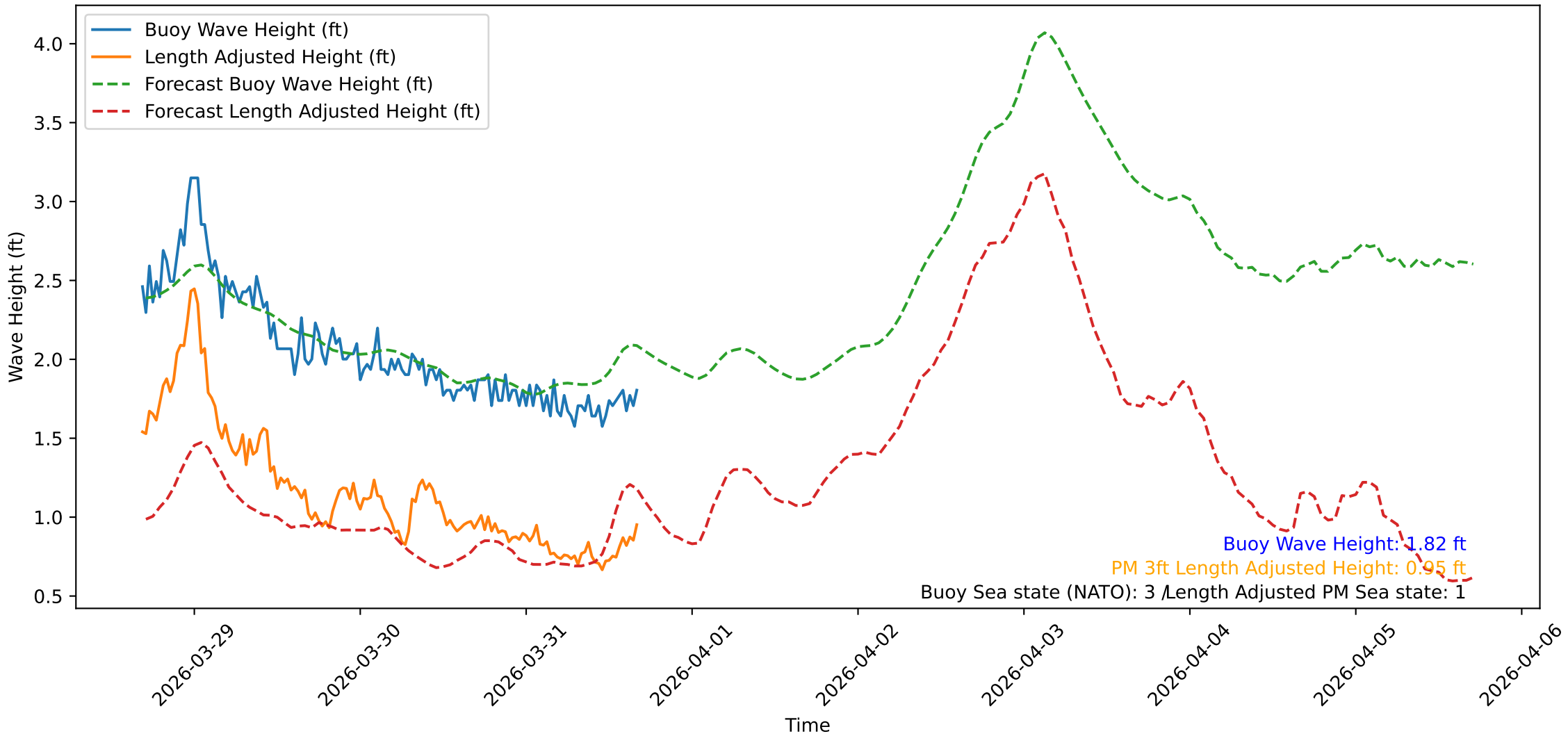
Wave Heights over Time for Oceanside Harbor at 2026-03-31 16:40:32
