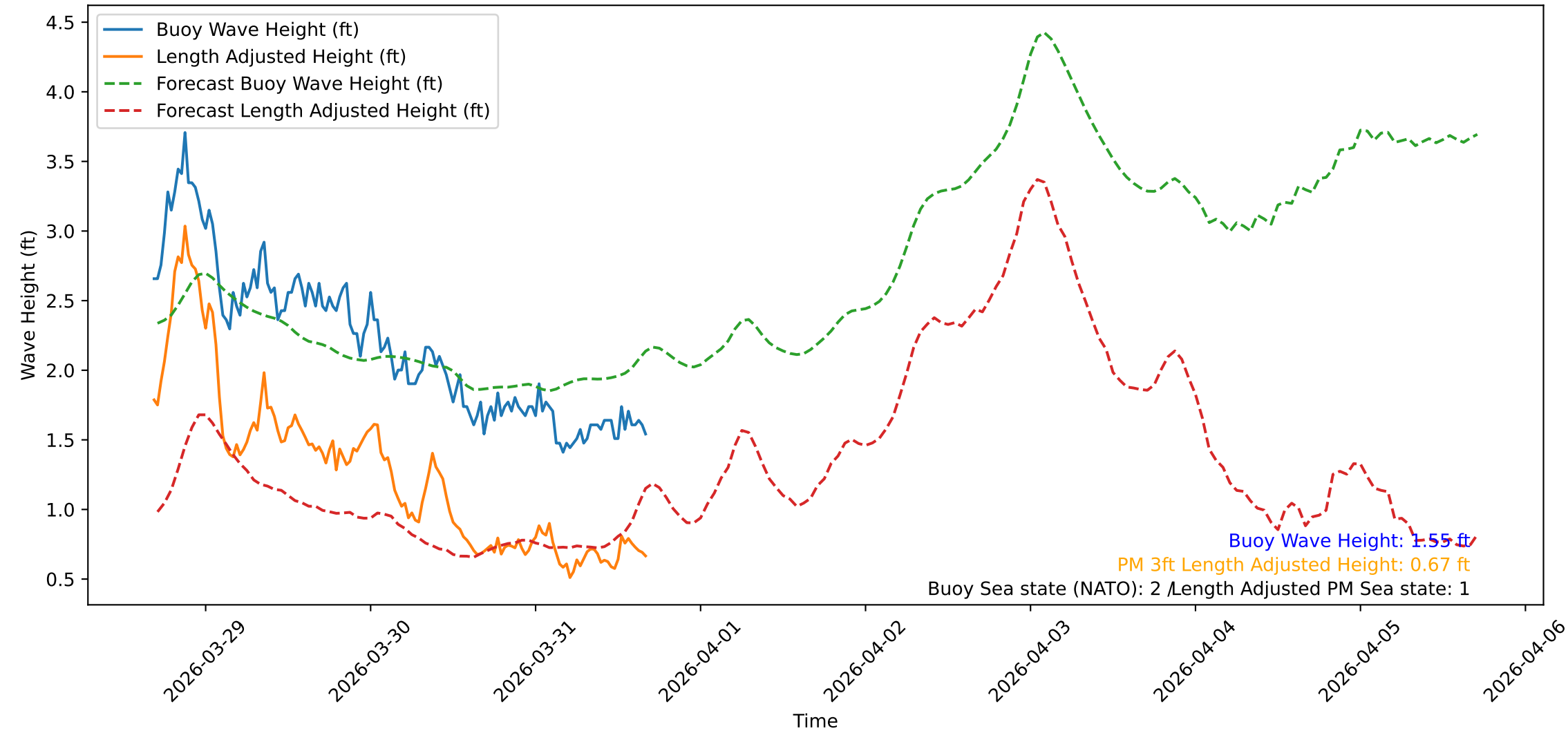
Wave Heights over Time for Green Beach at 2026-03-31 16:41:10
