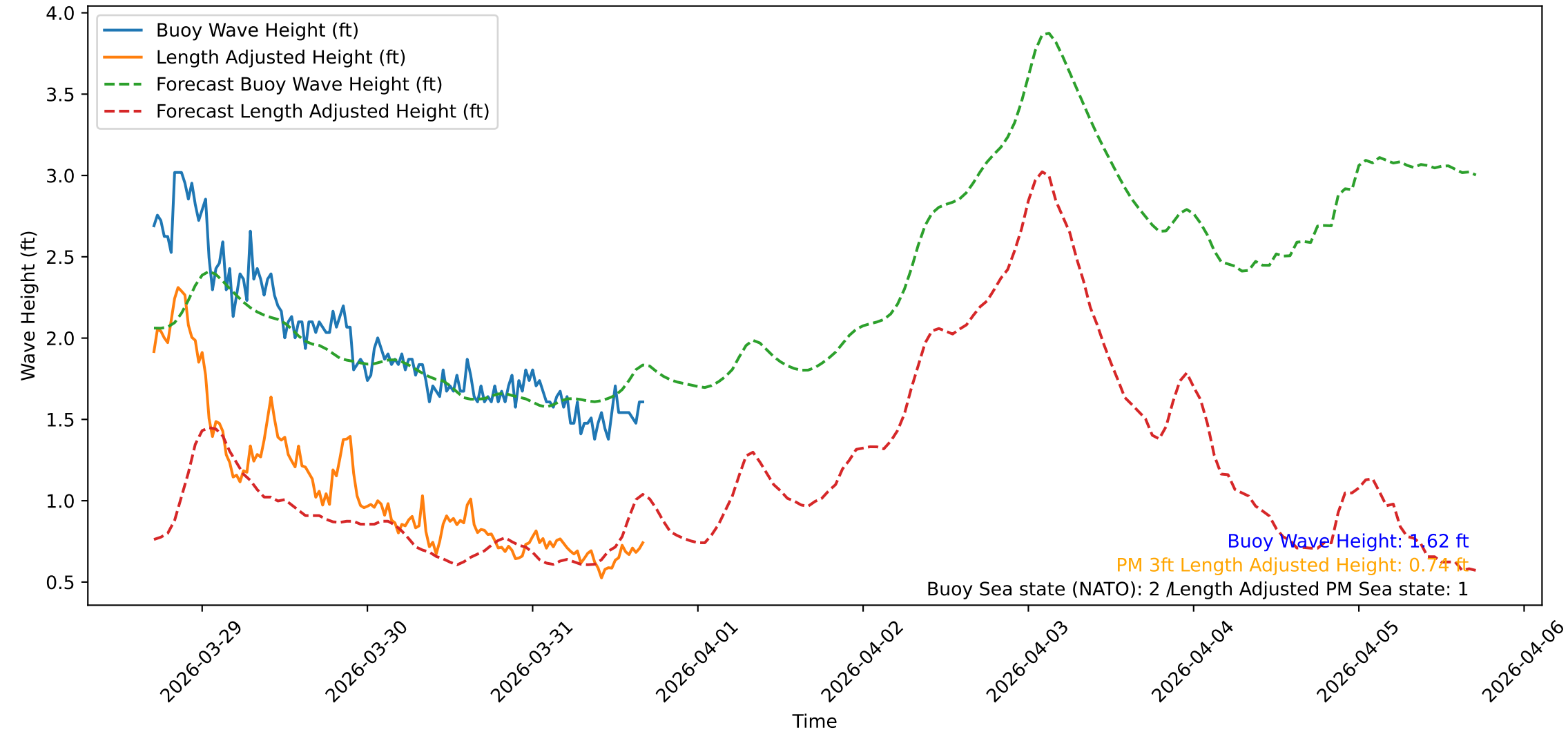
Wave Heights over Time for Red Beach at 2026-03-31 16:40:48
