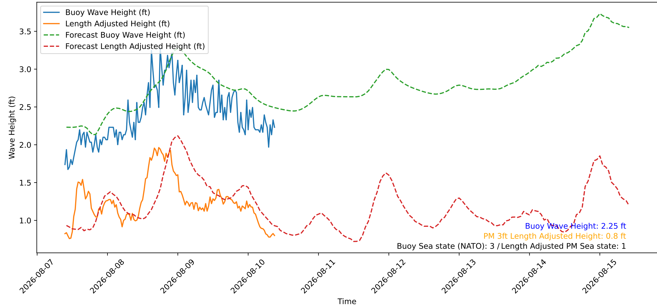
Wave Heights over Time for Oceanside Harbor at 2026-08-10 09:40:27
