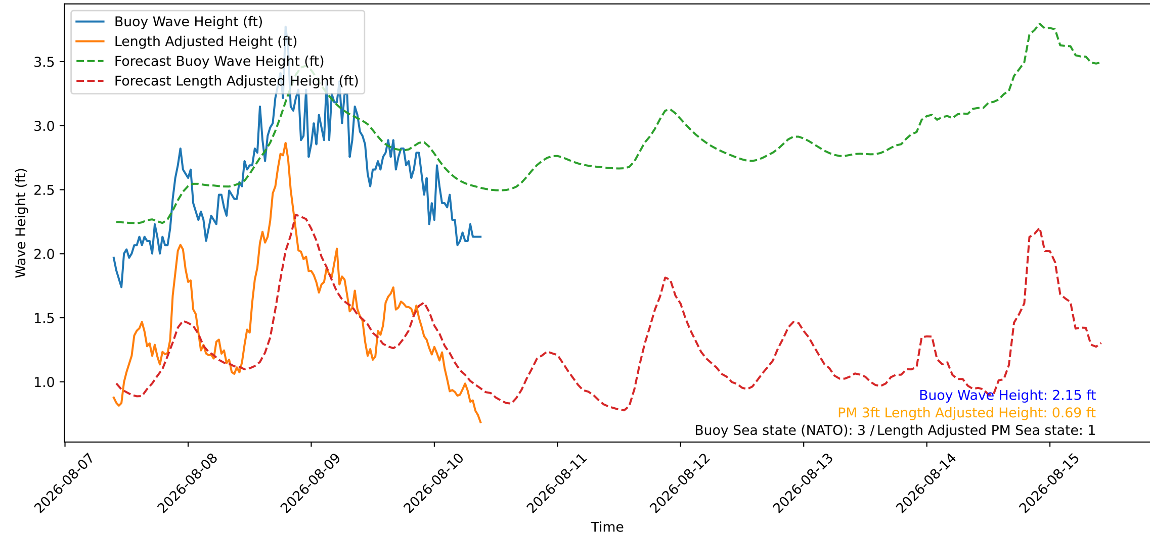
Wave Heights over Time for Green Beach at 2026-08-10 09:41:09
