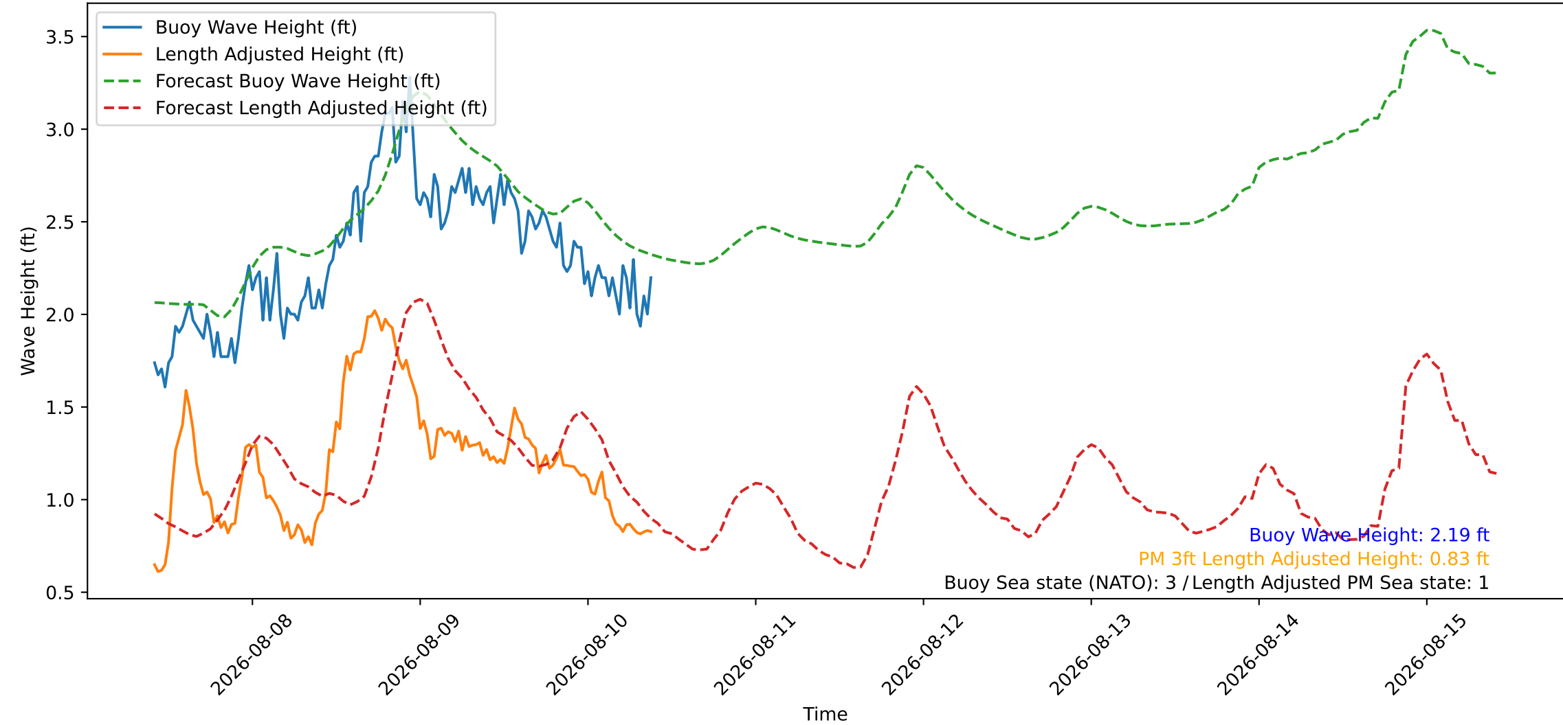
Wave Heights over Time for Red Beach at 2026-08-10 09:40:47
