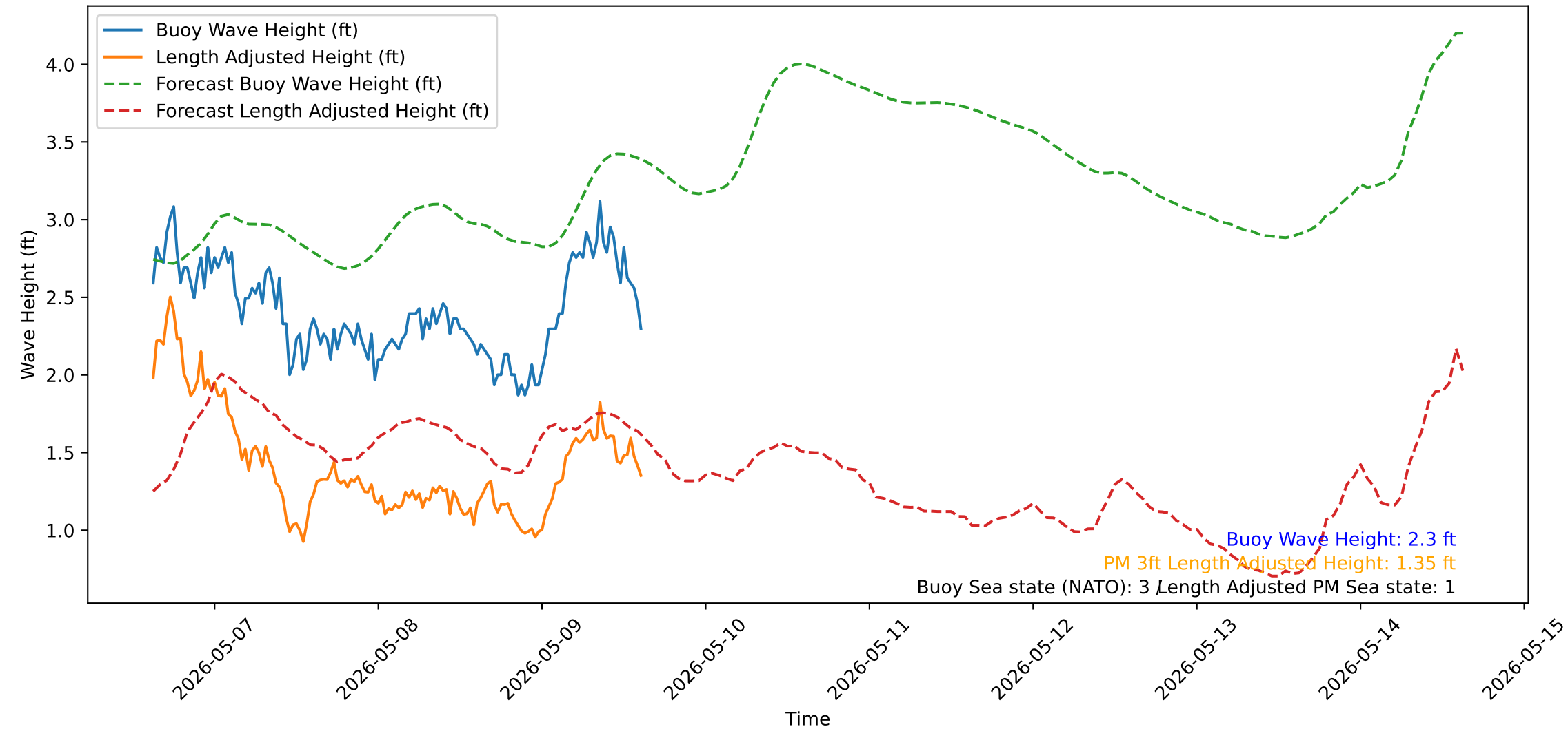
Wave Heights over Time for Oceanside Harbor at 2026-05-09 15:10:31
