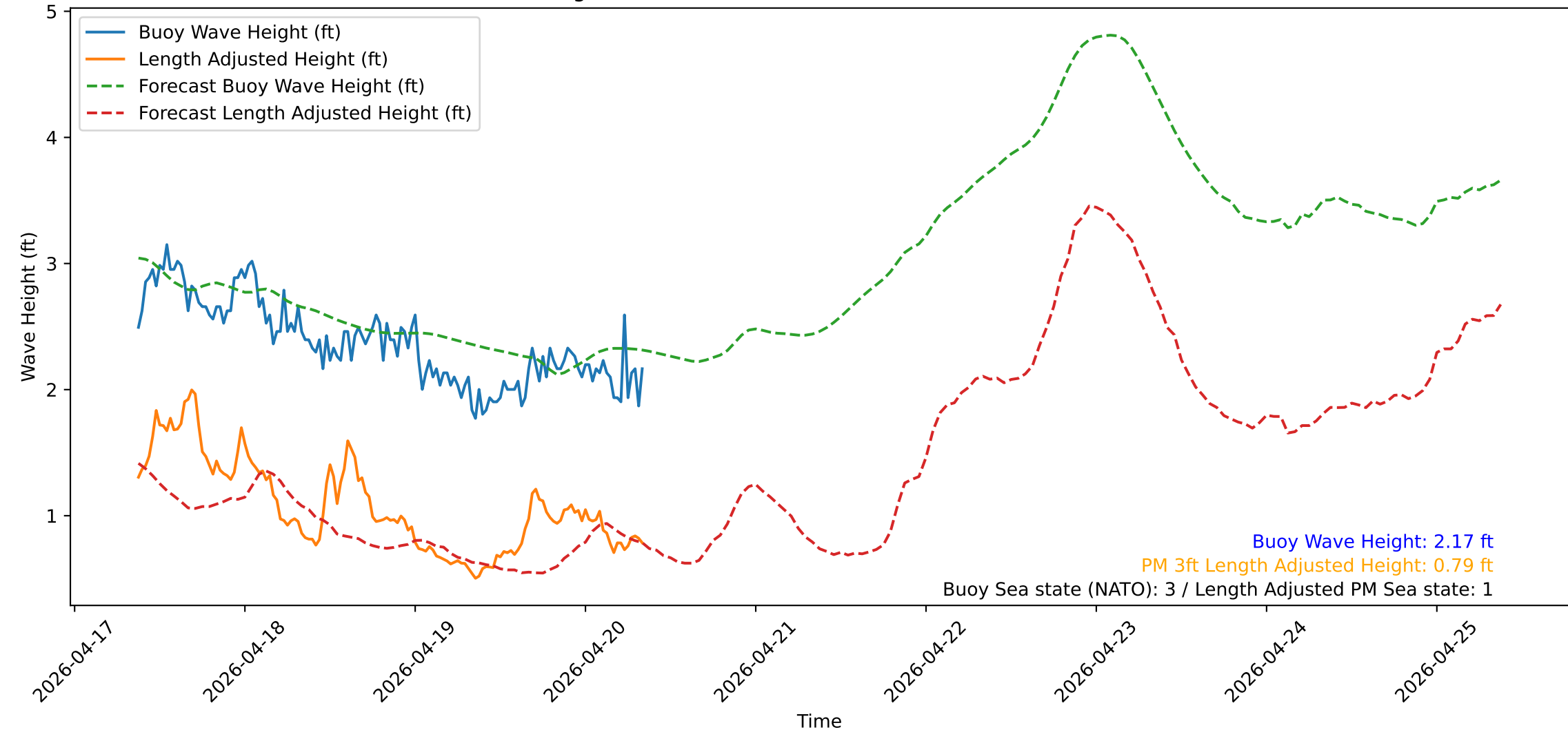
Wave Heights over Time for Red Beach at 2026-04-20 08:40:51
