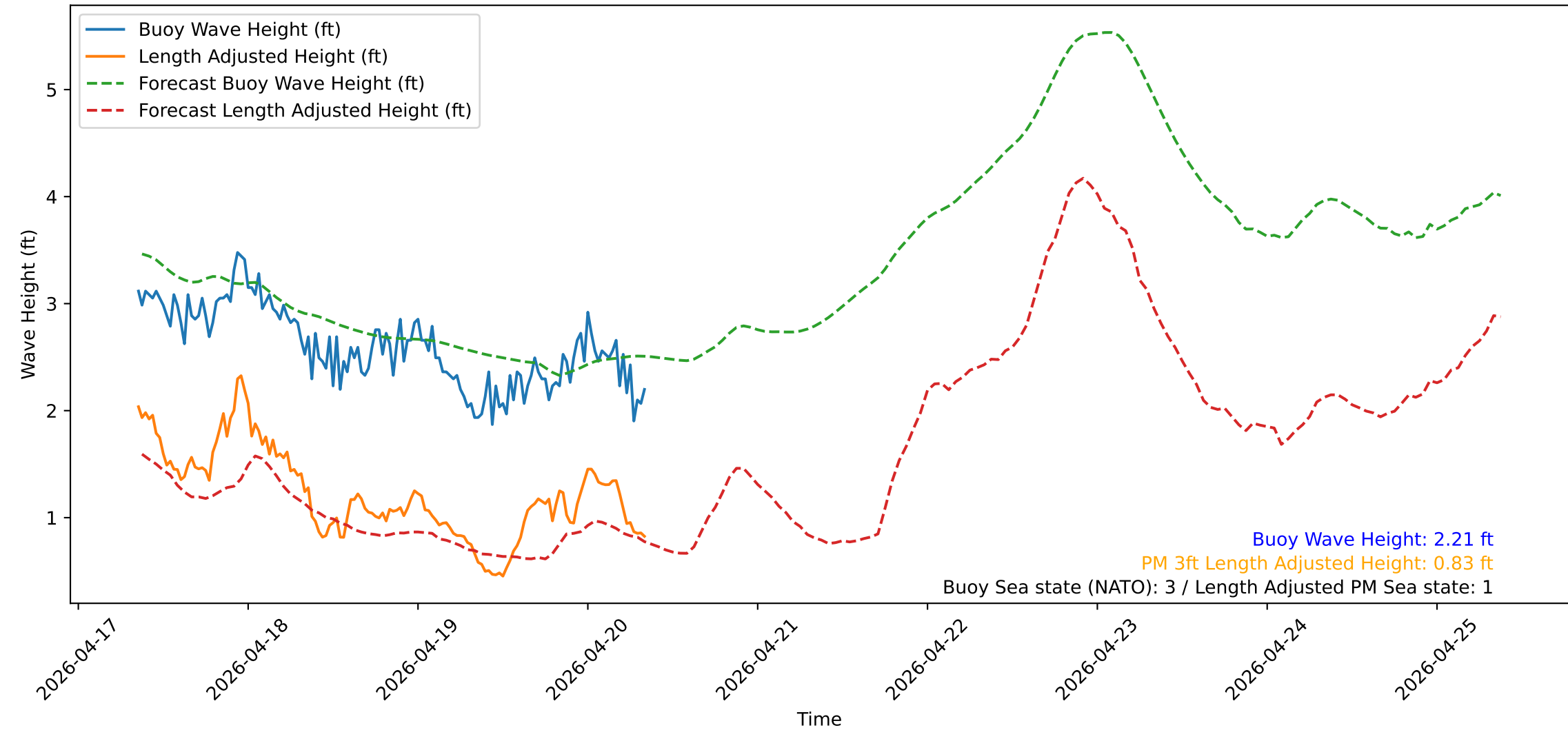
Wave Heights over Time for Green Beach at 2026-04-20 08:41:13
