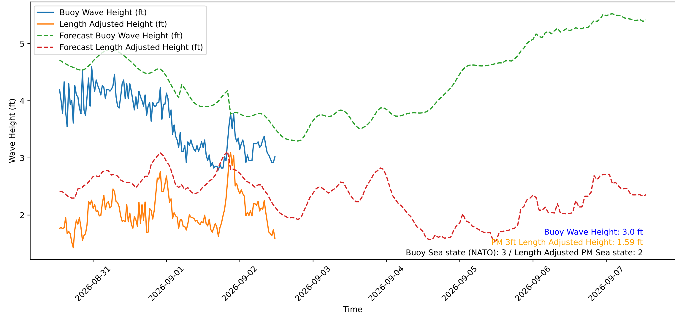
Wave Heights over Time for Green Beach at 2026-09-02 12:31:11
