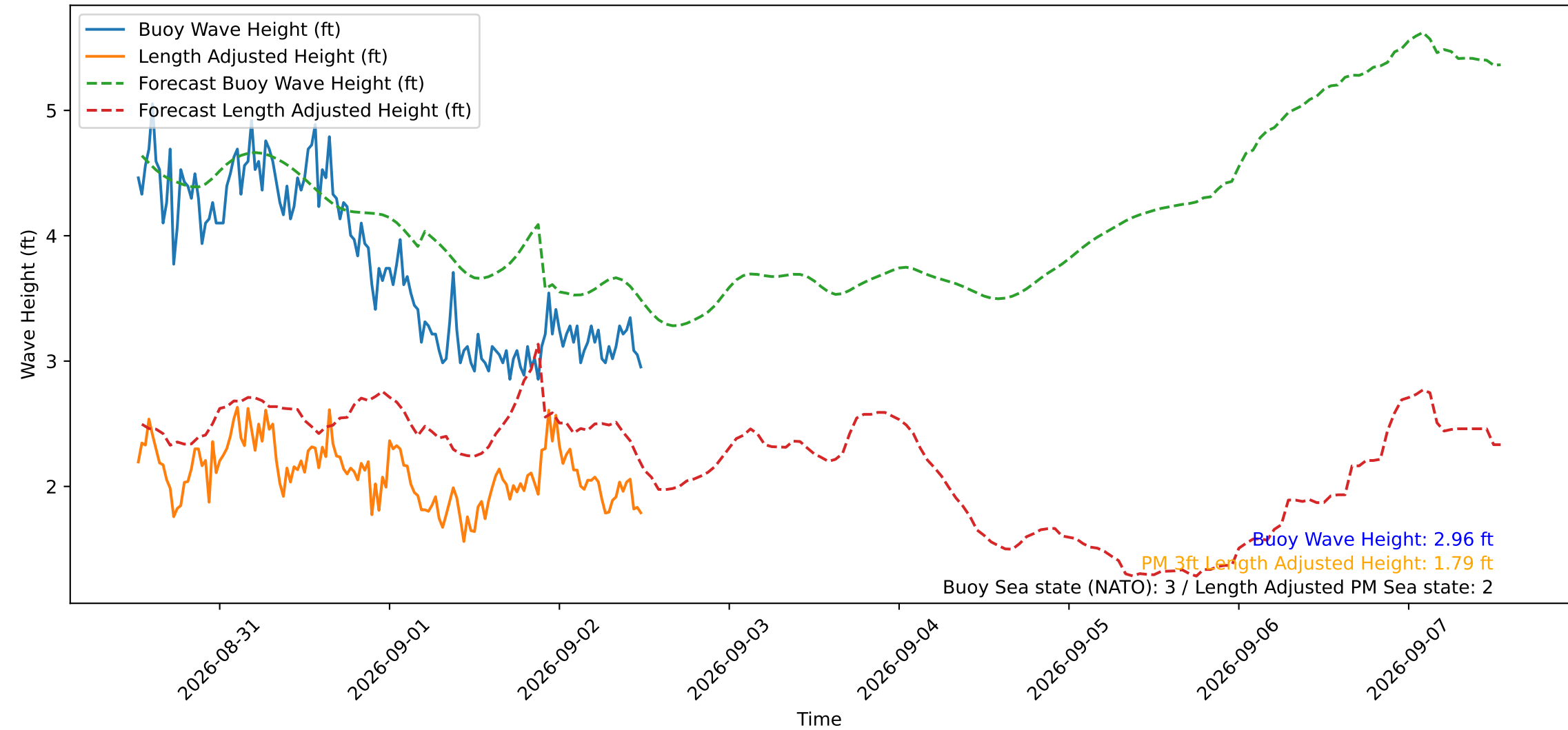
Wave Heights over Time for Oceanside Harbor at 2026-09-02 12:30:29
