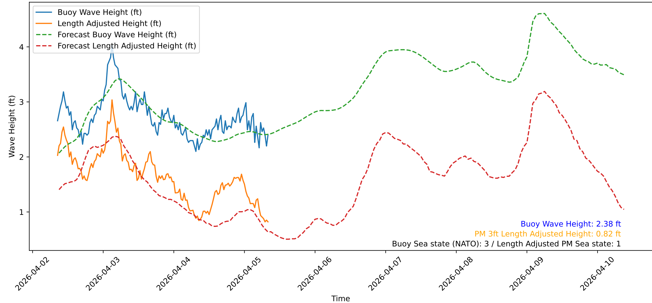
Wave Heights over Time for Oceanside Harbor at 2026-04-05 08:40:31
