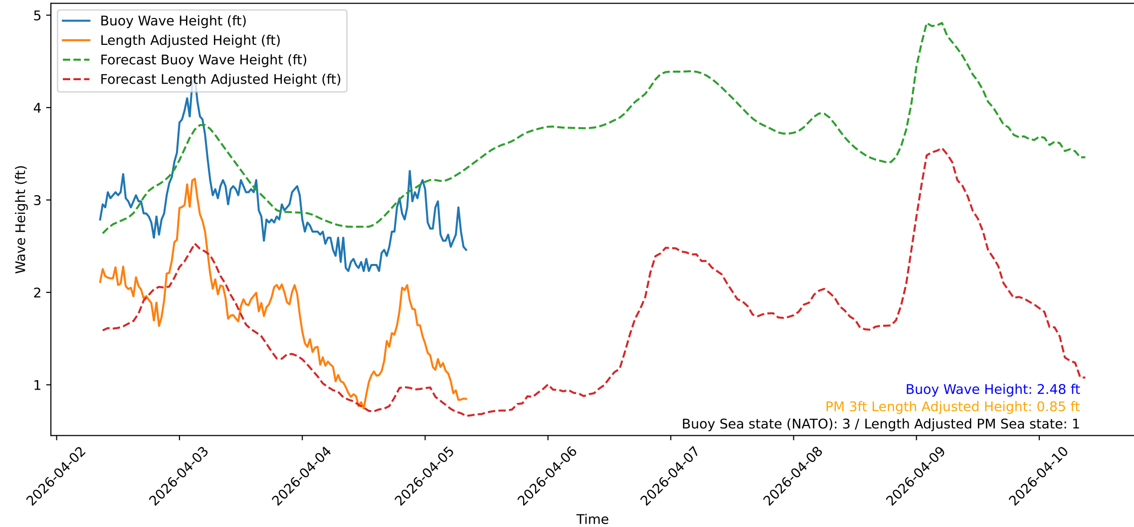
Wave Heights over Time for Green Beach at 2026-04-05 08:41:10
