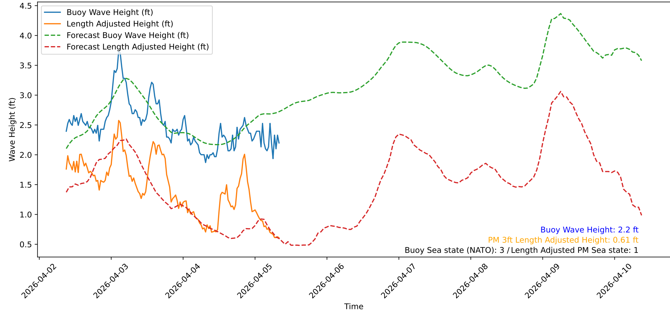
Wave Heights over Time for Red Beach at 2026-04-05 08:40:47
