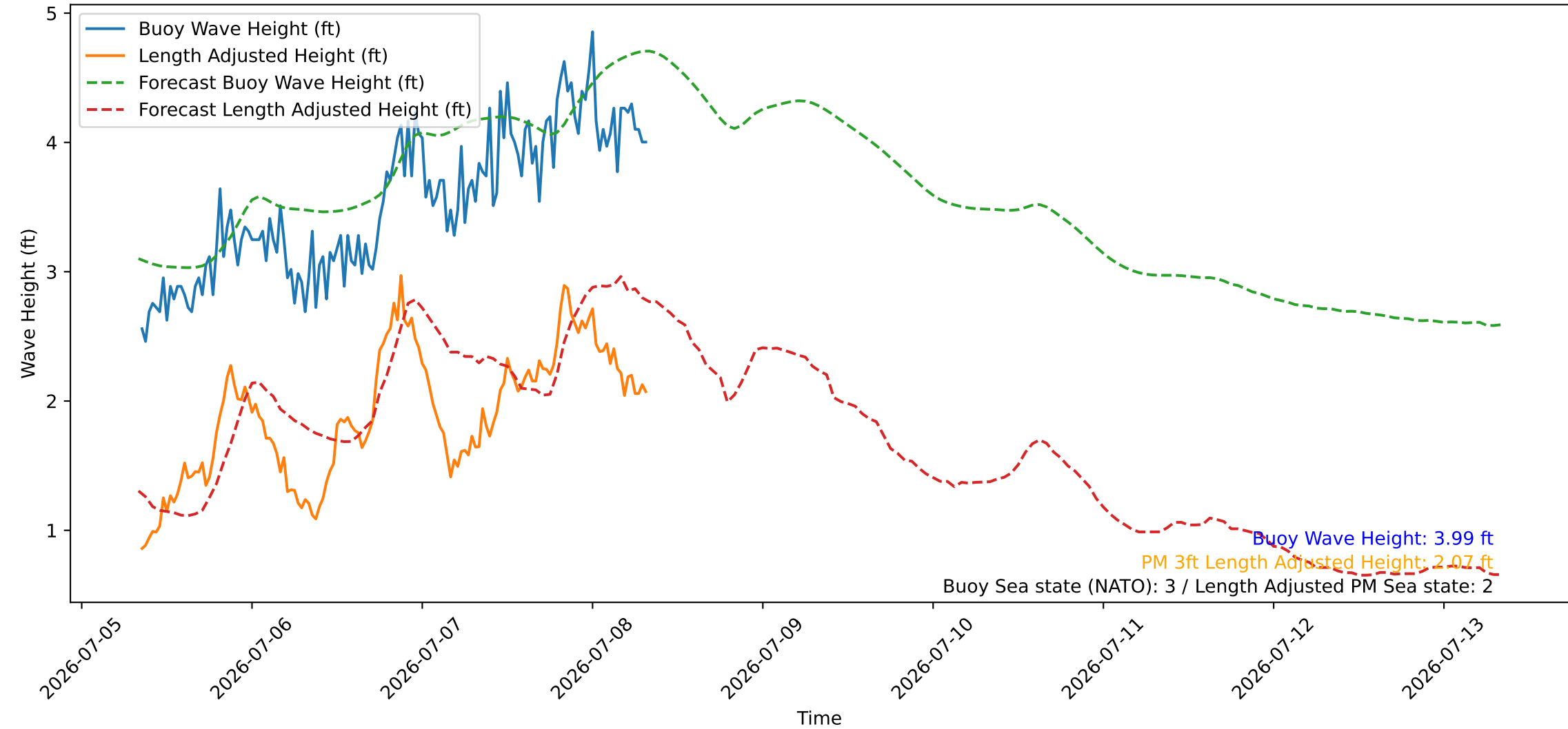
Wave Heights over Time for Red Beach at 2026-07-08 08:20:47
