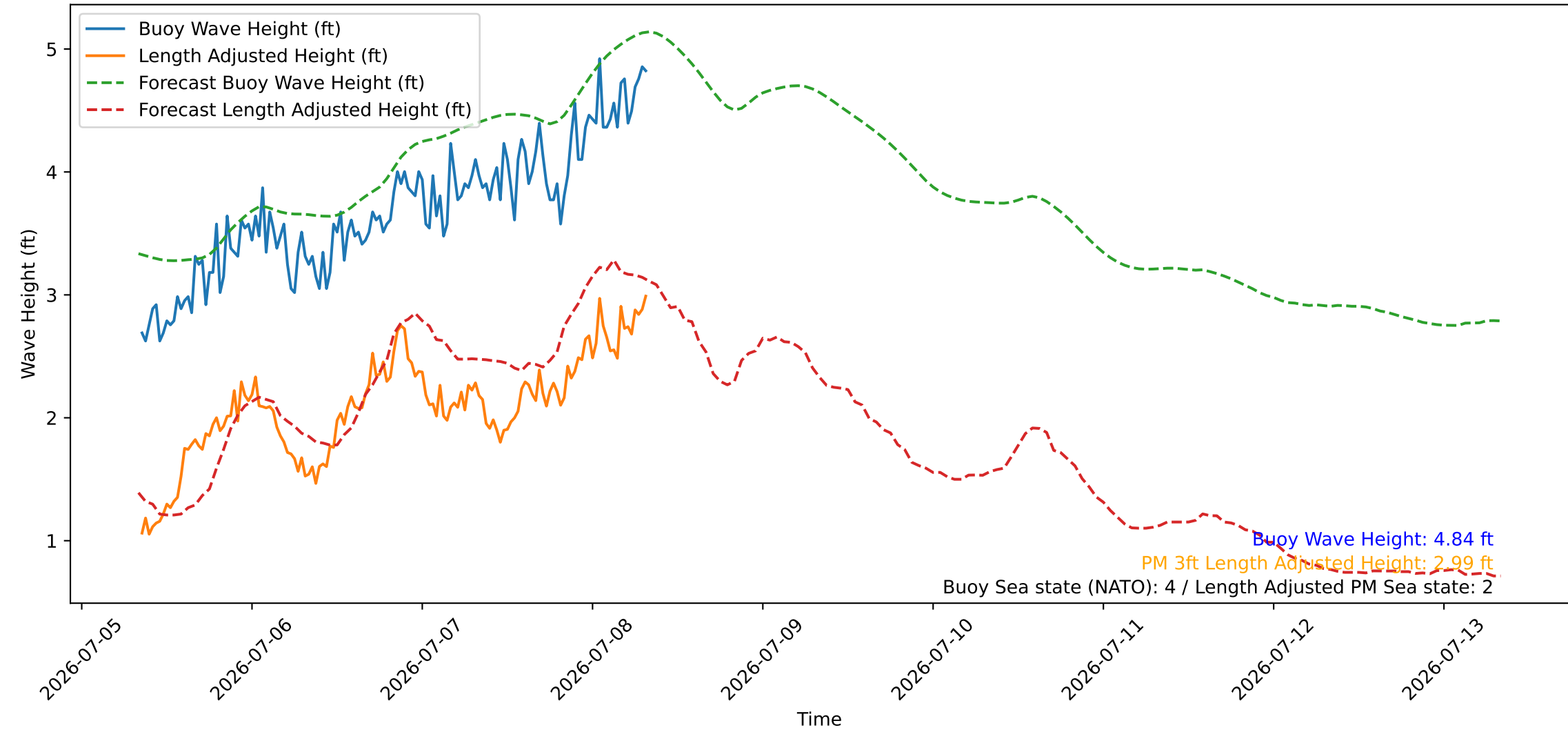
Wave Heights over Time for Oceanside Harbor at 2026-07-08 08:20:26
