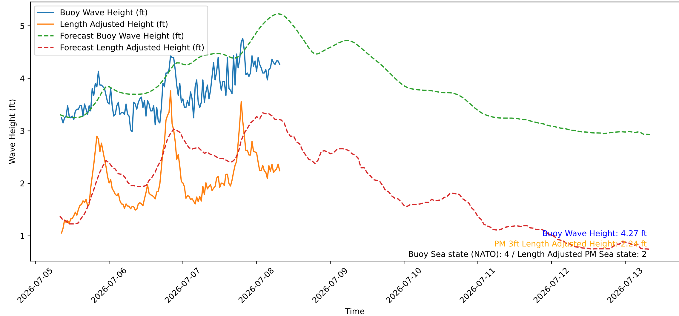
Wave Heights over Time for Green Beach at 2026-07-08 08:21:10
