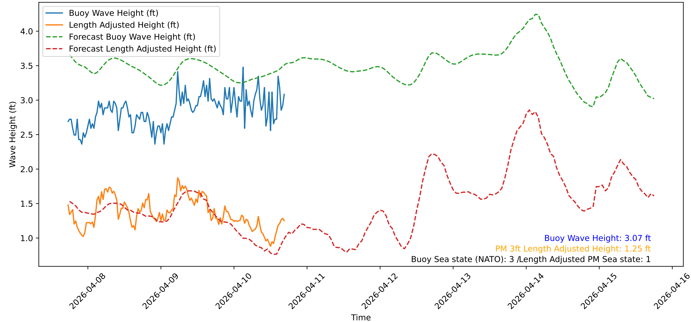
Wave Heights over Time for Green Beach at 2026-04-10 17:31:13
