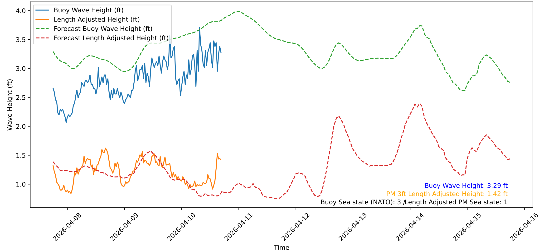
Wave Heights over Time for Red Beach at 2026-04-10 17:30:51
