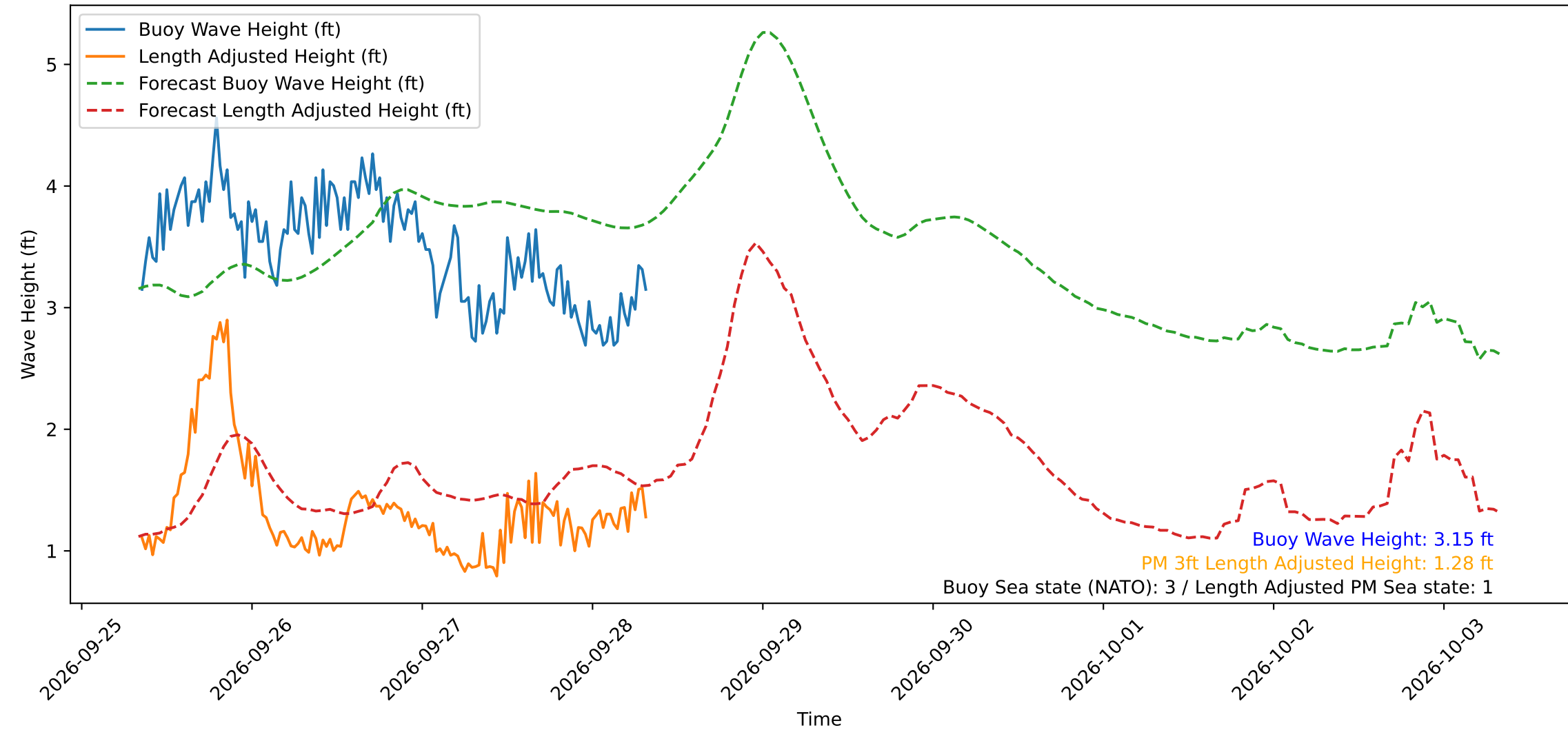
Wave Heights over Time for Green Beach at 2026-09-28 08:11:11
