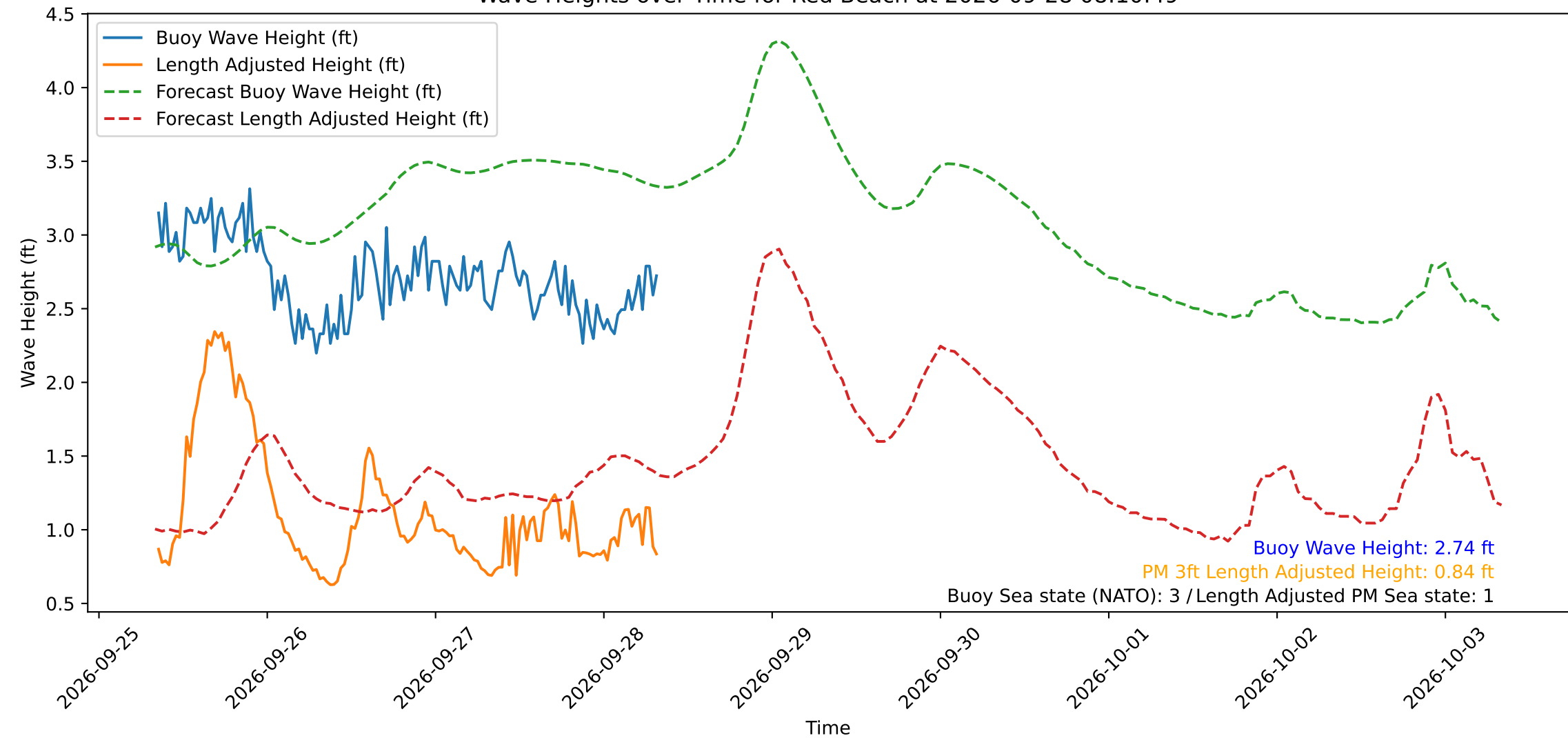
Wave Heights over Time for Red Beach at 2026-09-28 08:10:49
