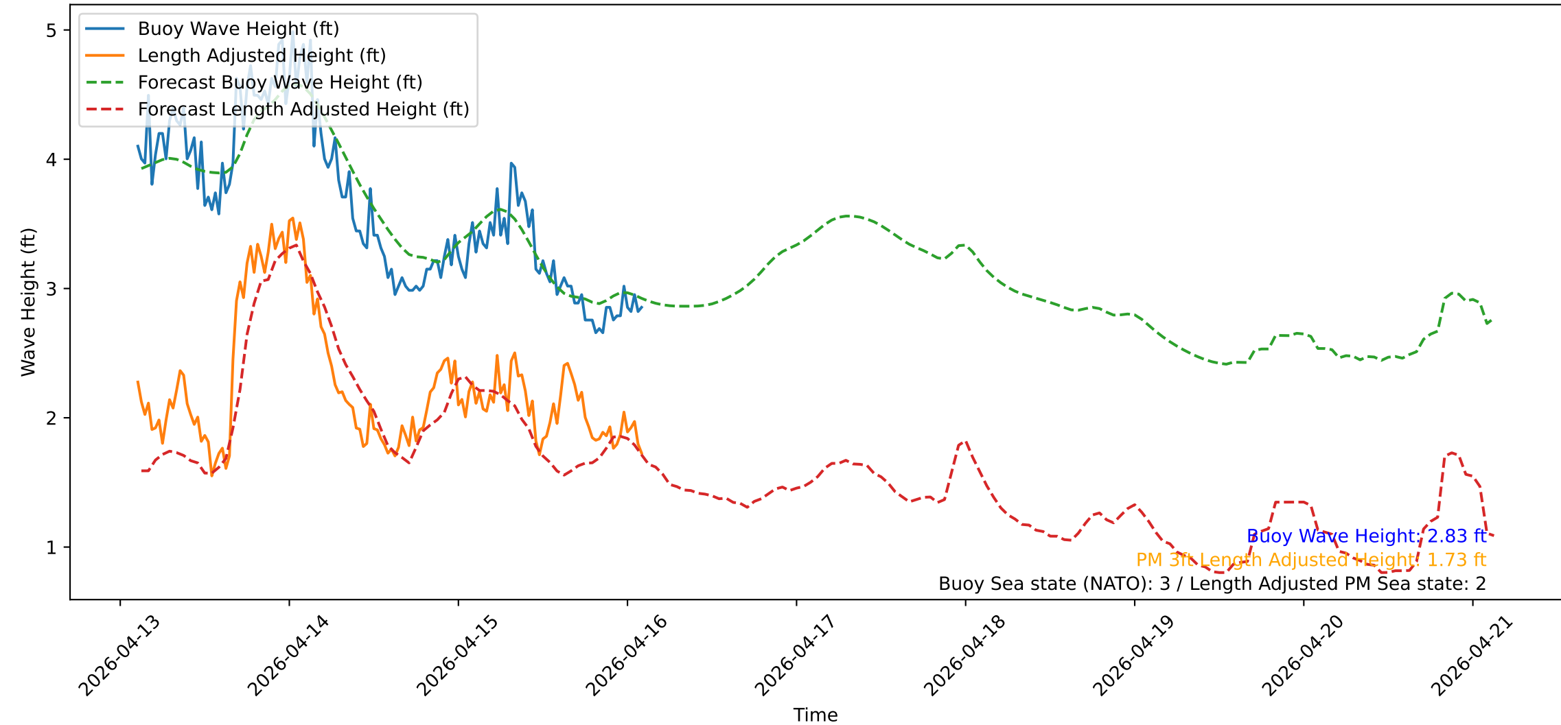
Wave Heights over Time for Green Beach at 2026-04-16 02:41:13
