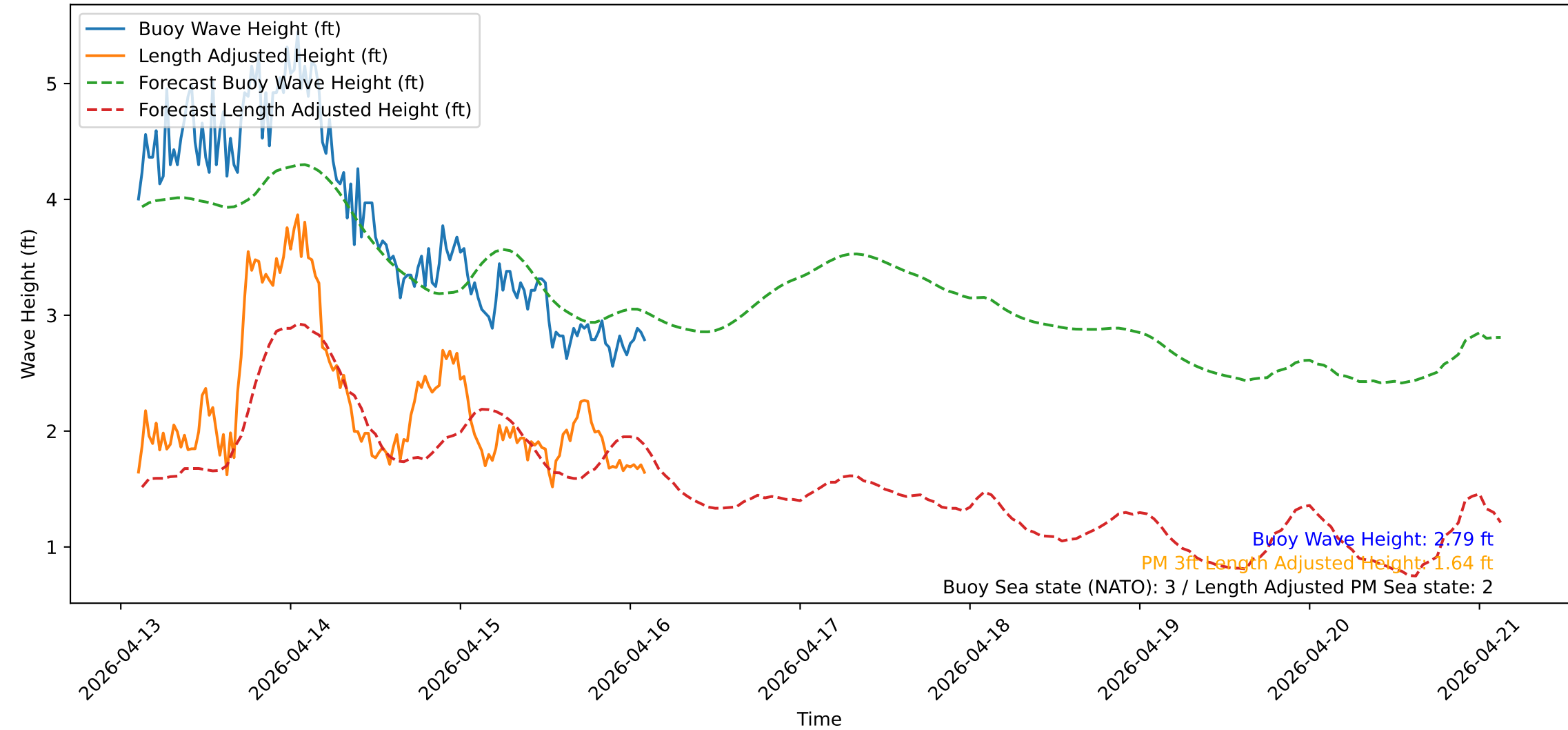
Wave Heights over Time for Oceanside Harbor at 2026-04-16 02:40:31
