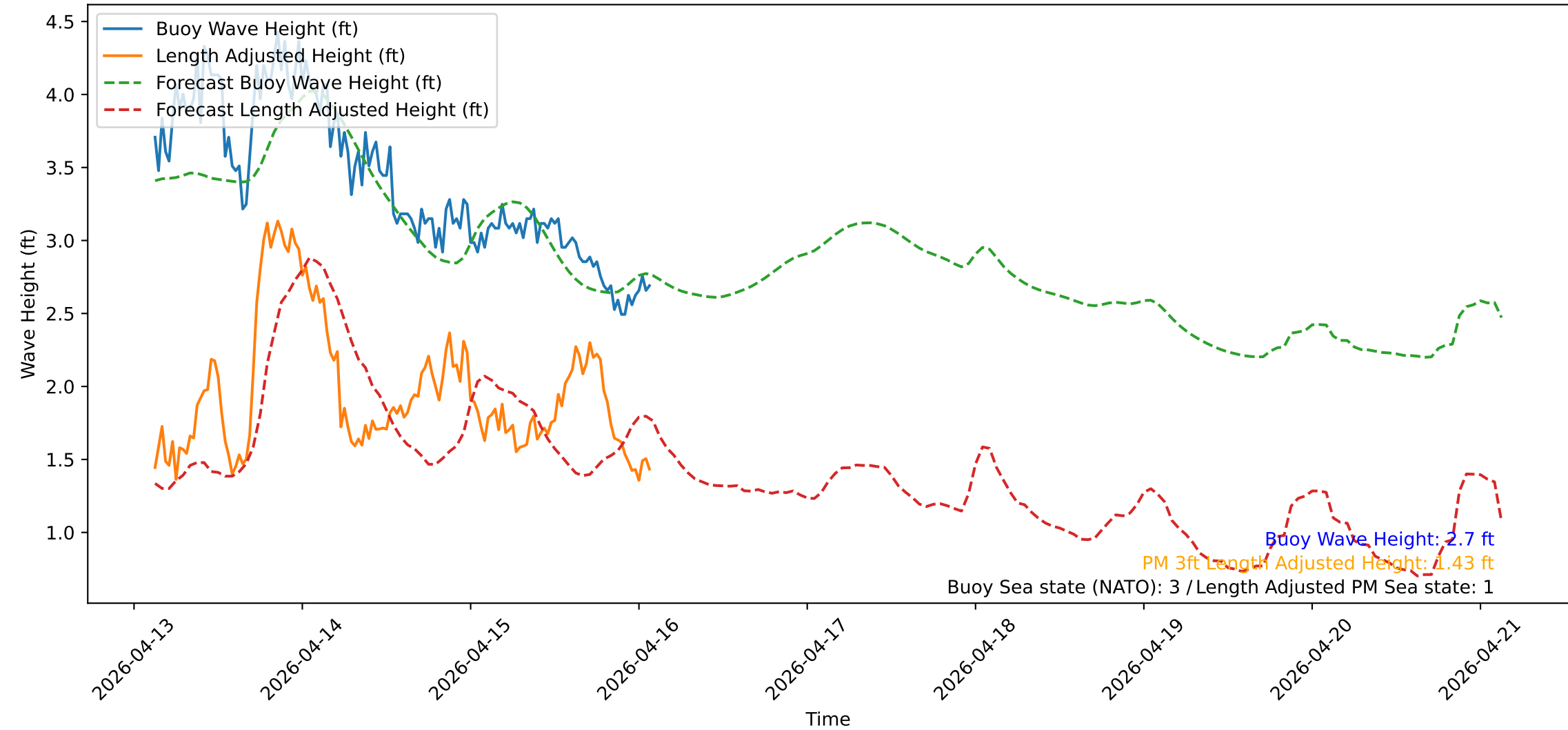
Wave Heights over Time for Red Beach at 2026-04-16 02:40:51
