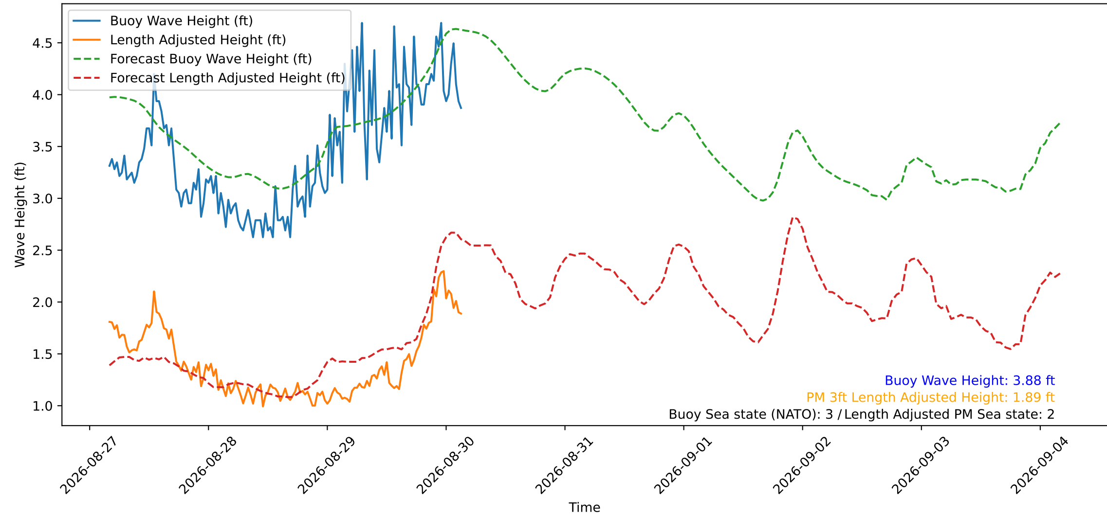
Wave Heights over Time for Red Beach at 2026-08-30 03:50:51
