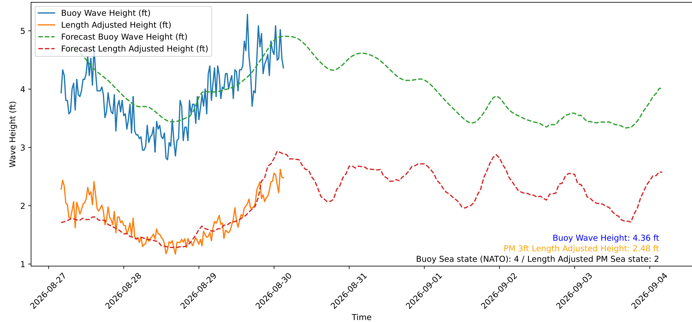
Wave Heights over Time for Oceanside Harbor at 2026-08-30 03:50:30
