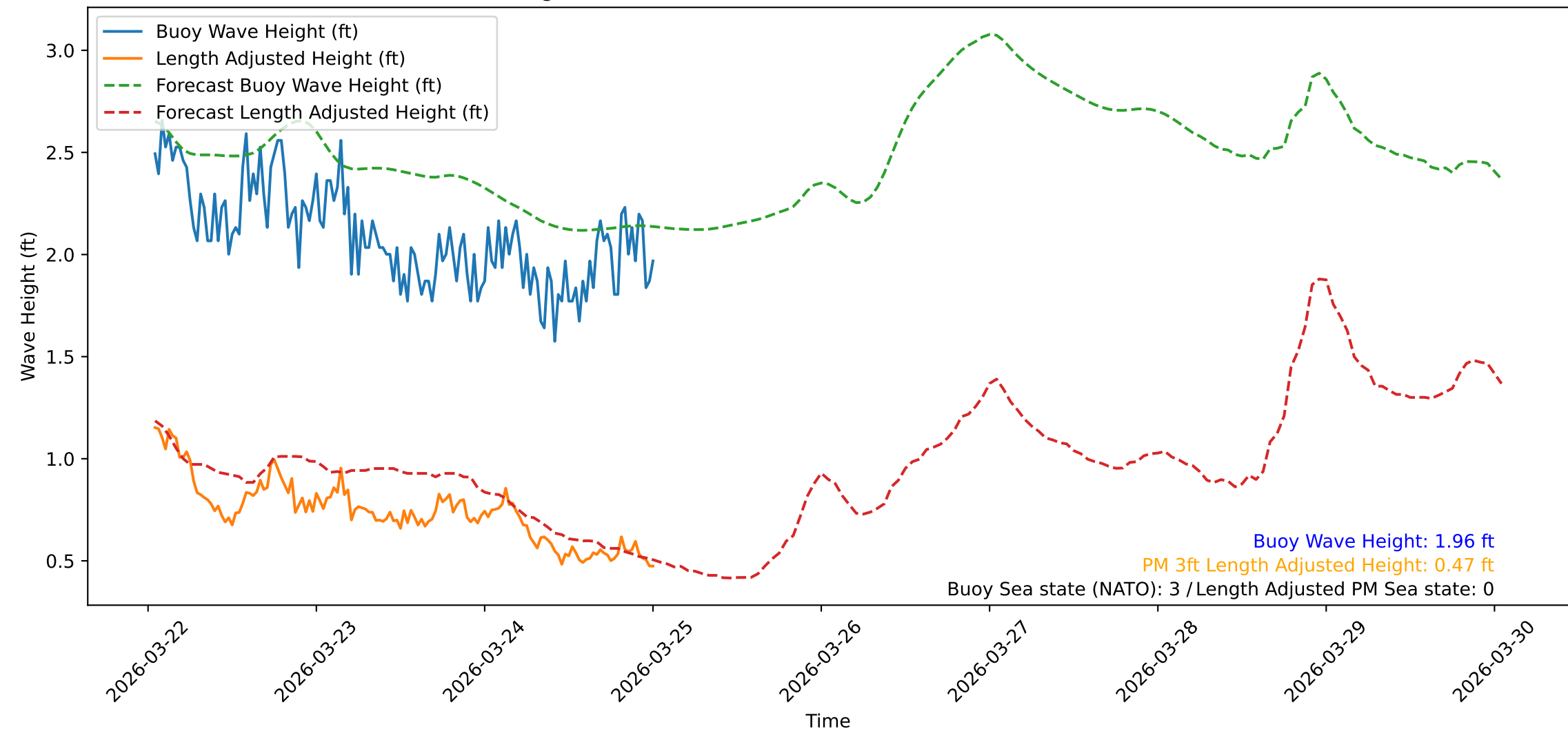
Wave Heights over Time for Oceanside Harbor at 2026-03-25 00:50:31
