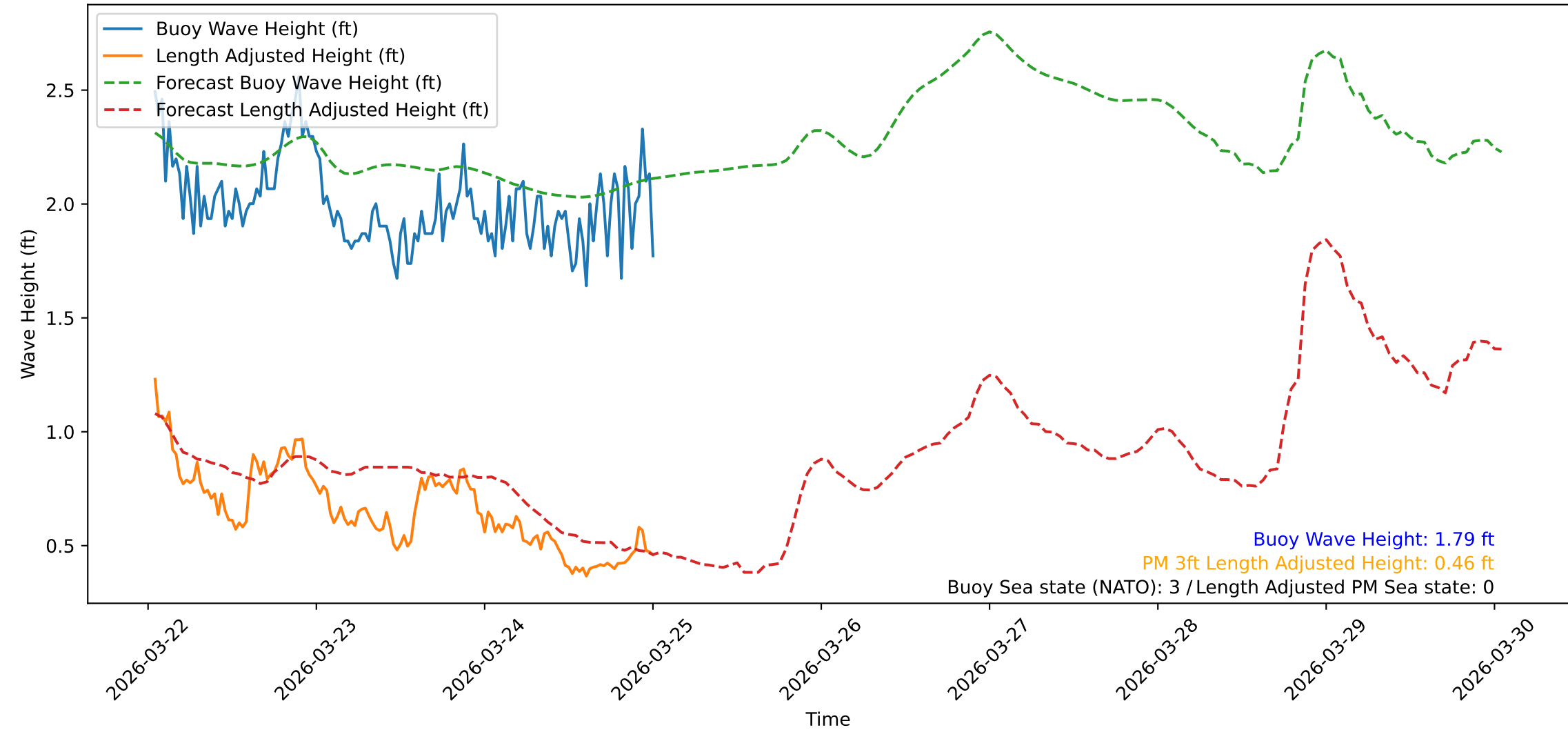
Wave Heights over Time for Red Beach at 2026-03-25 00:50:48
