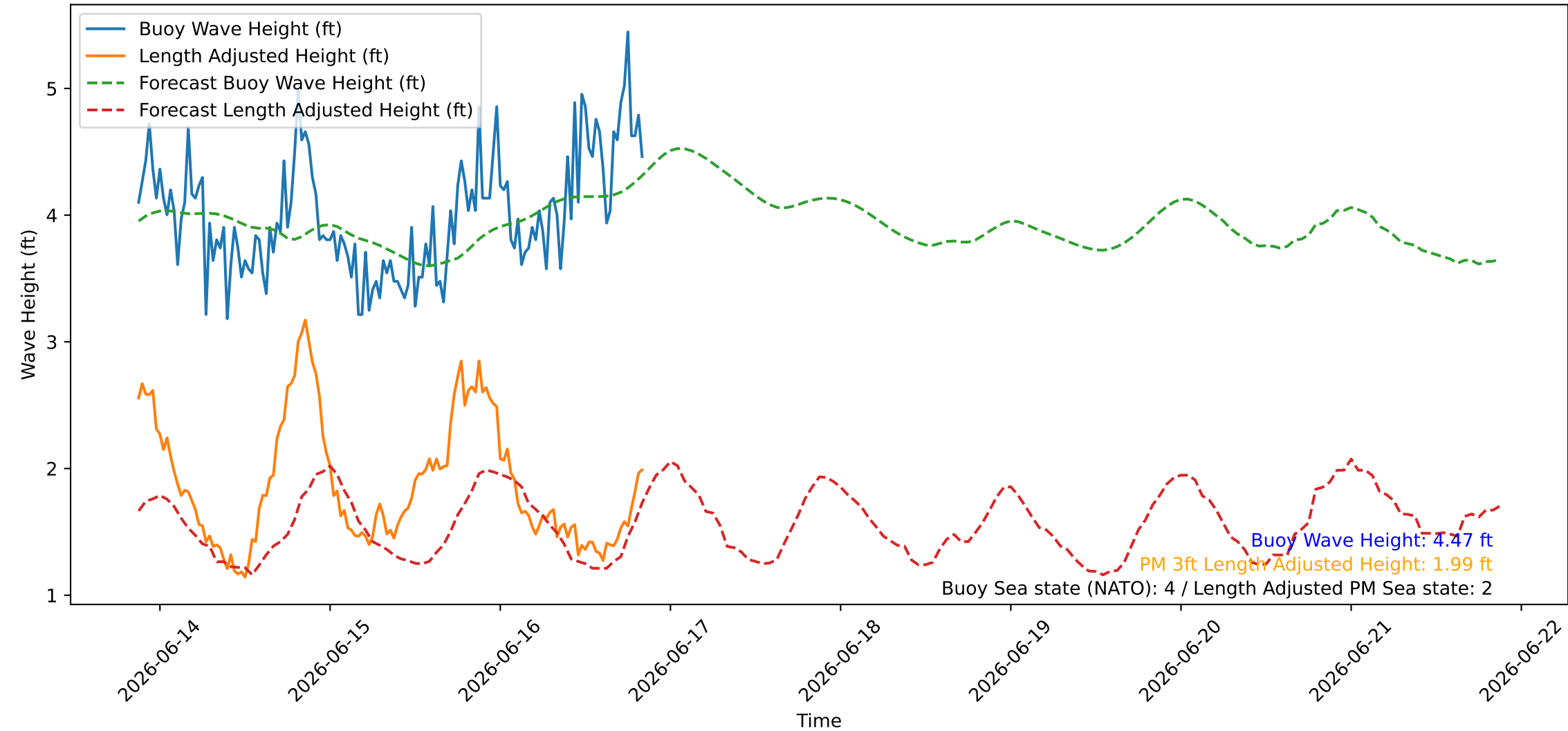
Wave Heights over Time for Oceanside Harbor at 2026-06-16 21:00:26
