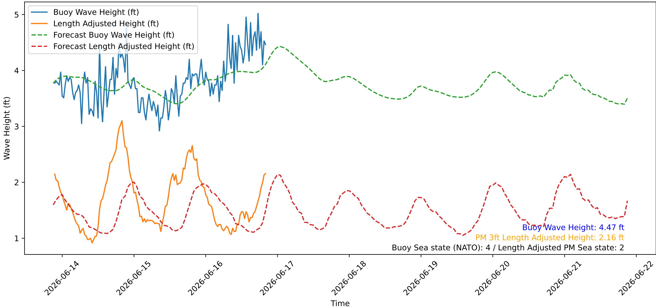
Wave Heights over Time for Red Beach at 2026-06-16 21:00:45
