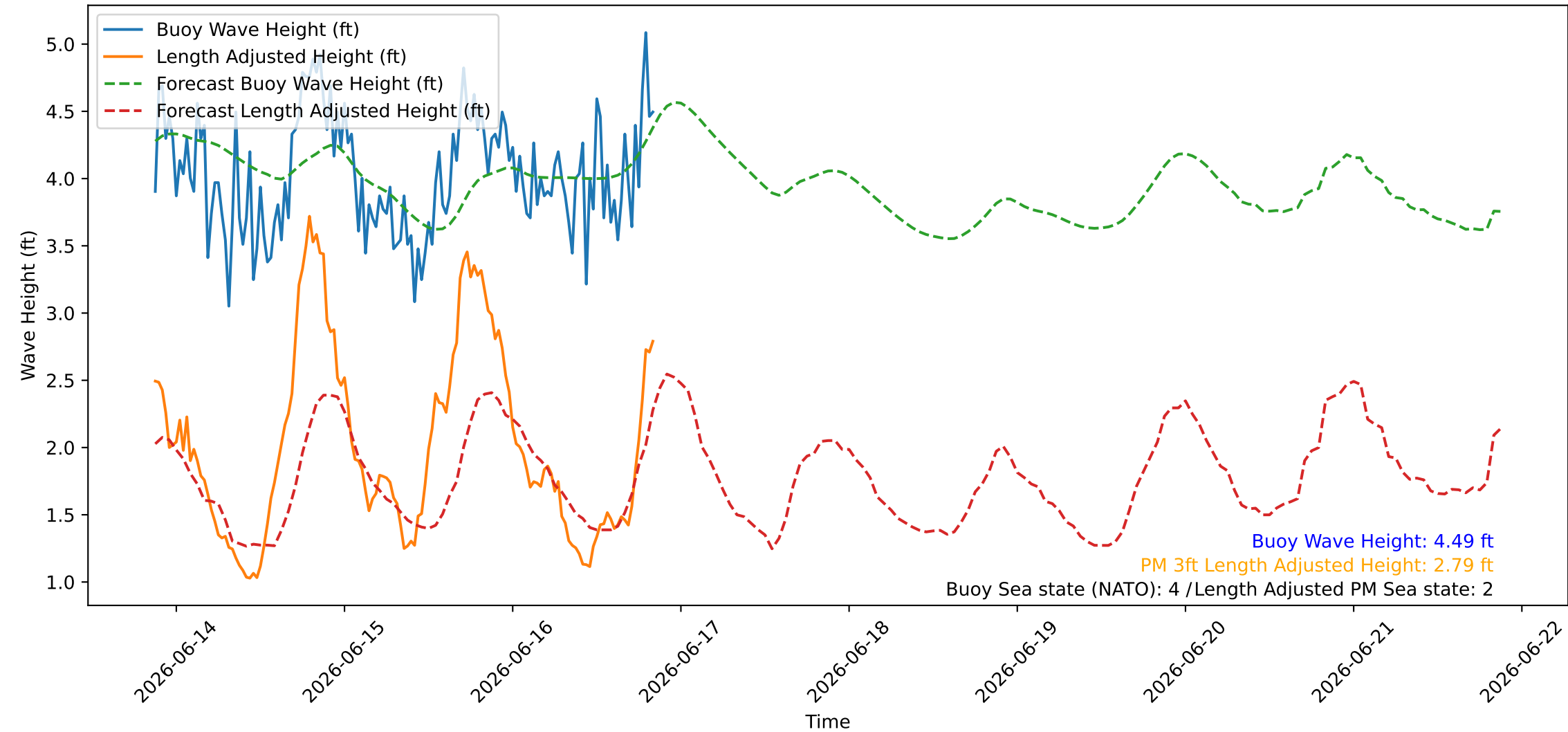
Wave Heights over Time for Green Beach at 2026-06-16 21:01:08
