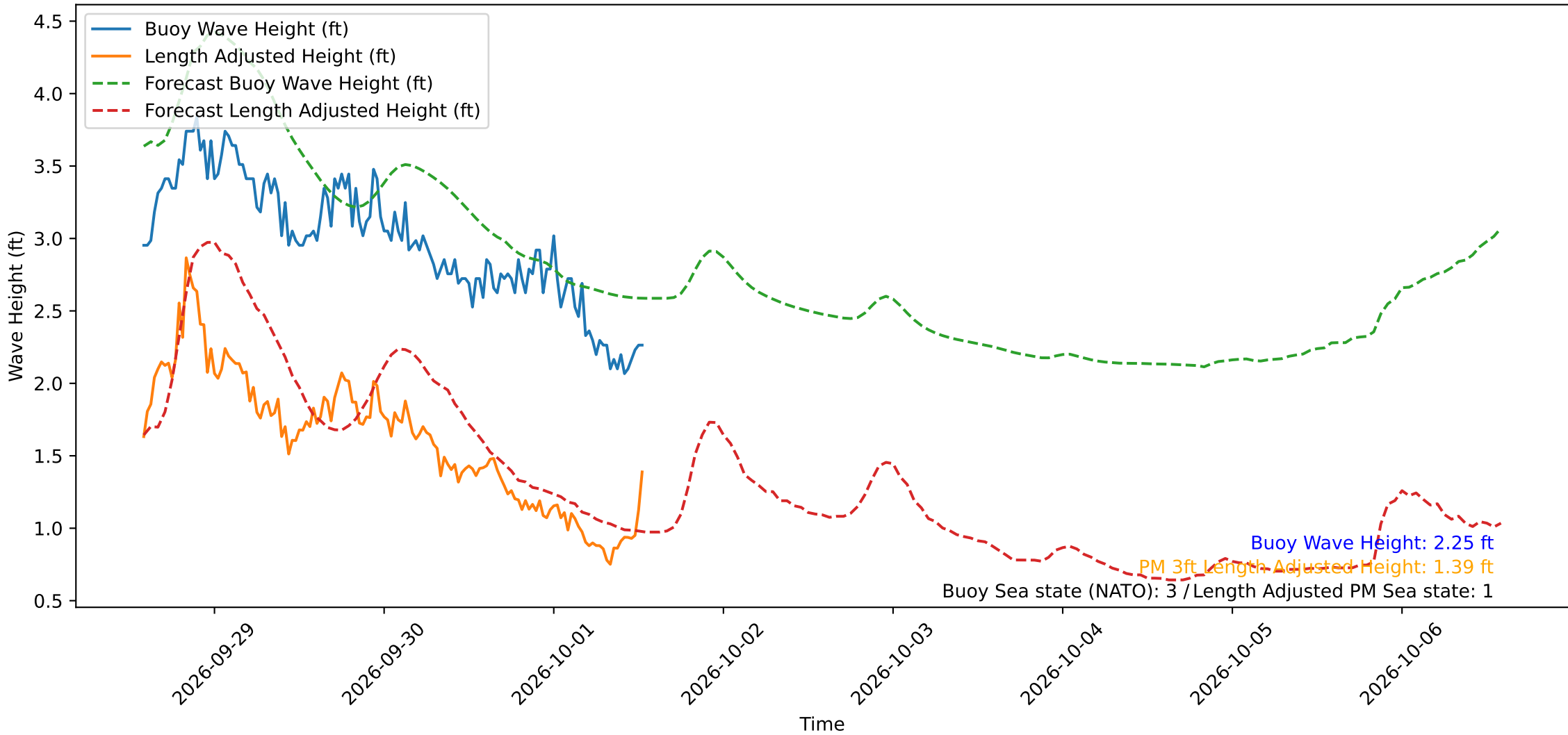
Wave Heights over Time for Red Beach at 2026-10-01 13:30:49
