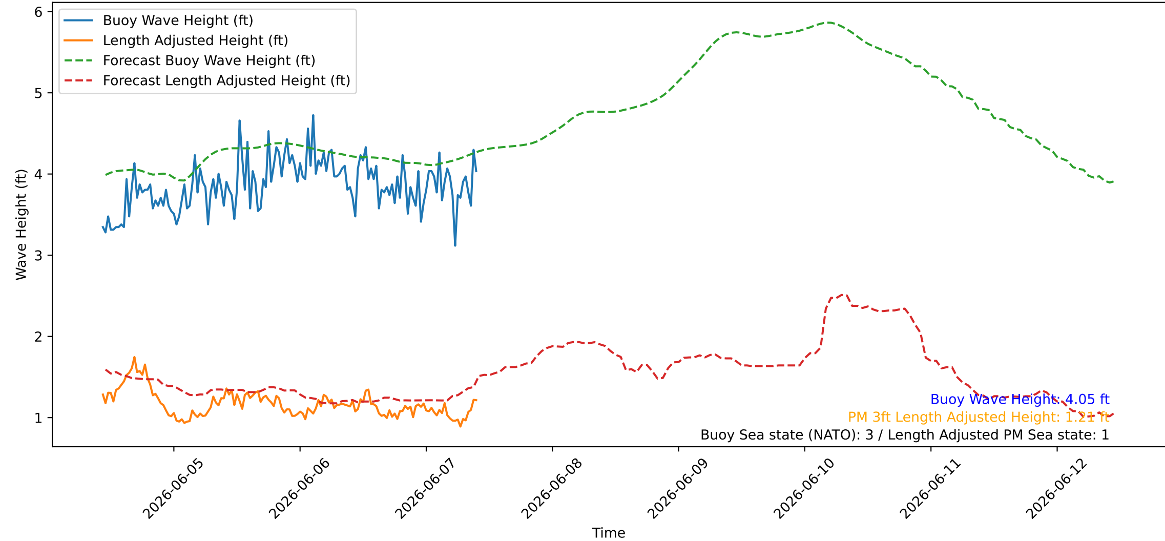
Wave Heights over Time for Green Beach at 2026-06-07 10:31:07
