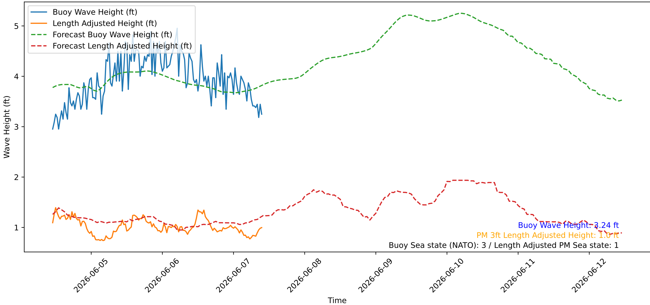
Wave Heights over Time for Red Beach at 2026-06-07 10:30:45
