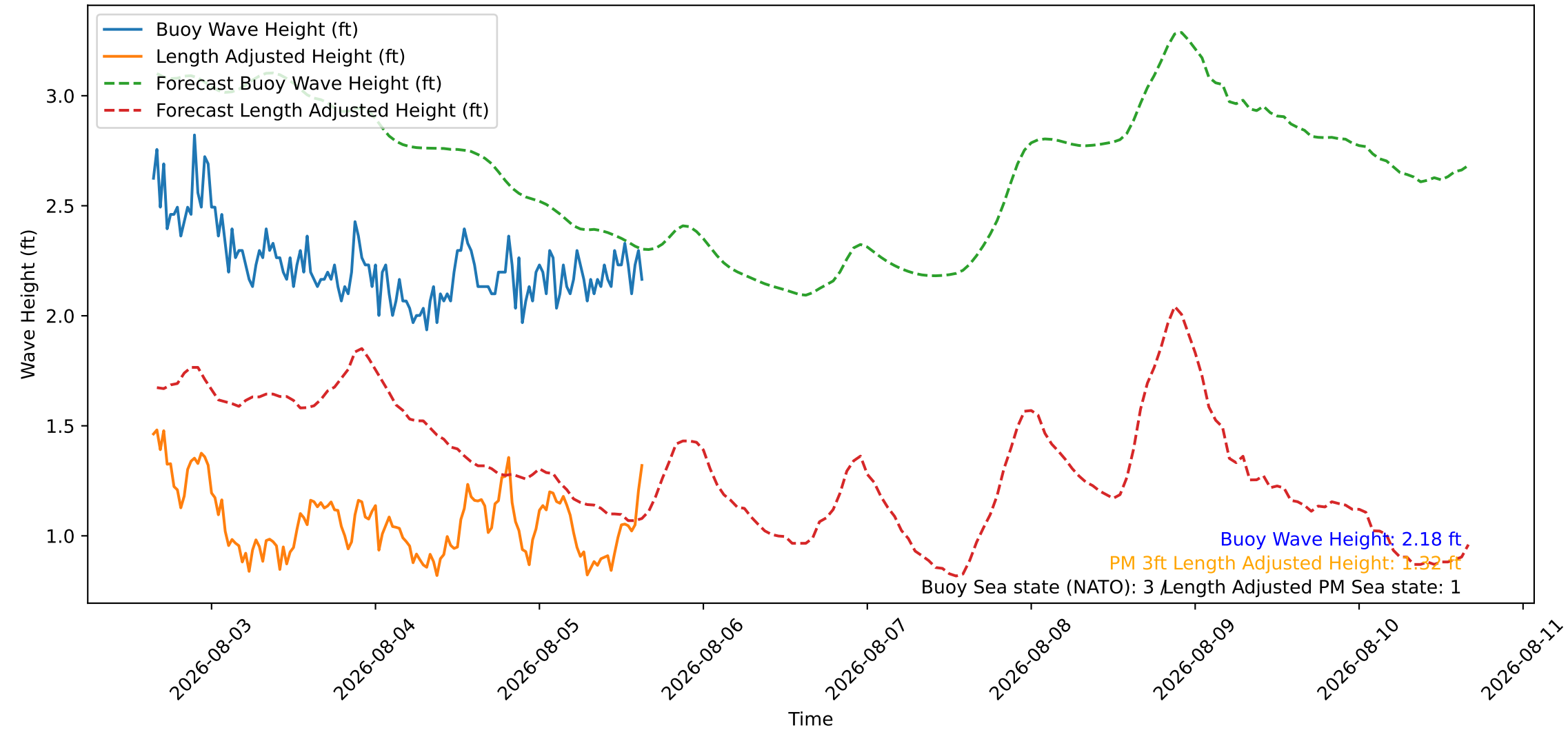
Wave Heights over Time for Green Beach at 2026-08-05 15:41:09
