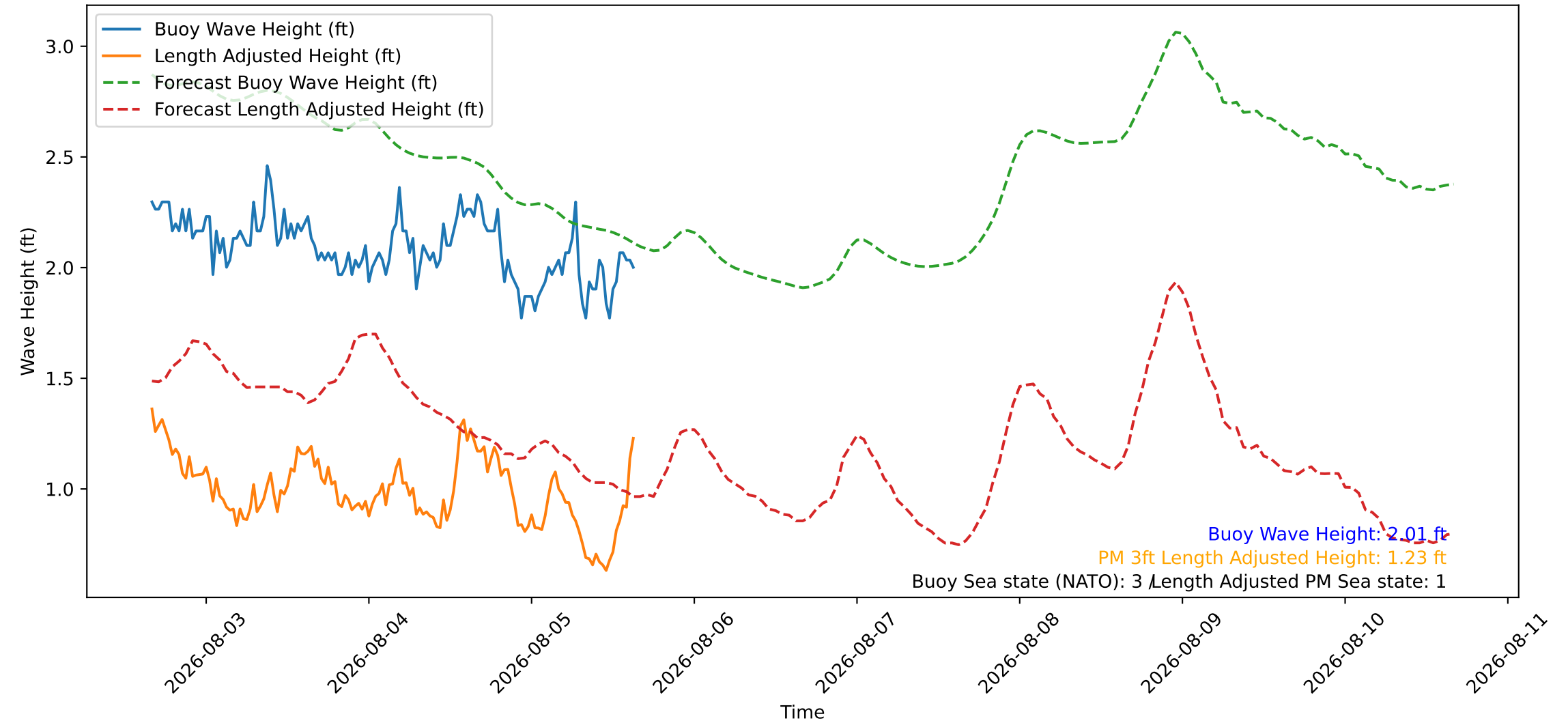
Wave Heights over Time for Red Beach at 2026-08-05 15:40:46
