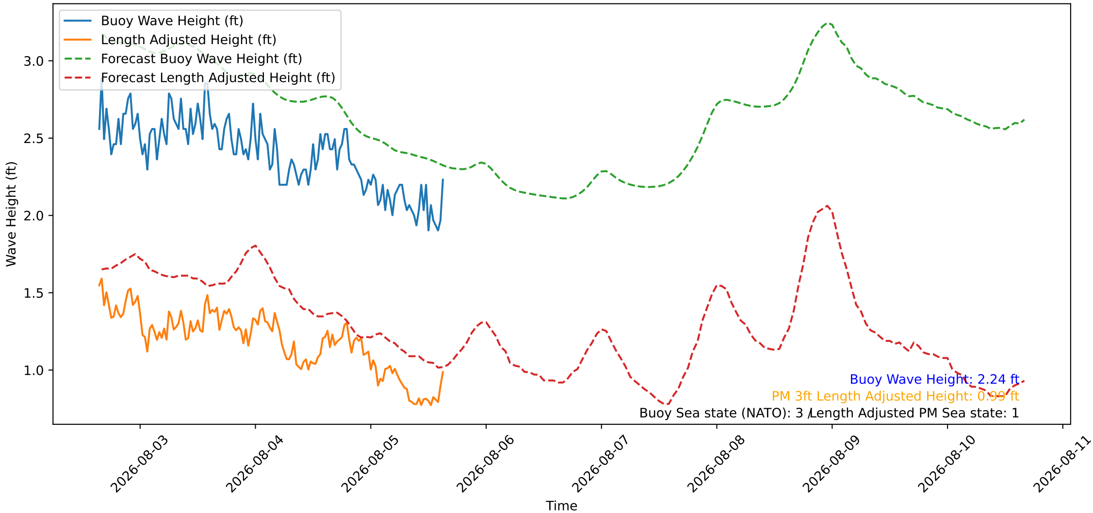
Wave Heights over Time for Oceanside Harbor at 2026-08-05 15:40:27
