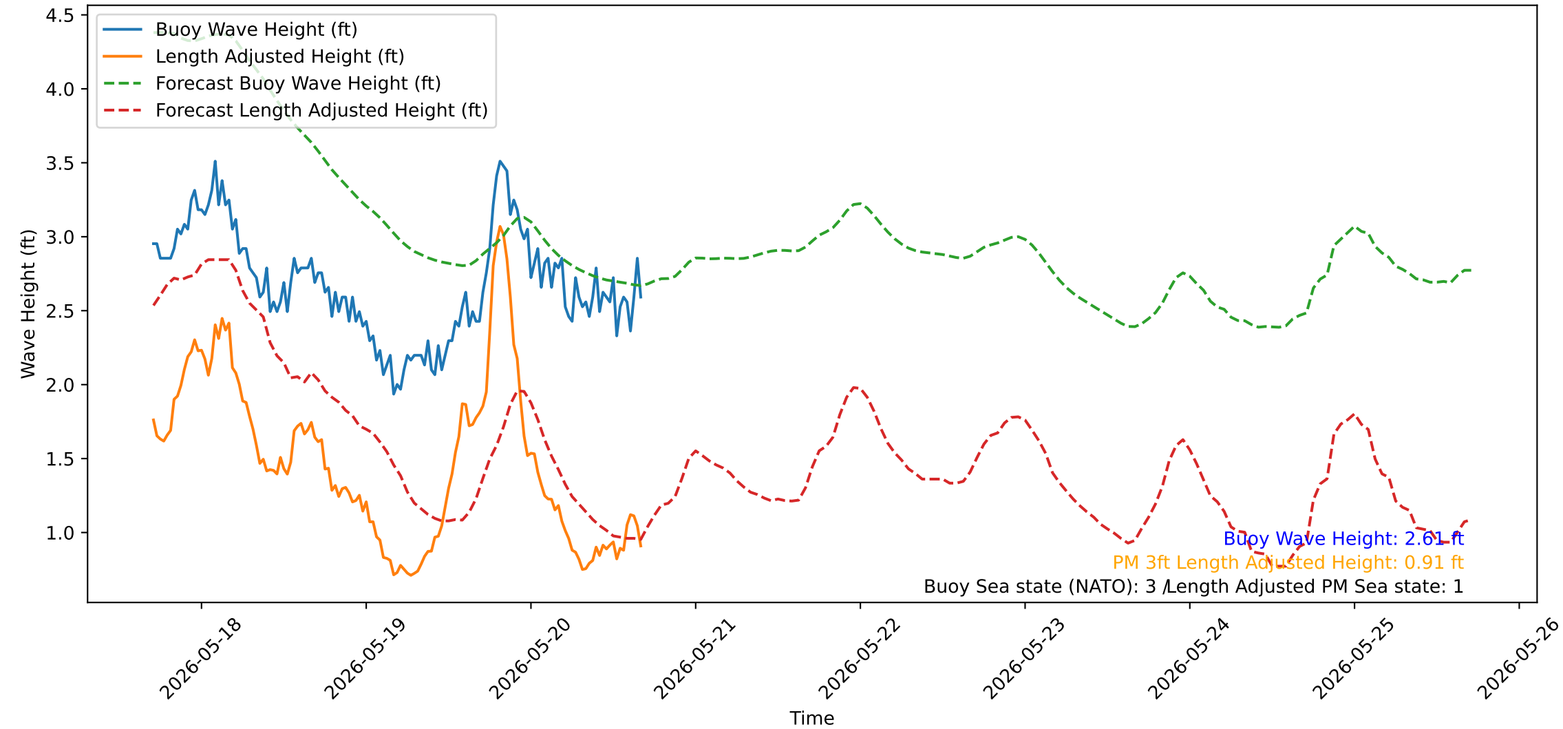
Wave Heights over Time for Red Beach at 2026-05-20 16:50:52
