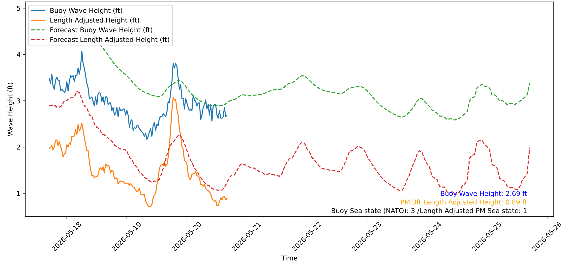
Wave Heights over Time for Green Beach at 2026-05-20 16:51:15
