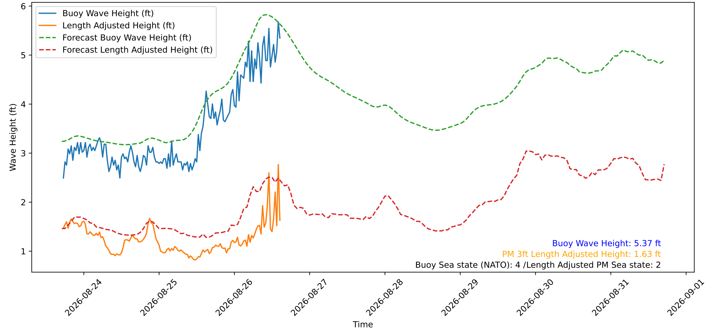
Wave Heights over Time for Green Beach at 2026-08-26 17:01:13
