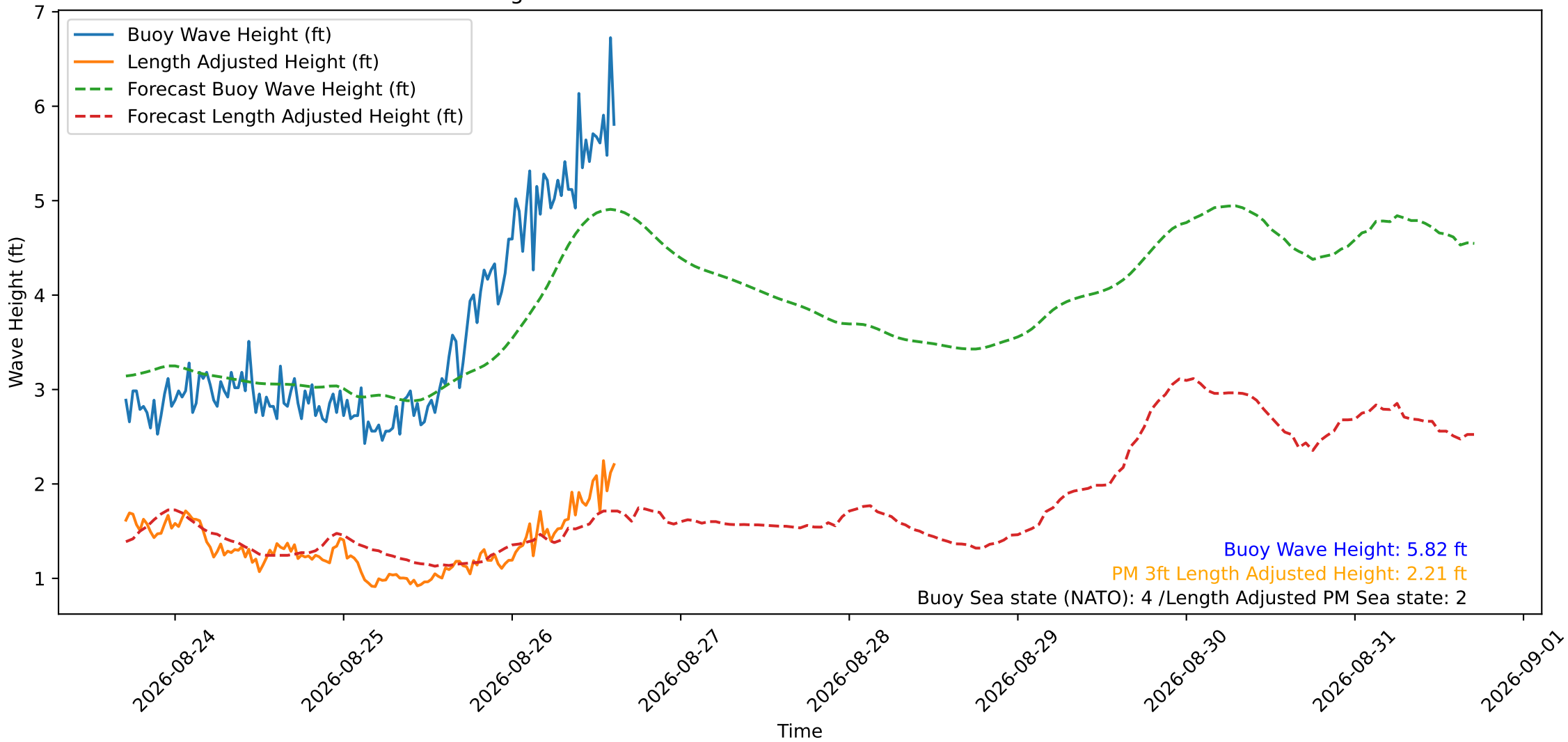
Wave Heights over Time for Oceanside Harbor at 2026-08-26 17:00:29
