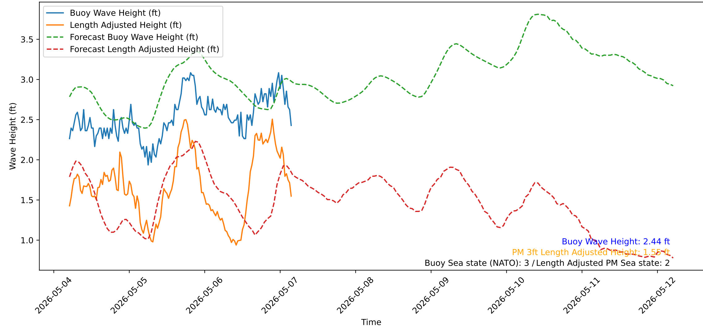
Wave Heights over Time for Red Beach at 2026-05-07 04:30:50
