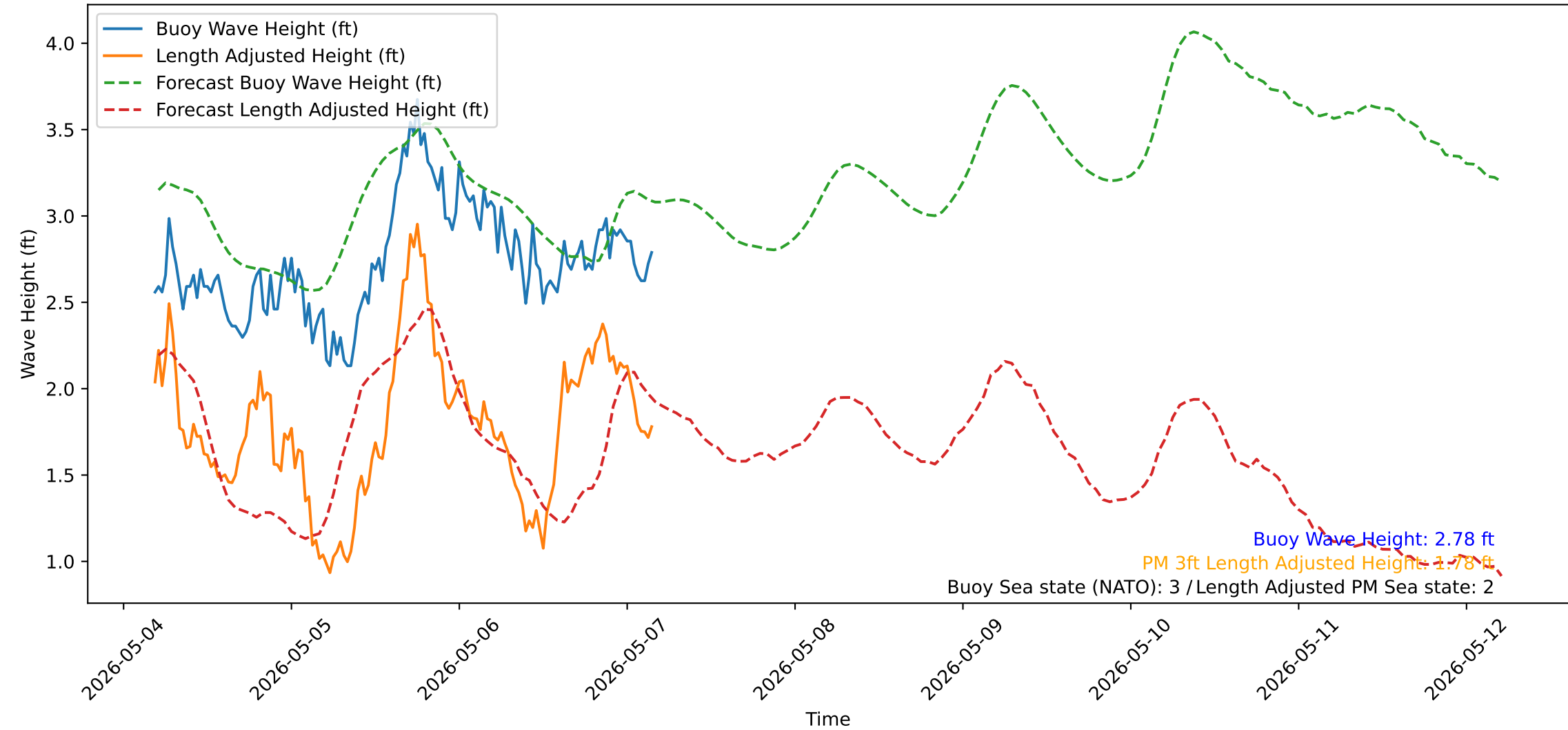
Wave Heights over Time for Green Beach at 2026-05-07 04:31:11
