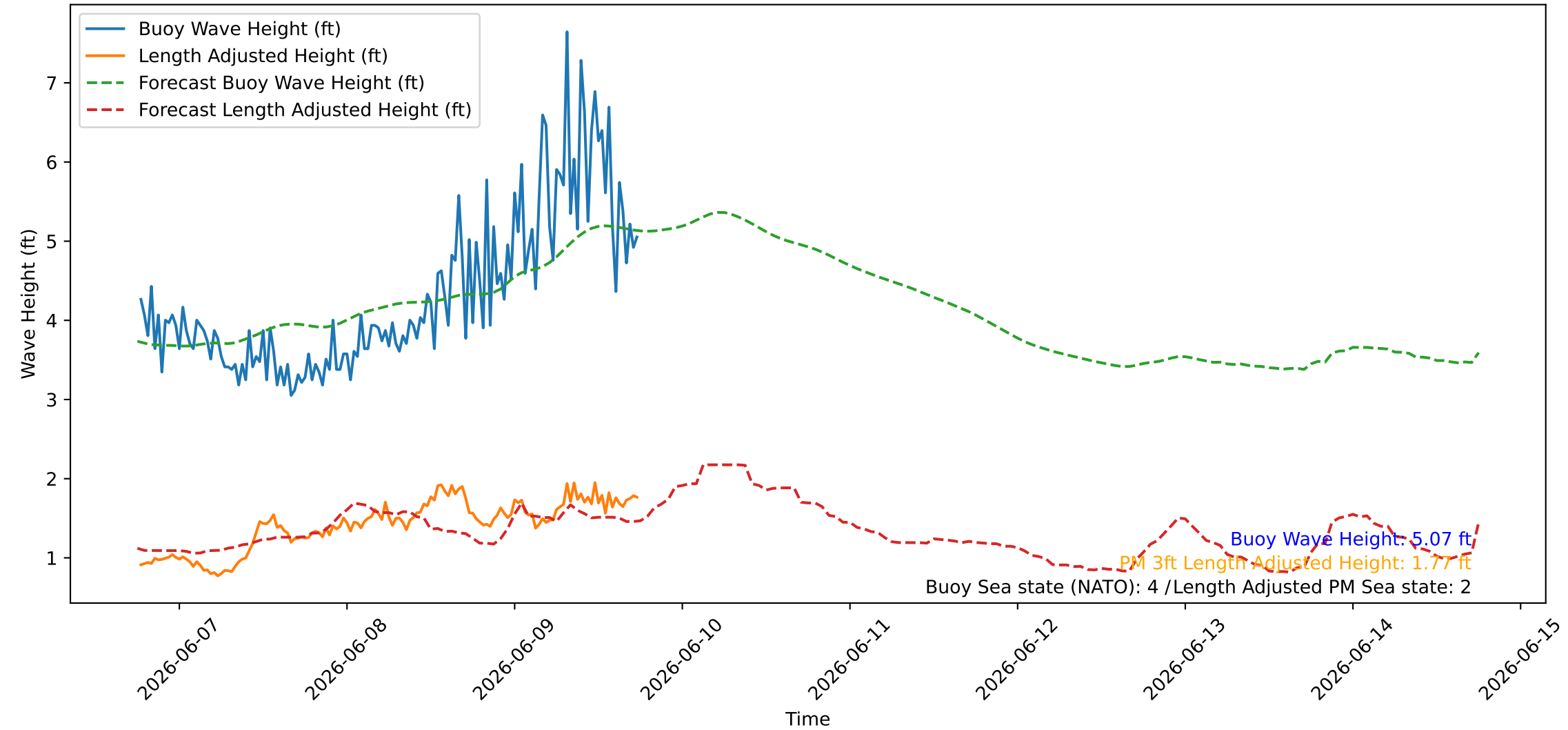
Wave Heights over Time for Red Beach at 2026-06-09 18:10:46
