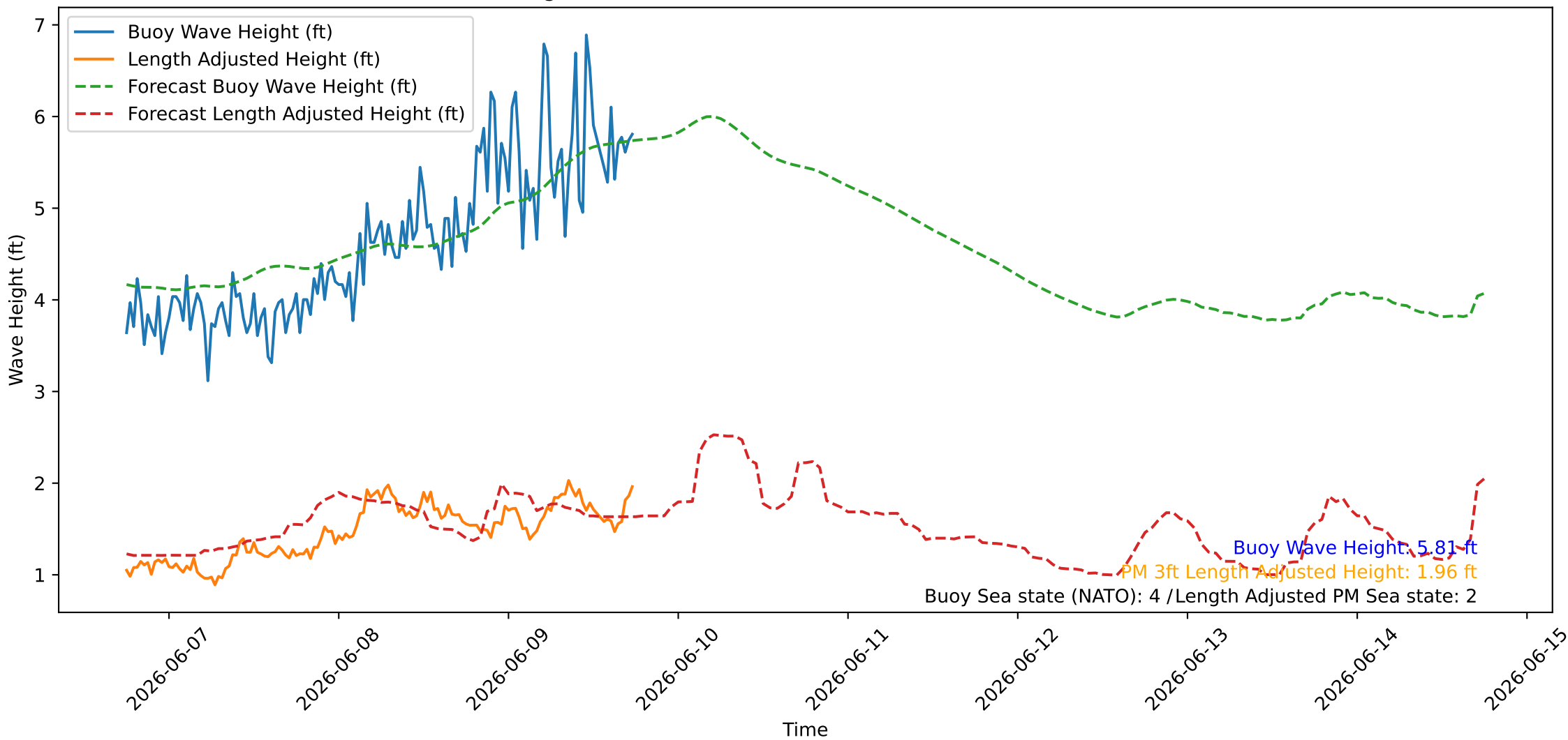
Wave Heights over Time for Green Beach at 2026-06-09 18:11:08
