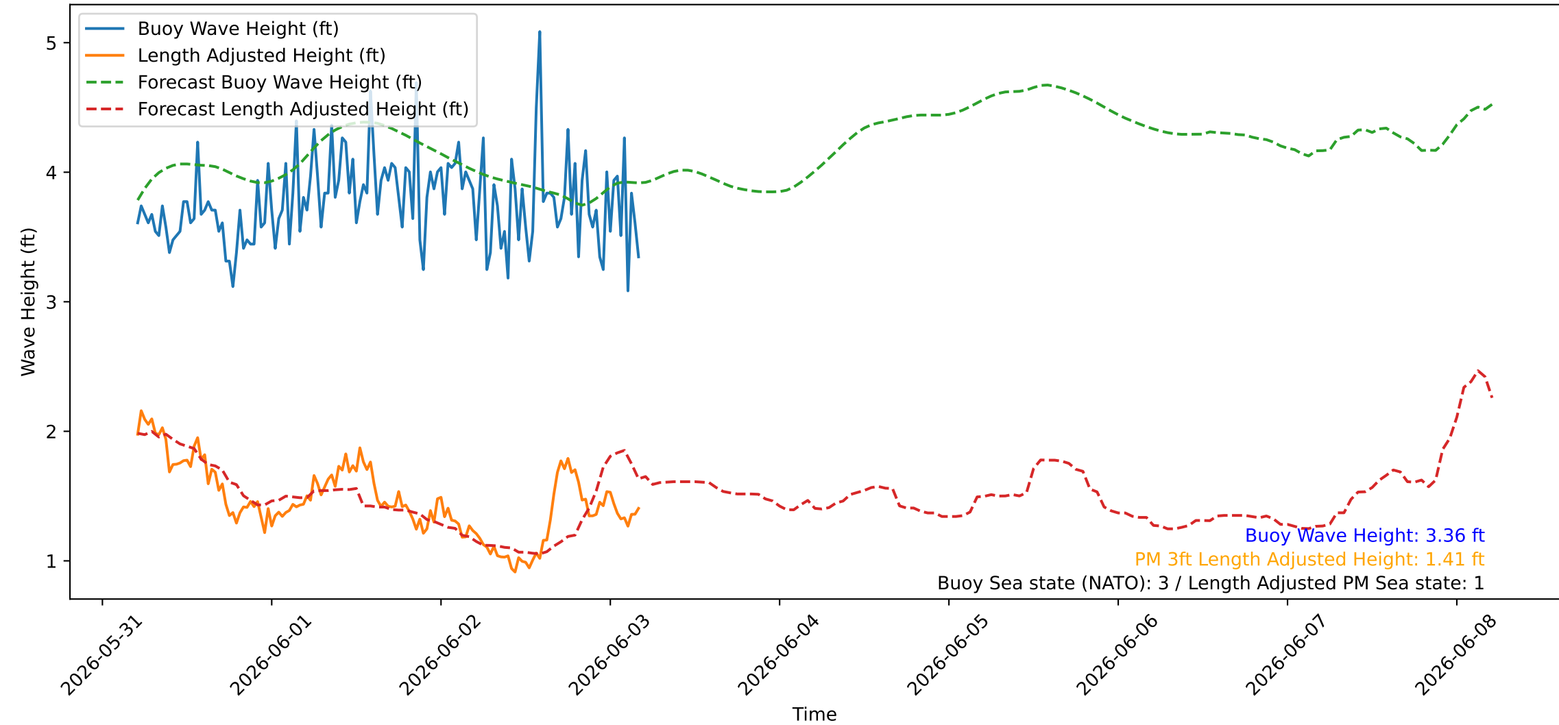
Wave Heights over Time for Oceanside Harbor at 2026-06-03 04:50:26
