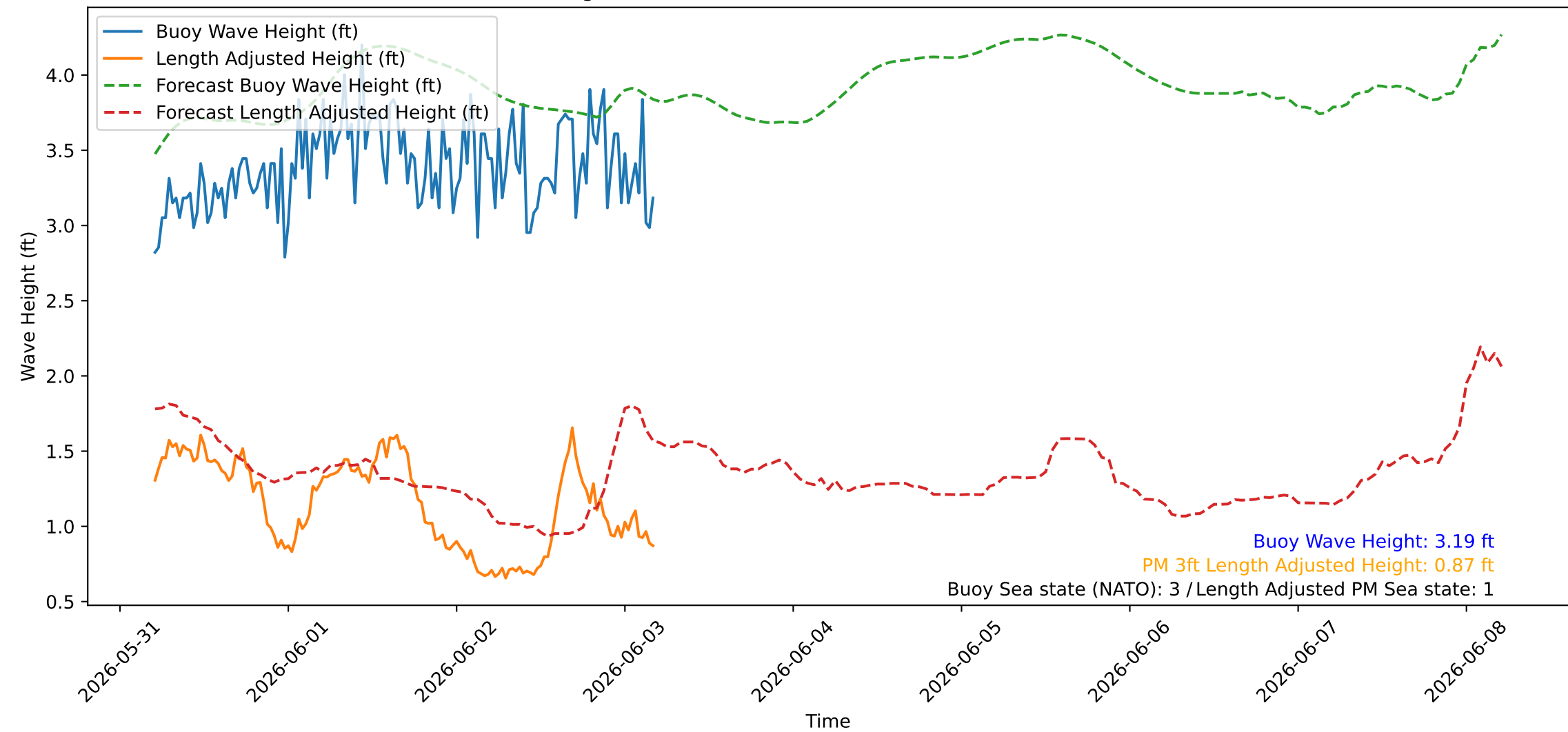
Wave Heights over Time for Red Beach at 2026-06-03 04:50:46
