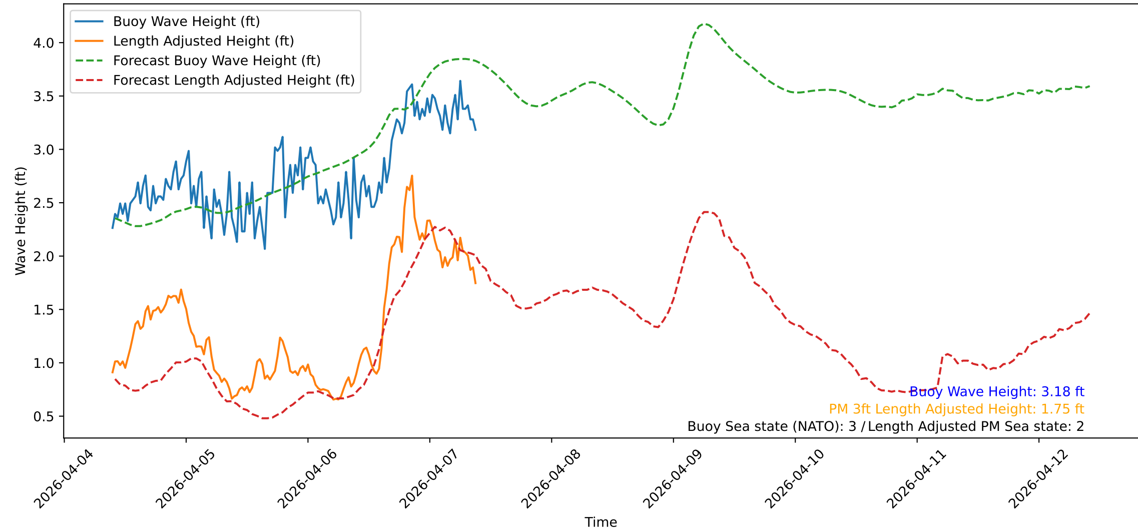
Wave Heights over Time for Oceanside Harbor at 2026-04-07 09:40:32
