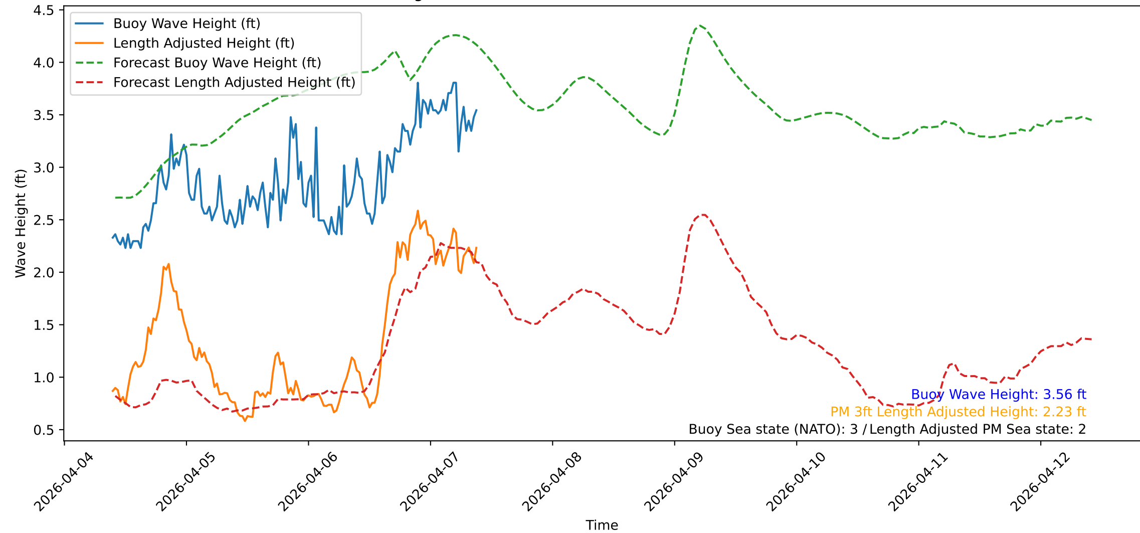
Wave Heights over Time for Green Beach at 2026-04-07 09:41:13
