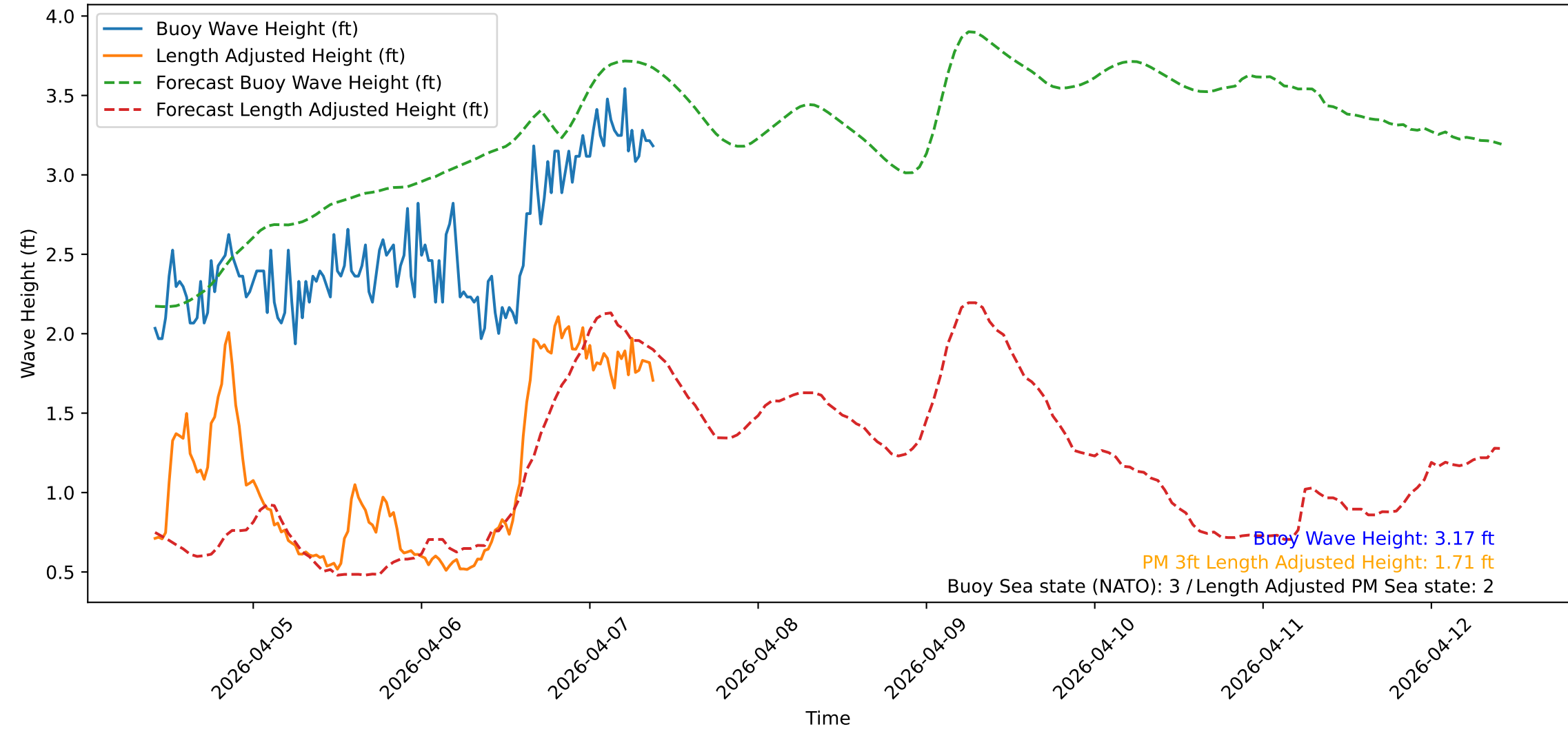
Wave Heights over Time for Red Beach at 2026-04-07 09:40:49
