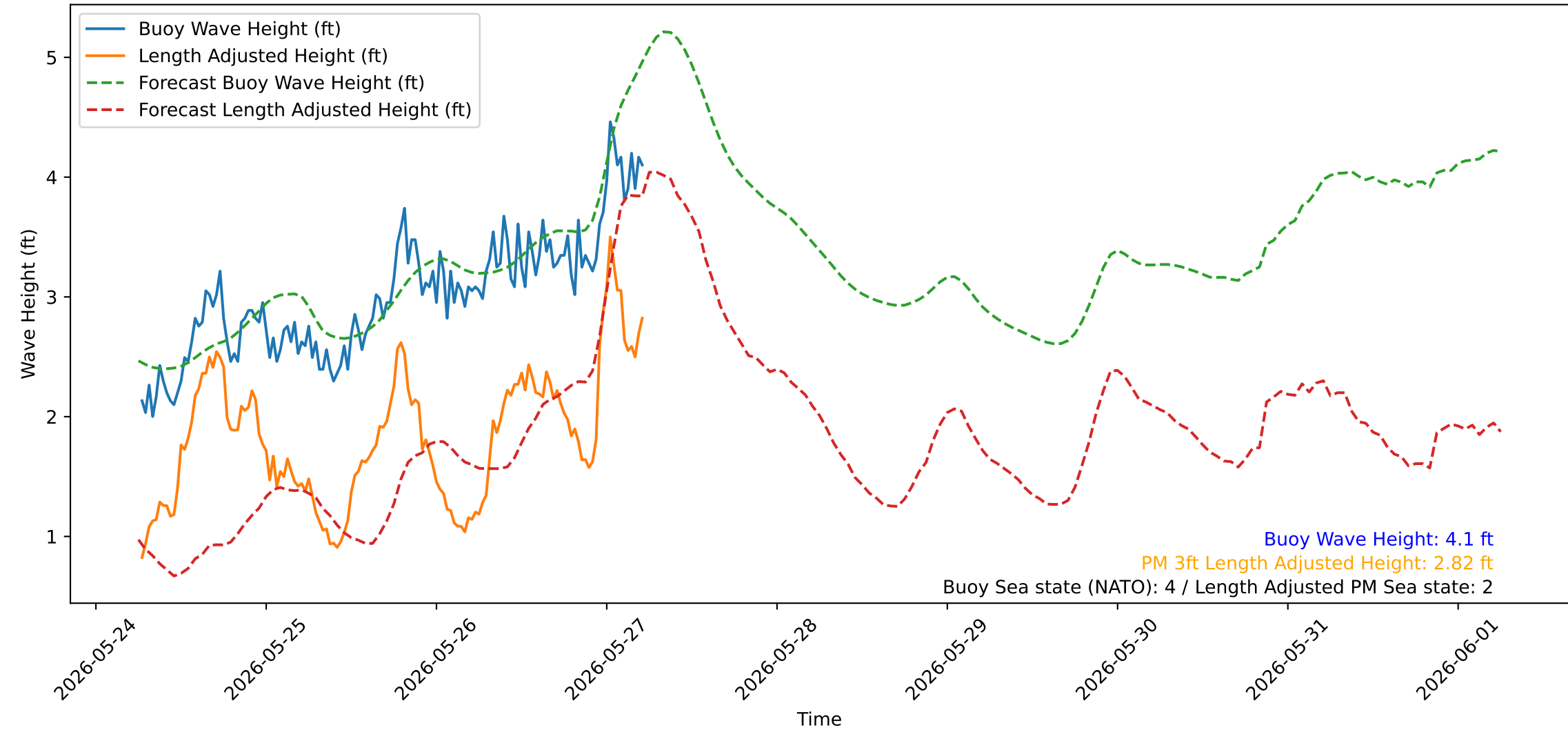
Wave Heights over Time for Red Beach at 2026-05-27 06:10:46
