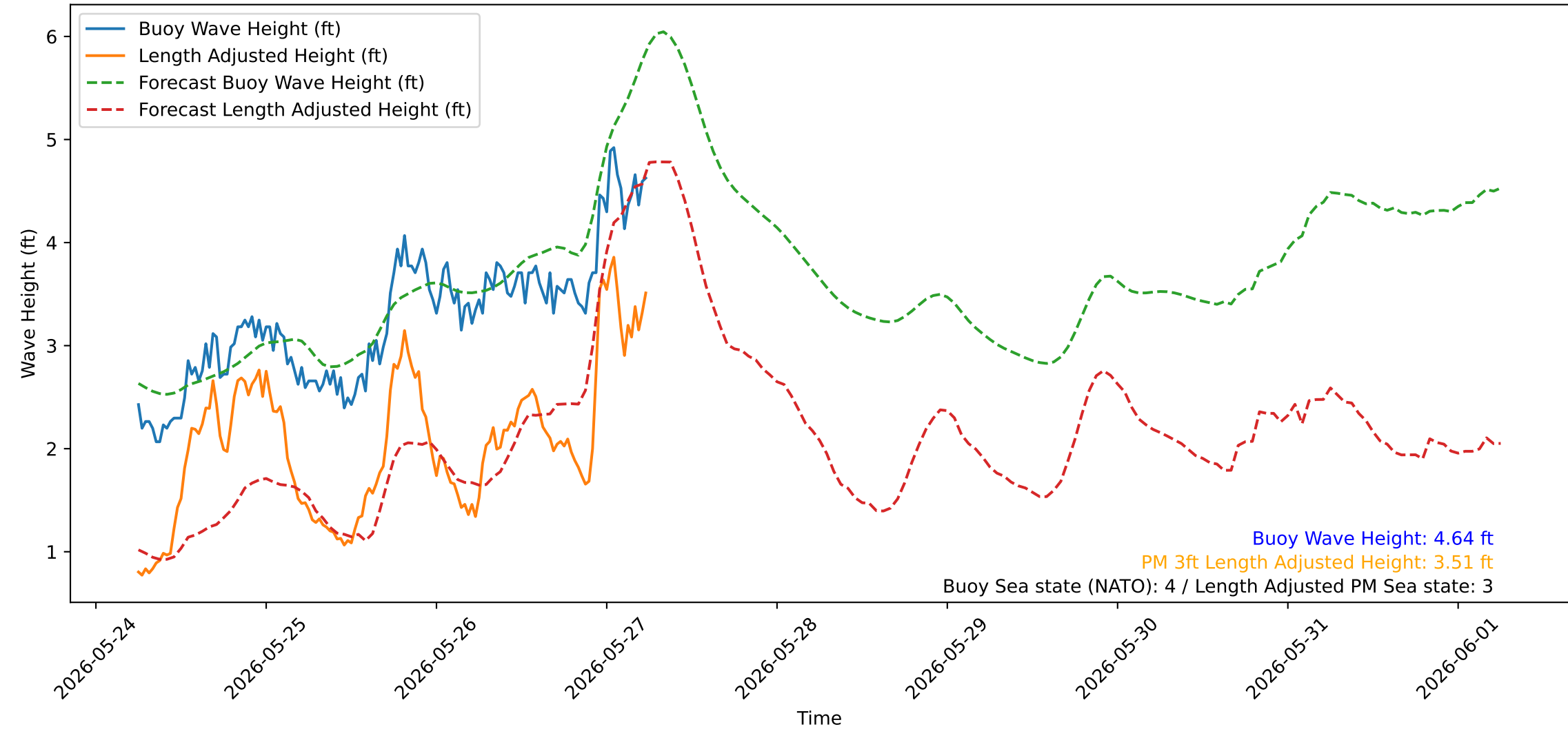
Wave Heights over Time for Green Beach at 2026-05-27 06:11:09
